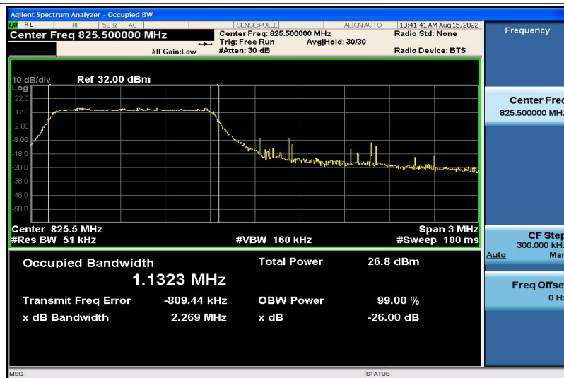
Band5-3MHz-QPSK-20415-6RB#0-1.1323
