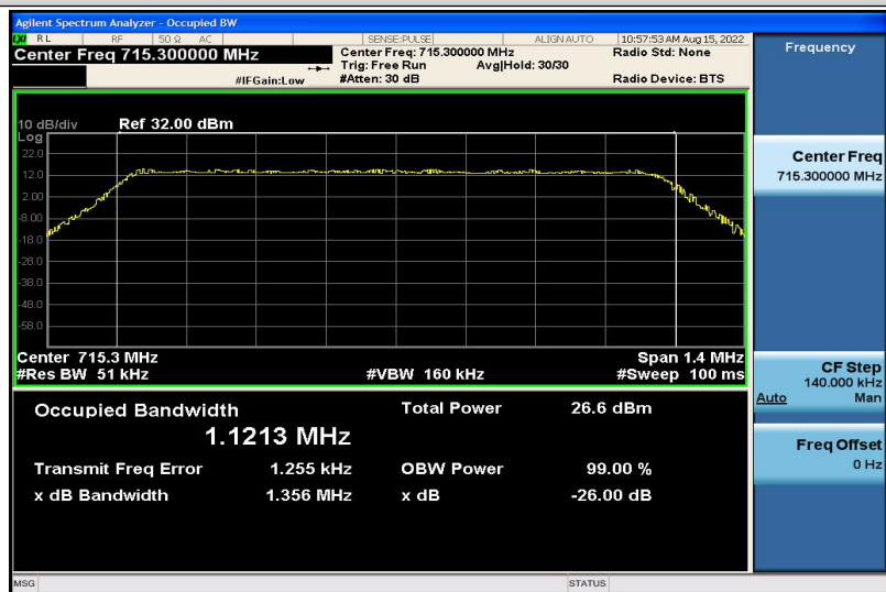
Band12-1.4MHz-QPSK-23173-6RB#0-1.1213
