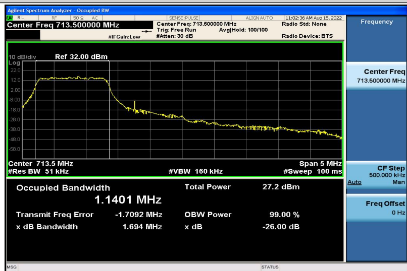
Band12-5MHz-16QAM-23155-6RB#0-1.1401
