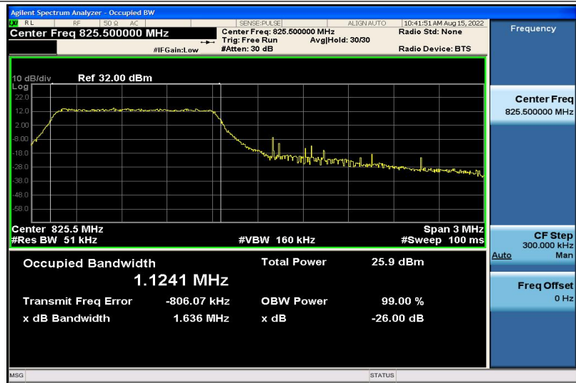
Band5-3MHz-16QAM-20415-6RB#0-1.1241
