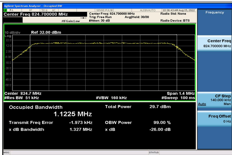
Band5-1.4MHz-QPSK-20407-6RB#0-1.1225
