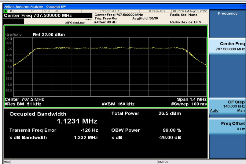
Band12-1.4MHz-QPSK-23095-6RB#0-1.1231
