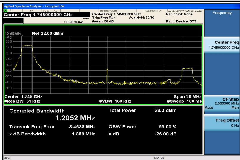
Band4-20MHz-16QAM-20300-6RB#0-1.2052
