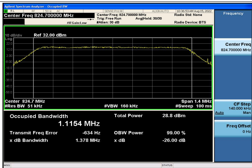
Band5-1.4MHz-16QAM-20407-6RB#0-1.1154
