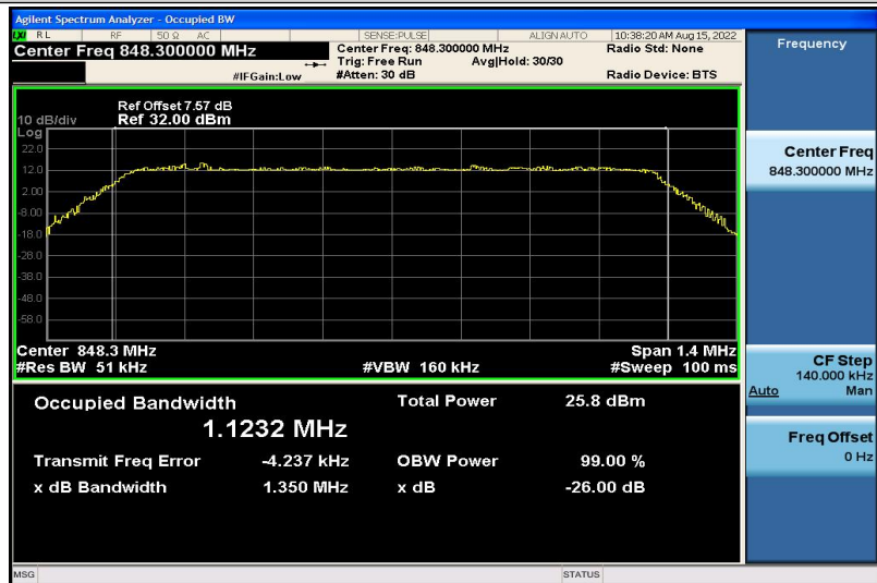
Band5-1.4MHz-16QAM-20643-6RB#0-1.1232
