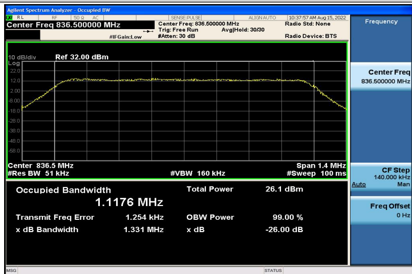
Band5-1.4MHz-16QAM-20525-6RB#0-1.1176
