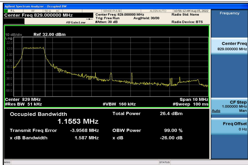
Band5-10MHz-16QAM-20450-6RB#0-1.1553
