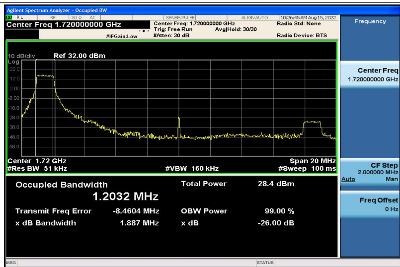
Band4-20MHz-16QAM-20050-6RB#0-1.2032
