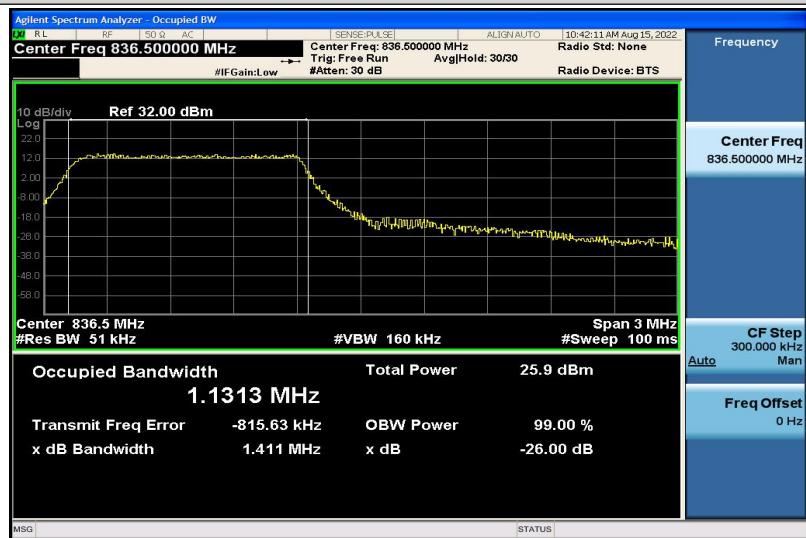
Band5-3MHz-16QAM-20525-6RB#0-1.1313
