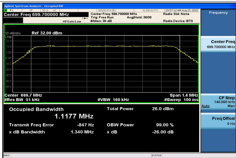
Band12-1.4MHz-QPSK-23017-6RB#0-1.1177
