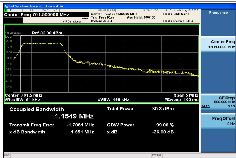
Band12-5MHz-QPSK-23035-6RB#0-1.1549
