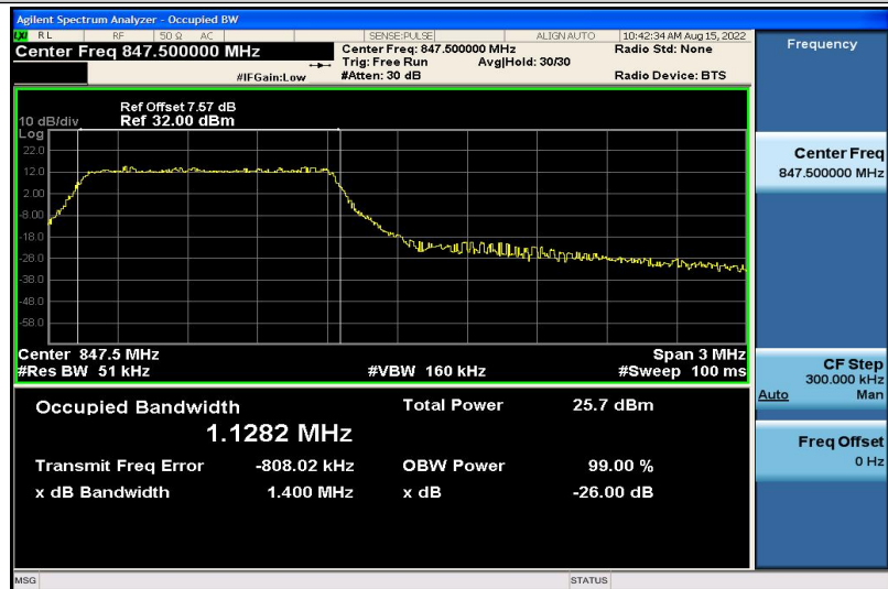
Band5-3MHz-16QAM-20635-6RB#0-1.1282
