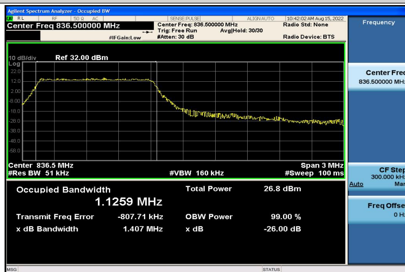
Band5-3MHz-QPSK-20525-6RB#0-1.1259
