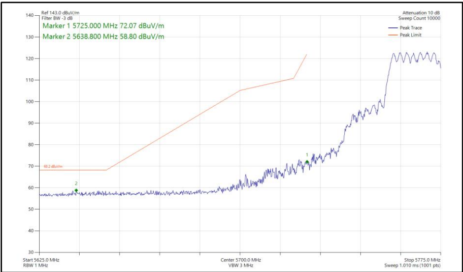
Figure 463 - 802.11ax HE20, SU, CDD, Core 0 - Core 1 - 5765 MHz Band Edge Frequency 5725 MHz
