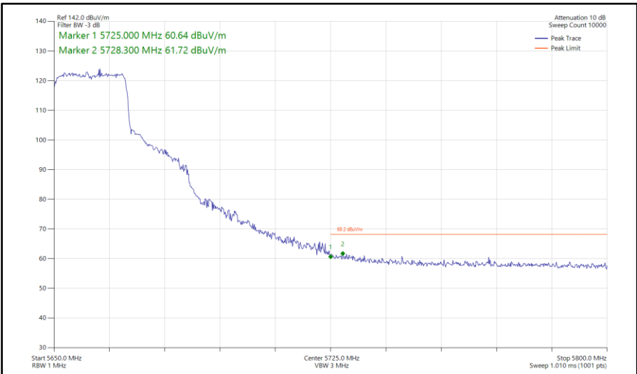
Figure 489 - 802.11ax HE20, SU, SDM, Core 0 - Core 1 - 5660 MHz Band Edge Frequency 5725 MHz
