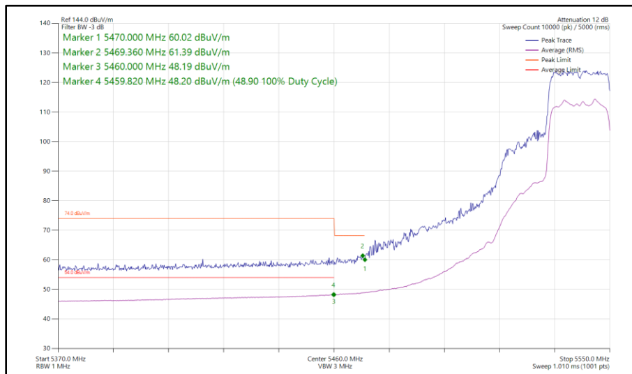
Figure 483 - 802.11ax HE20, SU, SDM, Core 0 - Core 1 - 5540 MHz Band Edge Frequency 5470 MHz
