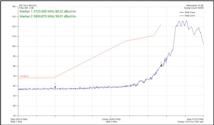
Figure 462 - 802.11ax HE20, RU 106-53, CDD, Core 0 - Core 1 - 5745 MHz Band Edge Frequency 5725 MHz
