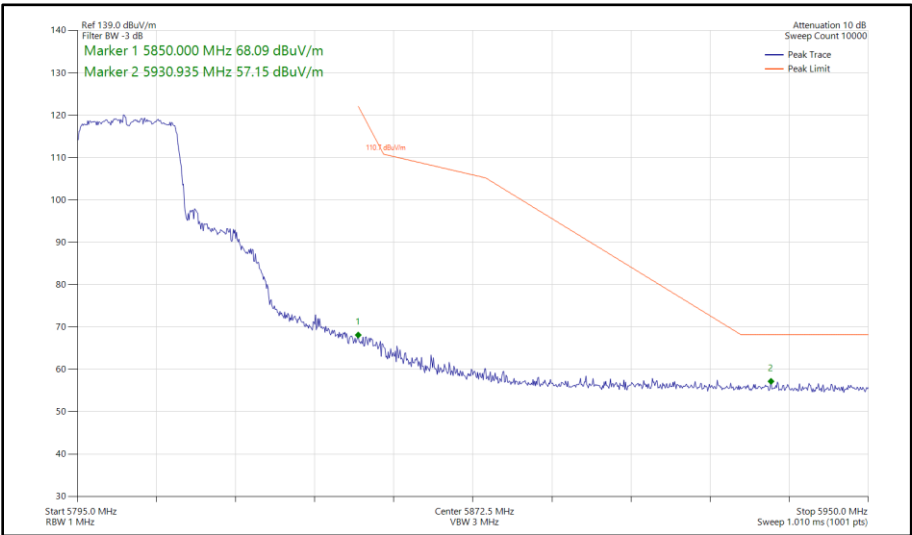
Figure 449 - 802.11ax HE20, SU, SISO, Core 1 - 5805 MHz Band Edge Frequency 5850 MHz
