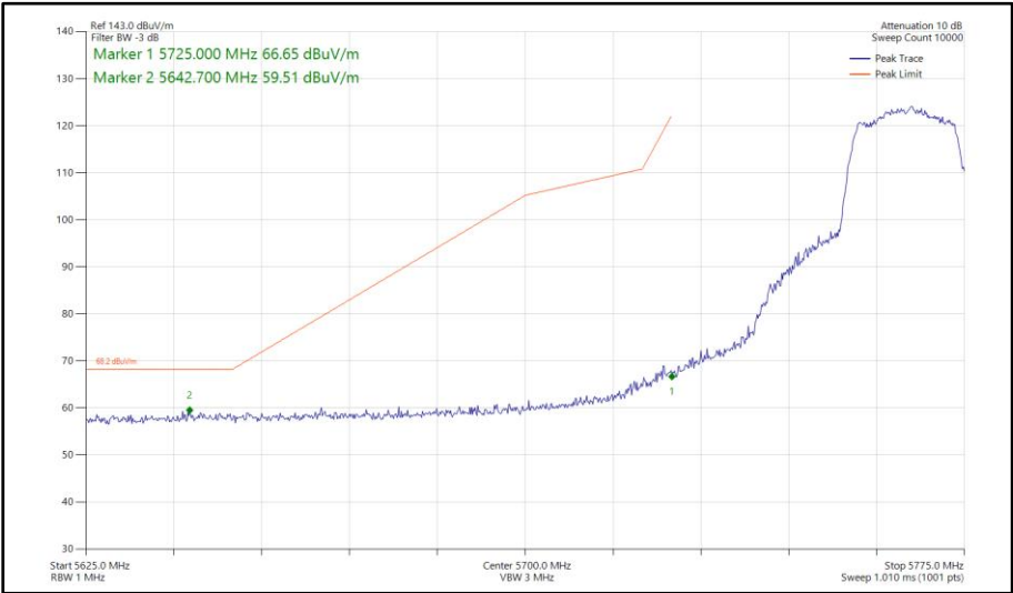
Figure 502 - 802.11ac VHT20, TxBF, Core 0 - Core 1 - 5765 MHz Band Edge Frequency 5725 MHz
