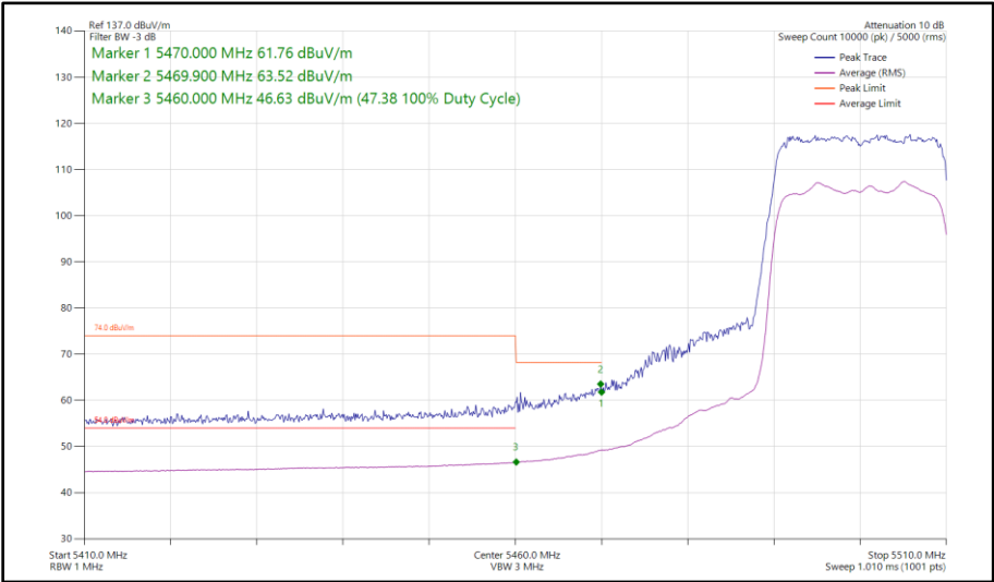
Figure 480 - 802.11ax HE20, SU, SDM, Core 0 - Core 1 - 5500 MHz Band Edge Frequency 5470 MHz
