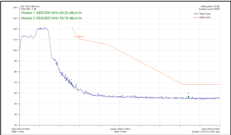
Figure 451 - 802.11ax HE20, RU 106-54, SISO, Core 1 - 5825 MHz Band Edge Frequency 5850 MHz
