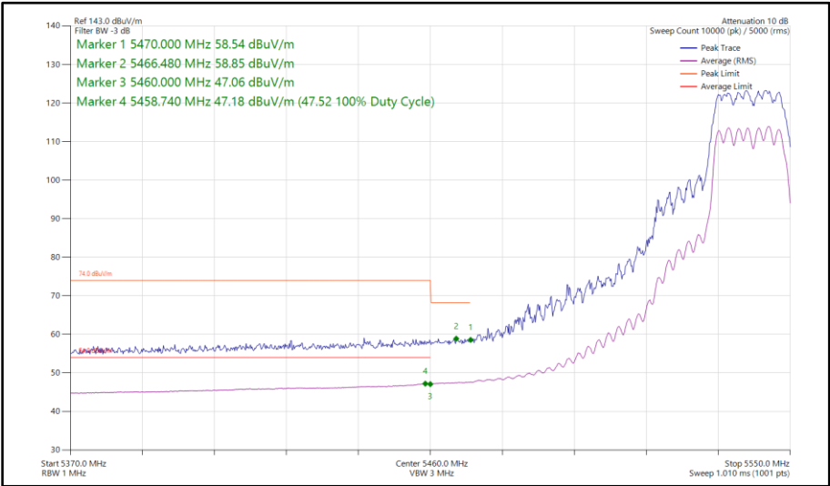
Figure 454 - 802.11n HT20, CDD, Core 0 - Core 1 - 5540 MHz Band Edge Frequency 5470 MHz
