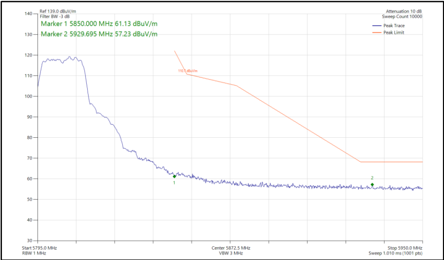
Figure 442 - 802.11a, SISO, Core 1 - 5805 MHz Band Edge Frequency 5850 MHz
