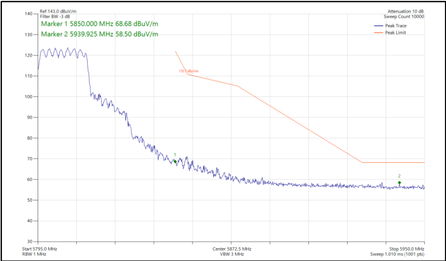
Figure 476 - 802.11ax HE20, SU, CDD, Core 0 - Core 1 - 5805 MHz Band Edge Frequency 5850 MHz
