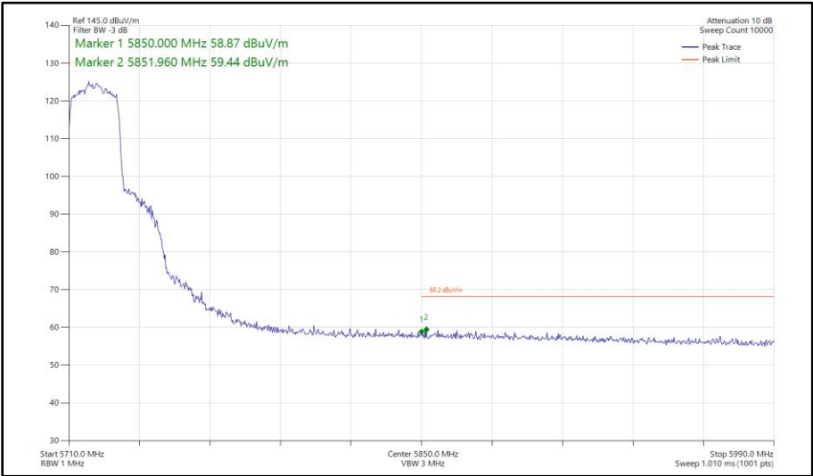
Figure 494 - 802.11ax HE20, SU, SDM, Core 0 - Core 1 - 5720 MHz Band Edge Frequency 5850 MHz
