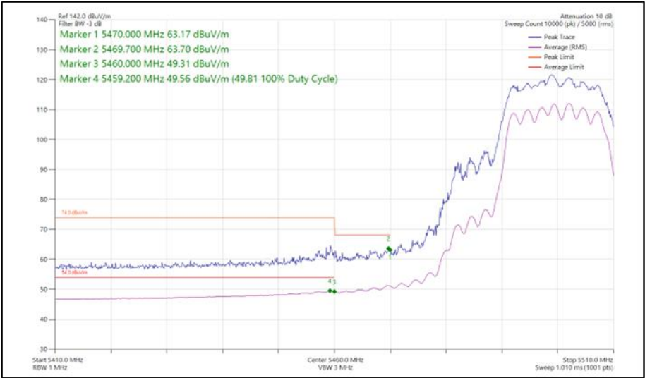
Figure 452 - 802.11n HT20, CDD, Core 0 - Core 1 - 5500 MHz Band Edge Frequency 5470 MHz
