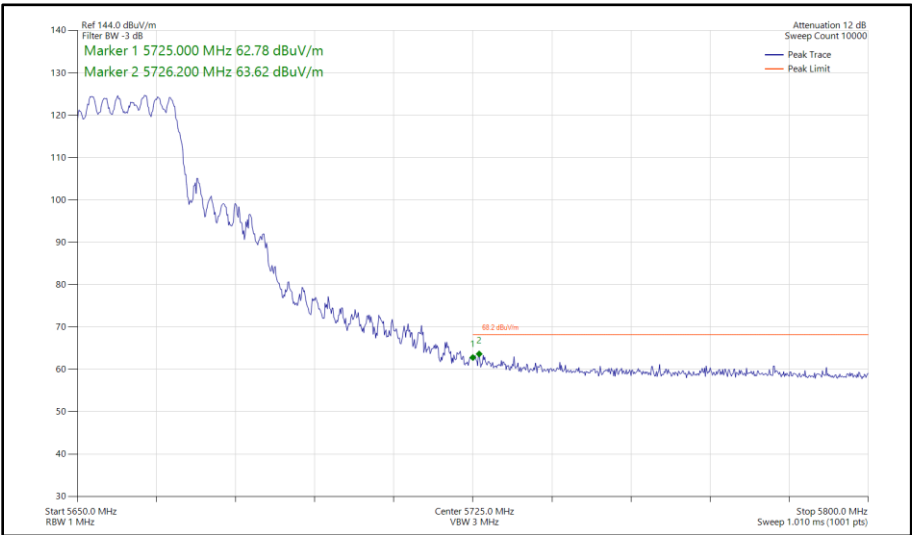
Figure 467 - 802.11ax HE20, SU, CDD, Core 0 - Core 1 - 5660 MHz Band Edge Frequency 5725 MHz
