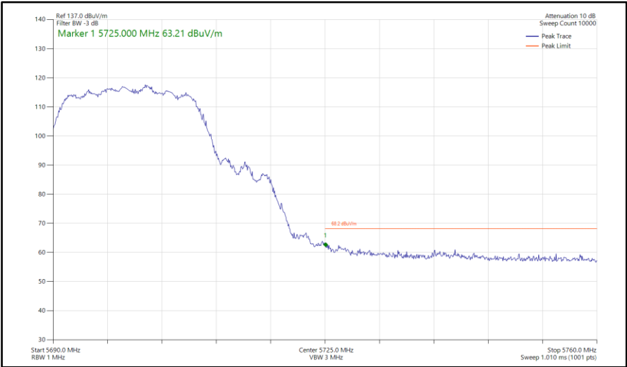
Figure 466 - 802.11n HT20, CDD, Core 0 - Core 1 - 5700 MHz Band Edge Frequency 5725 MHz
