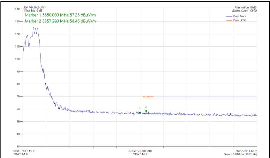
Figure 475 - 802.11ax HE20, RU 106-54, CDD, Core 0 - Core 1 - 5720 MHz Band Edge Frequency 5850 MHz
