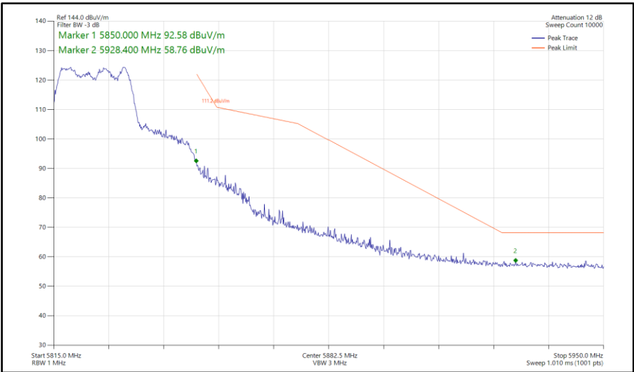
Figure 507 - 802.11ac VHT20, TxBF, Core 0 - Core 1 - 5825 MHz Band Edge Frequency 5850 MHz
