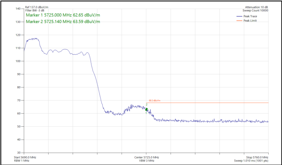
Figure 440 - 802.11ax HE20, RU 52-37, SISO, Core 1 - 5700 MHz Band Edge Frequency 5725 MHz
