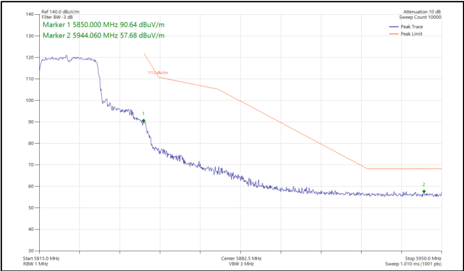
Figure 450 - 802.11ax HE20, SU, SISO, Core 1 - 5825 MHz Band Edge Frequency 5850 MHz
