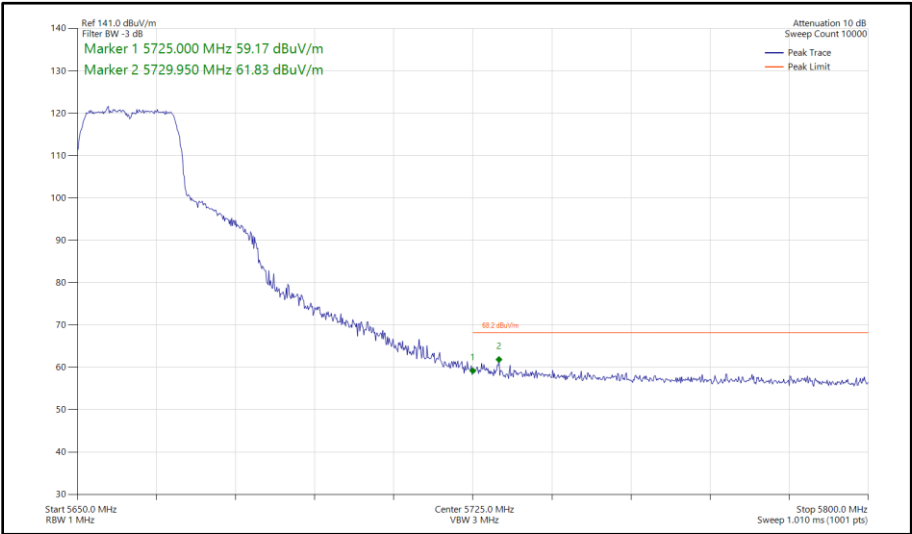
Figure 434 - 802.11n HT20, SISO, Core 1 - 5660 MHz Band Edge Frequency 5725 MHz
