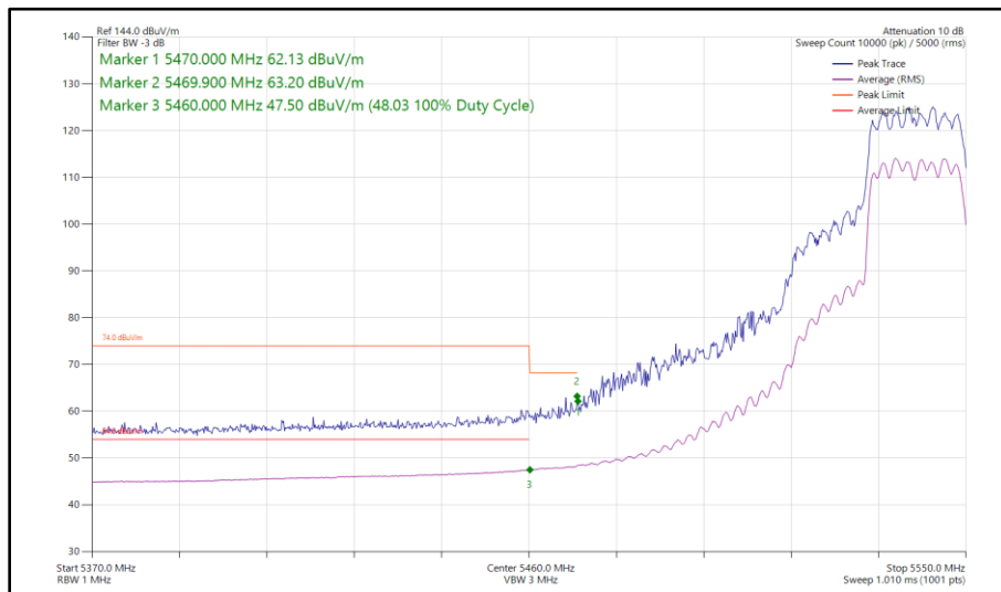
Figure 458 - 802.11ax HE20, SU, CDD, Core 0 - Core 1 - 5540 MHz Band Edge Frequency 5470 MHz
