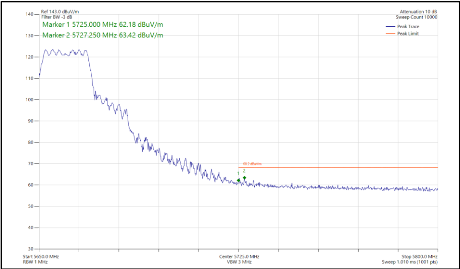
Figure 464 - 802.11n HT20, CDD, Core 0 - Core 1 - 5660 MHz Band Edge Frequency 5725 MHz
