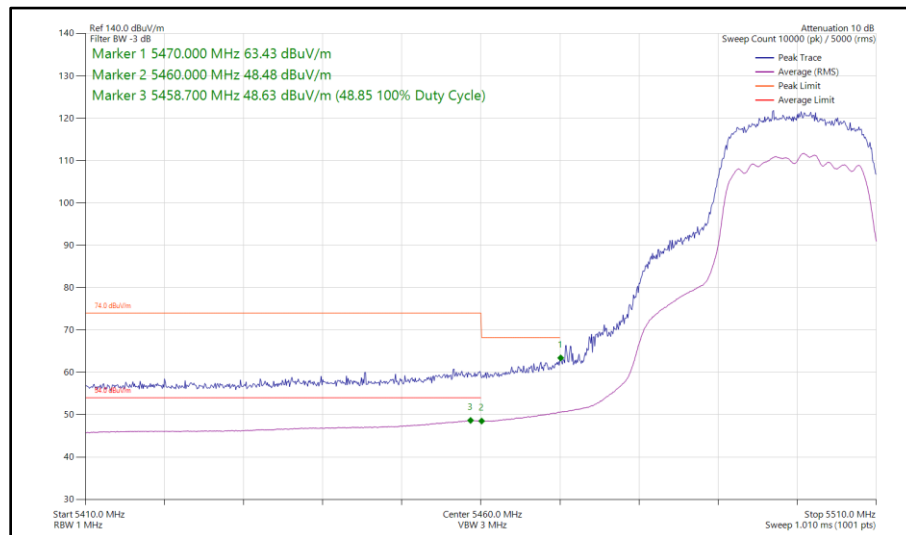
Figure 499 - 802.11ac VHT20, TxBF, Core 0 - Core 1 - 5500 MHz Band Edge Frequency 5470 MHz
