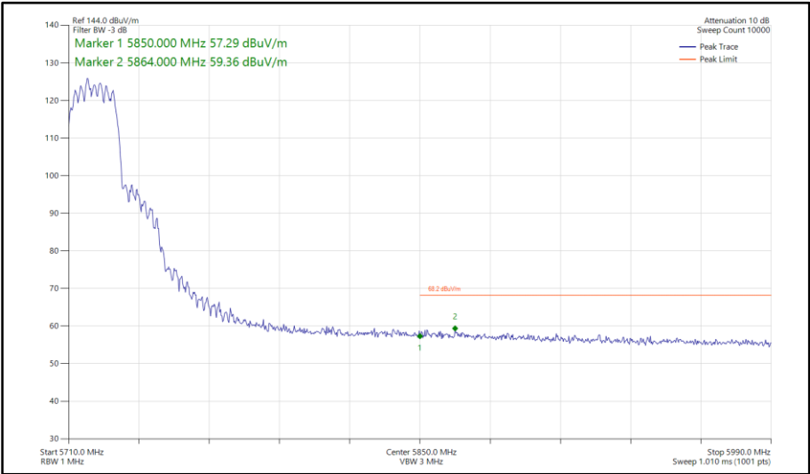
Figure 474 - 802.11ax HE20, SU, CDD, Core 0 - Core 1 - 5720 MHz Band Edge Frequency 5850 MHz
