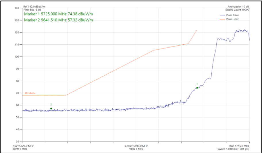
Figure 430 - 802.11ax HE20, RU 106-54, SISO, Core 1 - 5745 MHz Band Edge Frequency 5725 MHz
