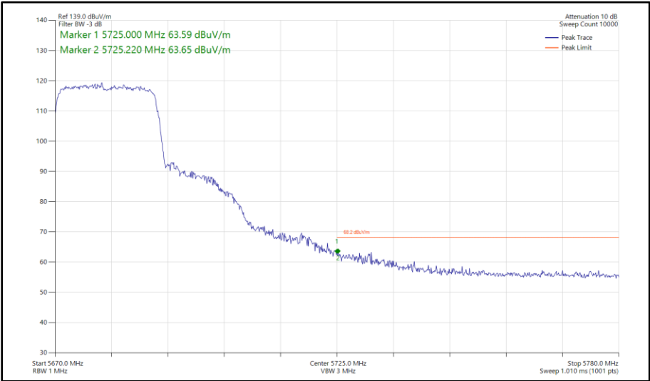
Figure 438 - 802.11ax HE20, SU, SISO, Core 1 - 5680 MHz Band Edge Frequency 5725 MHz
