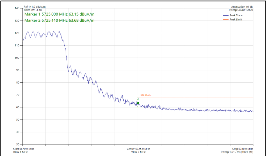
Figure 468 - 802.11ax HE20, SU, CDD, Core 0 - Core 1 - 5680 MHz Band Edge Frequency 5725 MHz
