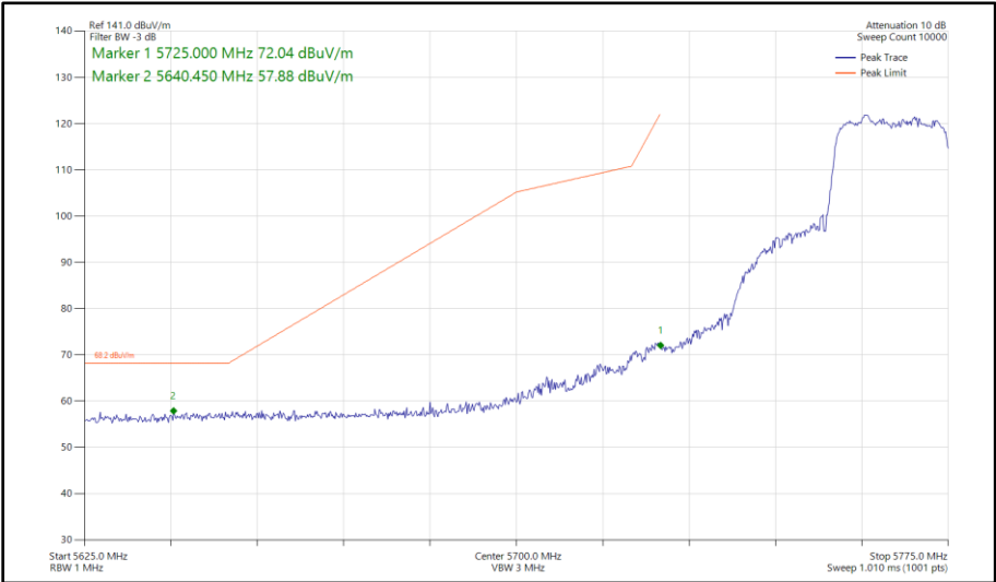
Figure 487 - 802.11ax HE20, SU, SDM, Core 0 - Core 1 - 5765 MHz Band Edge Frequency 5725 MHz
