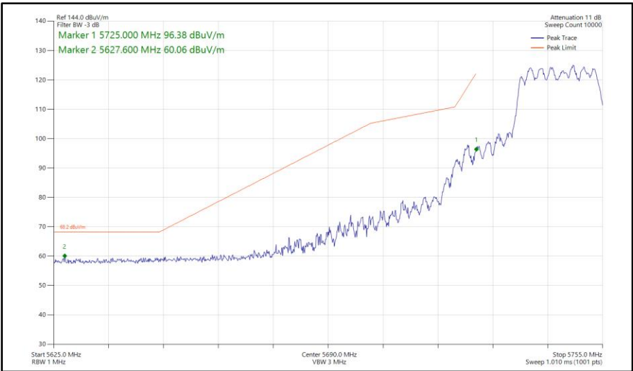
Figure 461 - 802.11ax HE20, SU, CDD, Core 0 - Core 1 - 5745 MHz Band Edge Frequency 5725 MHz
