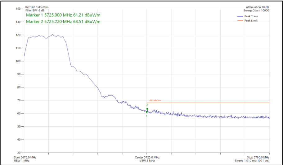
Figure 432 - 802.11a, SISO, Core 1 - 5680 MHz Band Edge Frequency 5725 MHz
