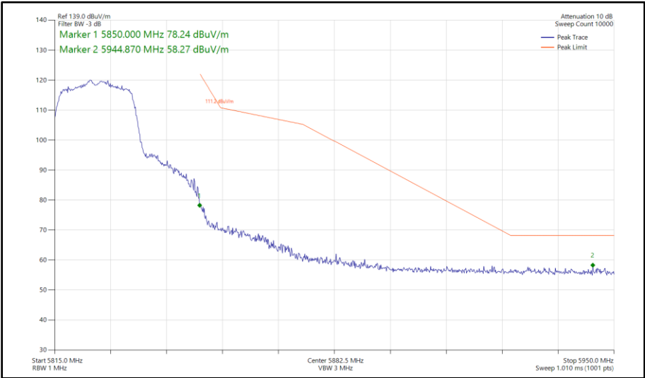
Figure 446 - 802.11n HT20, SISO, Core 1 - 5825 MHz Band Edge Frequency 5850 MHz
