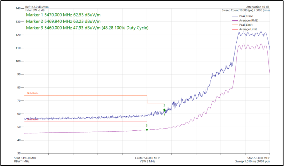
Figure 453 - 802.11n HT20, CDD, Core 0 - Core 1 - 5520 MHz Band Edge Frequency 5470 MHz
