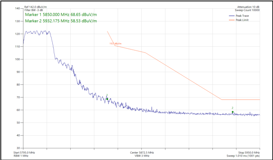
Figure 472 - 802.11n HT20, CDD, Core 0 - Core 1 - 5805 MHz Band Edge Frequency 5850 MHz
