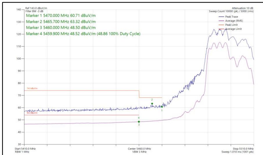
Figure 456 - 802.11ax HE20, RU 106-53, CDD, Core 0 - Core 1 - 5500 MHz Band Edge Frequency 5470 MHz
