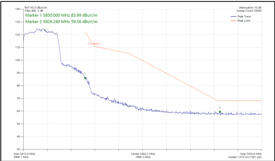
Figure 497 - 802.11ax HE20, SU, SDM, Core 0 - Core 1 - 5825 MHz Band Edge Frequency 5850 MHz
