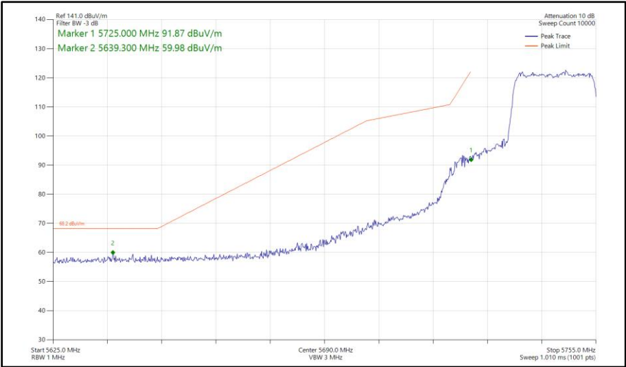
Figure 485 - 802.11ax HE20, SU, SDM, Core 0 - Core 1 - 5745 MHz Band Edge Frequency 5725 MHz
