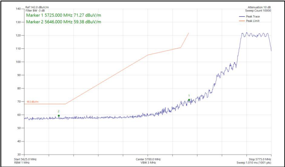
Figure 460 - 802.11n HT20, CDD, Core 0 - Core 1 - 5765 MHz Band Edge Frequency 5725 MHz
