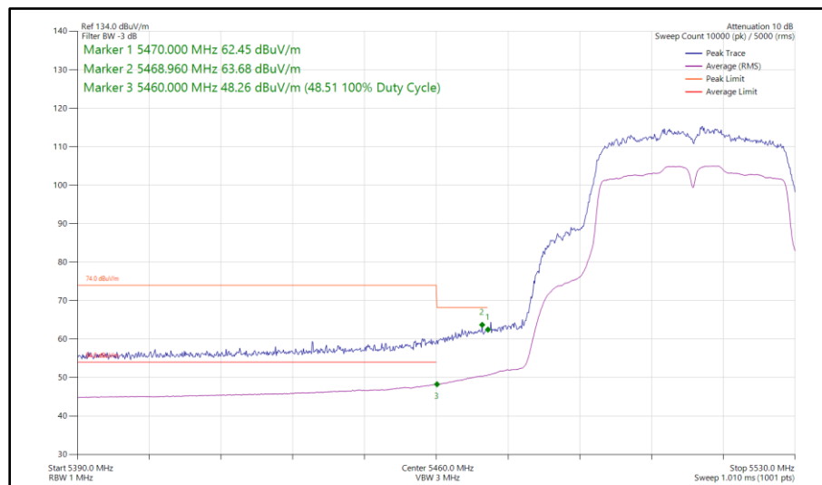
Figure 508 - 802.11n HT40, SISO, Core 0 - 5510 MHz Band Edge Frequency 5470 MHz
