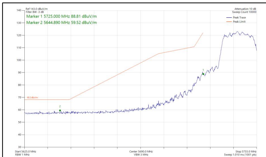
Figure 459 - 802.11n HT20, CDD, Core 0 - Core 1 - 5745 MHz Band Edge Frequency 5725 MHz
