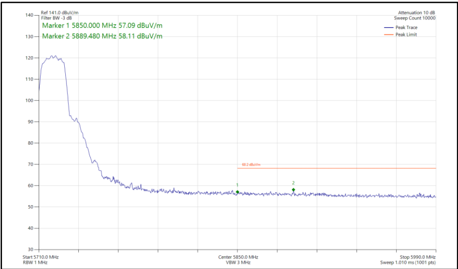
Figure 441 - 802.11a, SISO, Core 1 - 5720 MHz Band Edge Frequency 5850 MHz
