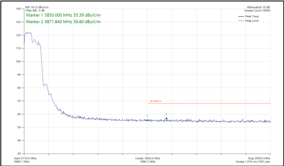
Figure 448 - 802.11ax HE20, RU 106-53, SISO, Core 1 - 5720 MHz Band Edge Frequency 5850 MHz
