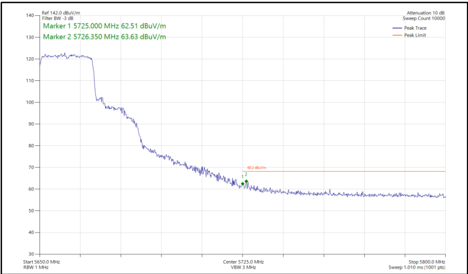
Figure 437 - 802.11ax HE20, SU, SISO, Core 1 - 5660 MHz Band Edge Frequency 5725 MHz
