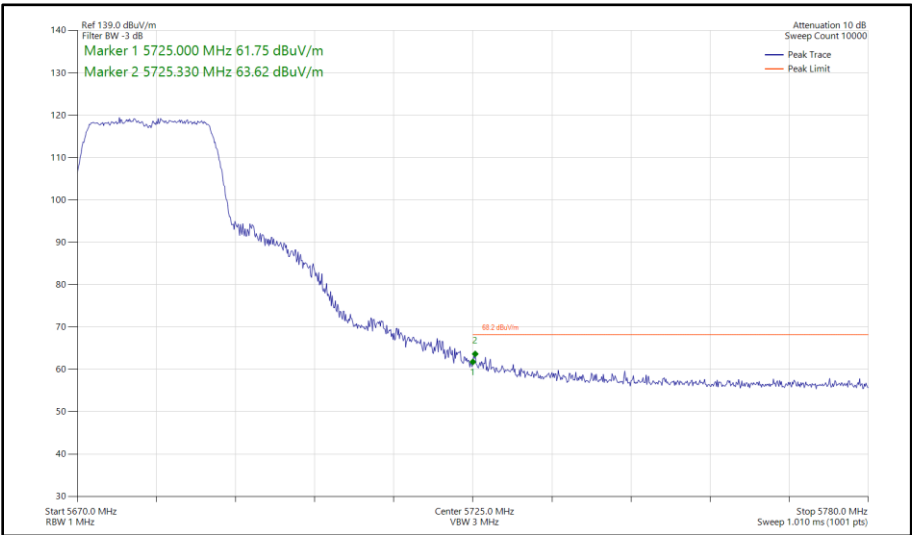
Figure 435 - 802.11n HT20, SISO, Core 1 - 5680 MHz Band Edge Frequency 5725 MHz
