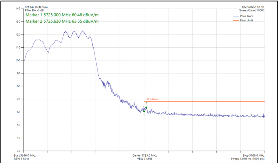
Figure 492 - 802.11ax HE20, RU 106-54, SDM, Core 0 - Core 1 - 5700 MHz Band Edge Frequency 5725 MHz
