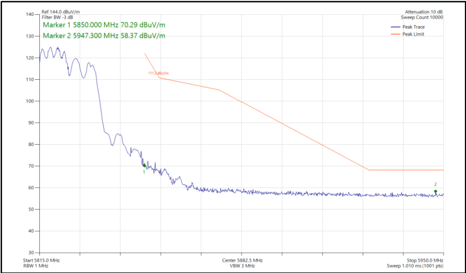
Figure 478 - 802.11ax HE20, RU 106-53, CDD, Core 0 - Core 1 - 5825 MHz Band Edge Frequency 5850 MHz
