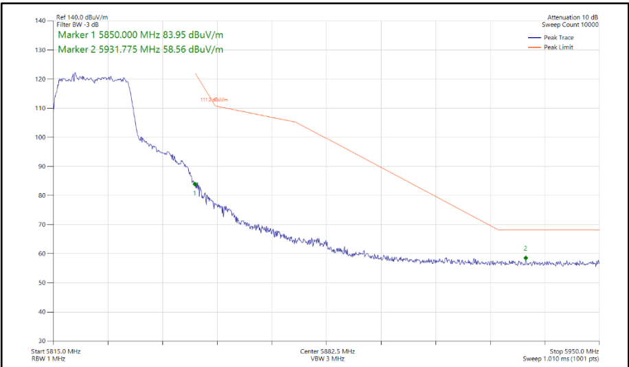
Figure 493 - 802.11n HT20, SDM, Core 0 - Core 1 - 5825 MHz Band Edge Frequency 5850 MHz
