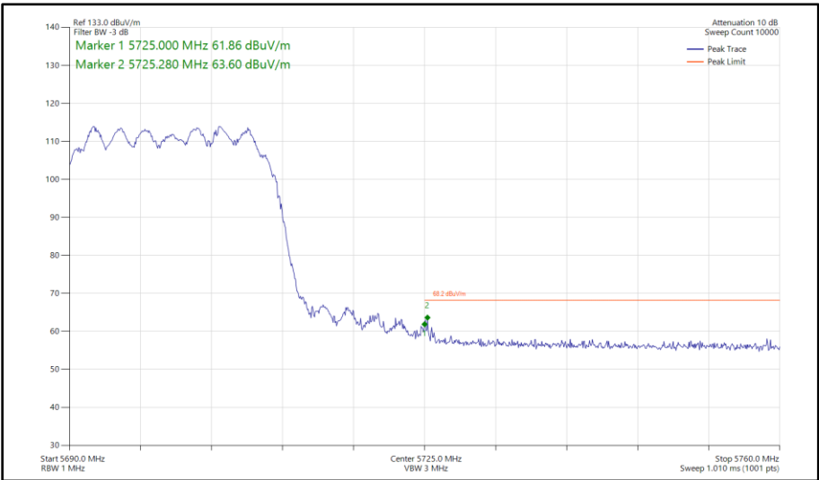
Figure 469 - 802.11ax HE20, SU, CDD, Core 0 - Core 1 - 5700 MHz Band Edge Frequency 5725 MHz
