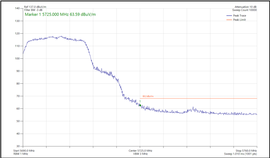
Figure 504 - 802.11ac VHT20, TxBF, Core 0 - Core 1 - 5700 MHz Band Edge Frequency 5725 MHz
