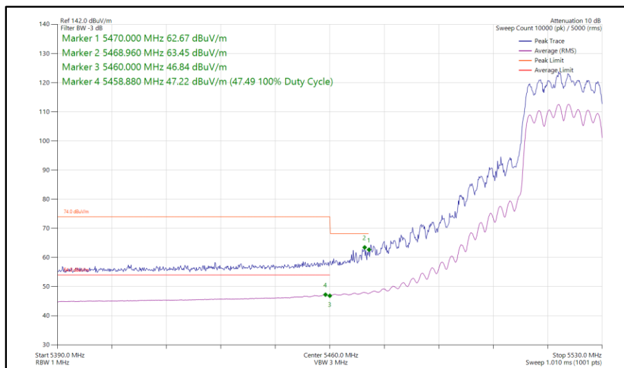
Figure 457 - 802.11ax HE20, SU, CDD, Core 0 - Core 1 - 5520 MHz Band Edge Frequency 5470 MHz
