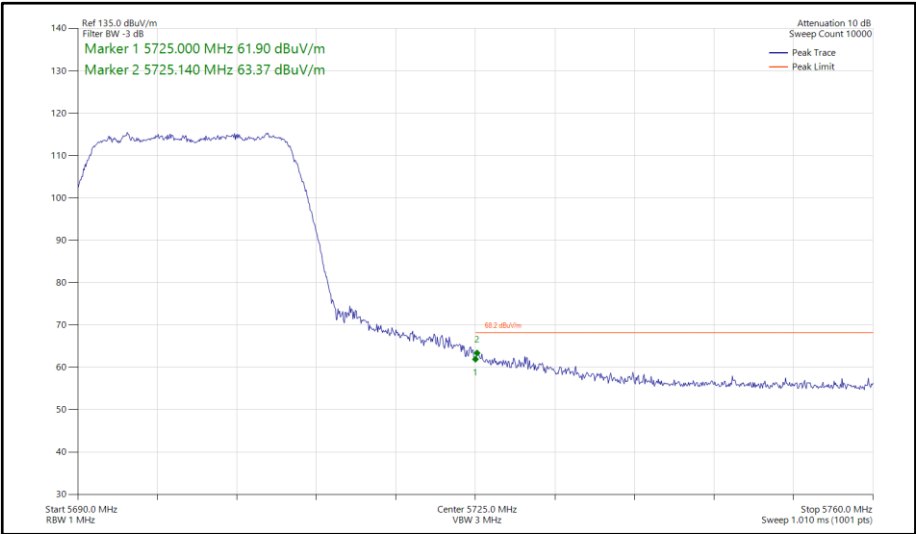
Figure 488 - 802.11n HT20, SDM, Core 0 - Core 1 - 5700 MHz Band Edge Frequency 5725 MHz
