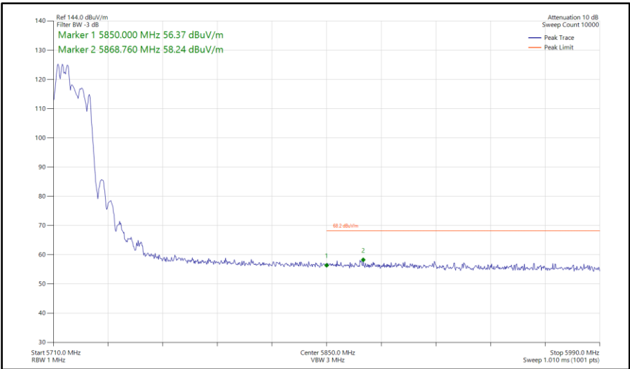
Figure 495 - 802.11ax HE20, RU 106-53, SDM, Core 0 - Core 1 - 5720 MHz Band Edge Frequency 5850 MHz
