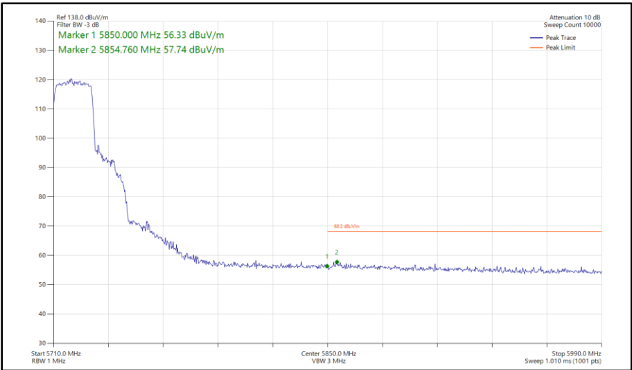
Figure 447 - 802.11ax HE20, SU, SISO, Core 1 - 5720 MHz Band Edge Frequency 5850 MHz
