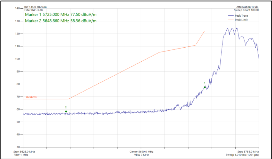
Figure 486 - 802.11ax HE20, RU 106-53, SDM, Core 0 - Core 1 - 5745 MHz Band Edge Frequency 5725 MHz
