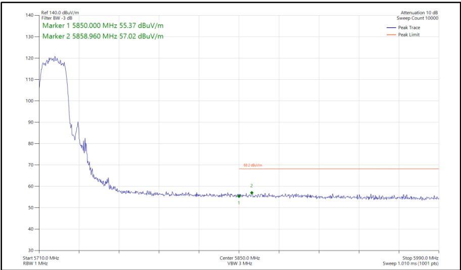
Figure 505 - 802.11ac VHT20, TxBF, Core 0 - Core 1 - 5720 MHz Band Edge Frequency 5850 MHz
