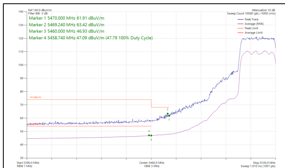
Figure 482 - 802.11ax HE20, SU, SDM, Core 0 - Core 1 - 5520 MHz Band Edge Frequency 5470 MHz
