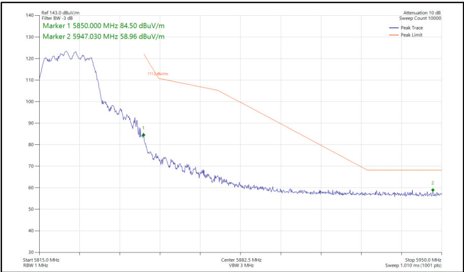
Figure 473 - 802.11n HT20, CDD, Core 0 - Core 1 - 5825 MHz Band Edge Frequency 5850 MHz
