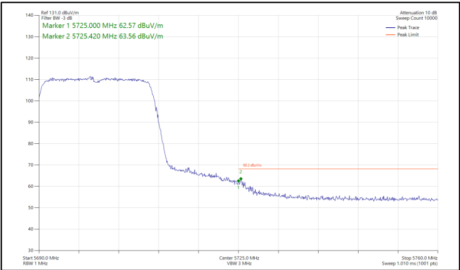
Figure 439 - 802.11ax HE20, SU, SISO, Core 1 - 5700 MHz Band Edge Frequency 5725 MHz
