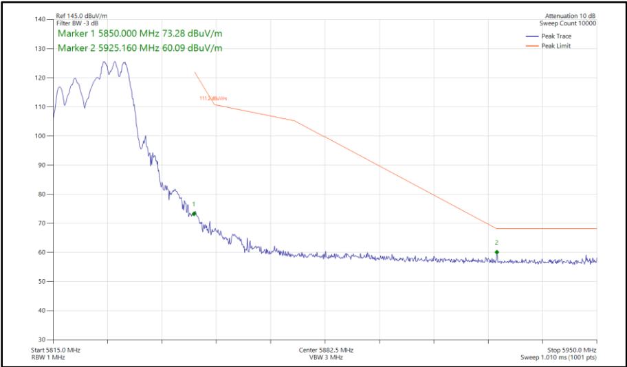
Figure 498 - 802.11ax HE20, RU 106-54, SDM, Core 0 - Core 1 - 5825 MHz Band Edge Frequency 5850 MHz
