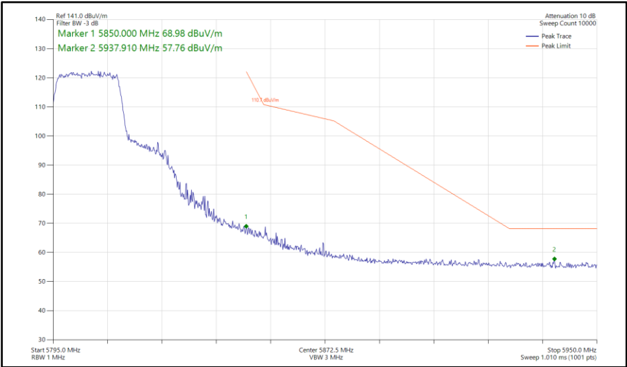
Figure 506 - 802.11ac VHT20, TxBF, Core 0 - Core 1 - 5805 MHz Band Edge Frequency 5850 MHz
