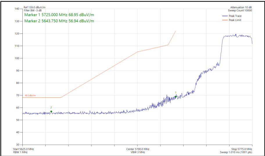
Figure 431 - 802.11ax HE20, SU, SISO, Core 1 - 5765 MHz Band Edge Frequency 5725 MHz
