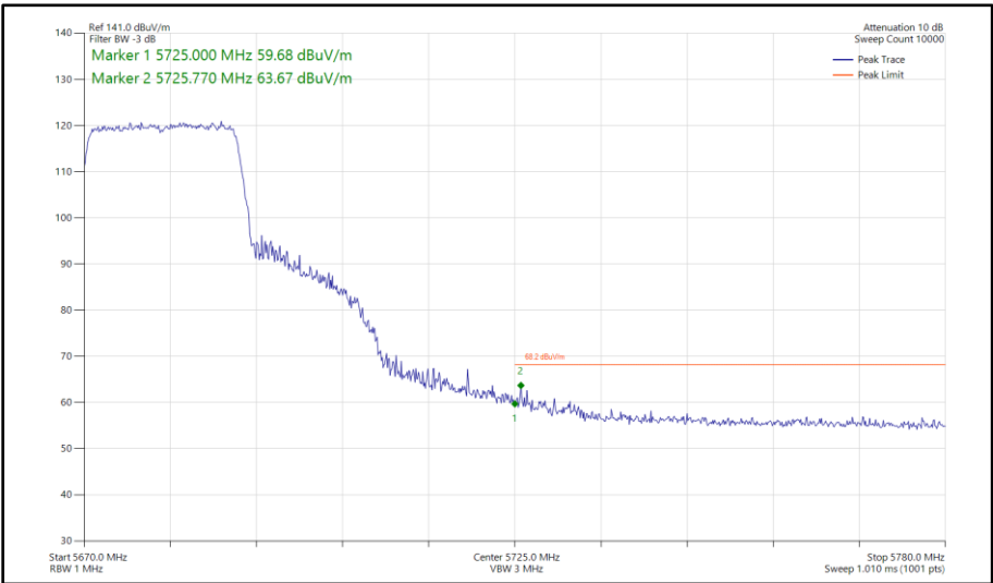
Figure 503 - 802.11ac VHT20, TxBF, Core 0 - Core 1 - 5680 MHz Band Edge Frequency 5725 MHz
