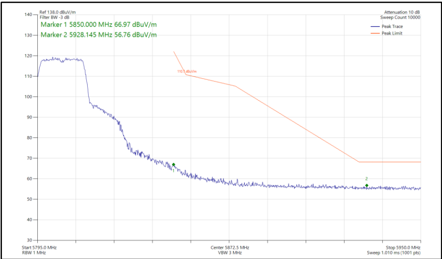
Figure 445 - 802.11n HT20, SISO, Core 1 - 5805 MHz Band Edge Frequency 5850 MHz
