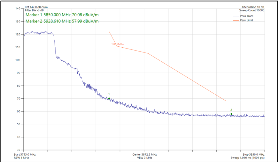
Figure 496 - 802.11ax HE20, SU, SDM, Core 0 - Core 1 - 5805 MHz Band Edge Frequency 5850 MHz
