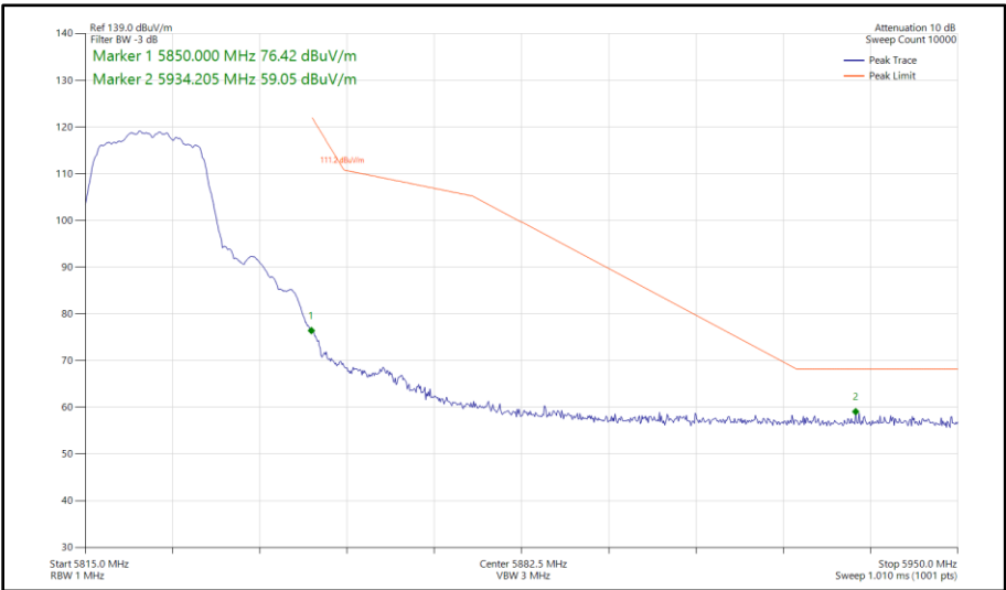
Figure 443 - 802.11a, SISO, Core 1 - 5825 MHz Band Edge Frequency 5850 MHz
