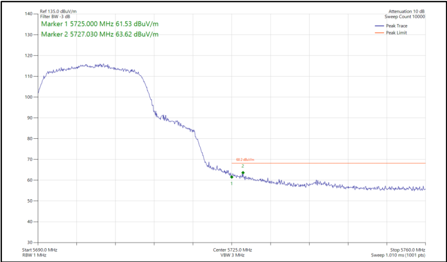
Figure 436 - 802.11n HT20, SISO, Core 1 - 5700 MHz Band Edge Frequency 5725 MHz
