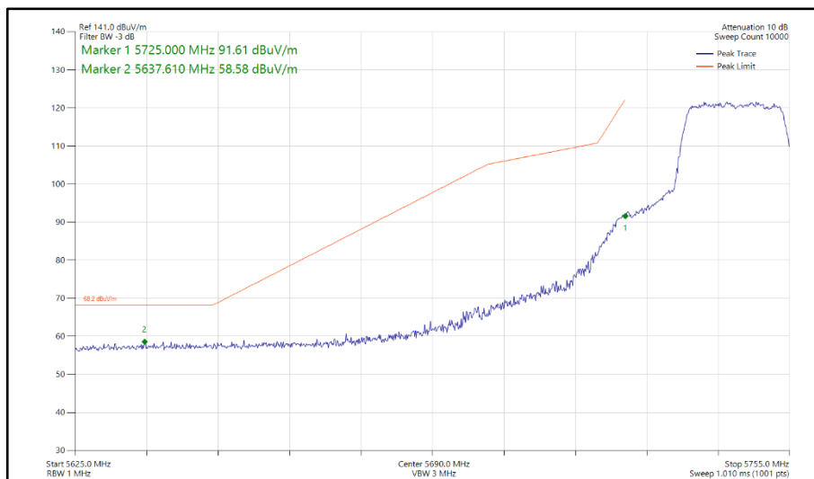
Figure 484 - 802.11n HT20, SDM, Core 0 - Core 1 - 5745 MHz Band Edge Frequency 5725 MHz
