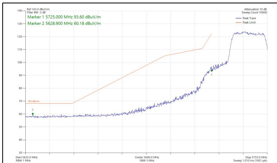
Figure 501 - 802.11ac VHT20, TxBF, Core 0 - Core 1 - 5745 MHz Band Edge Frequency 5725 MHz
