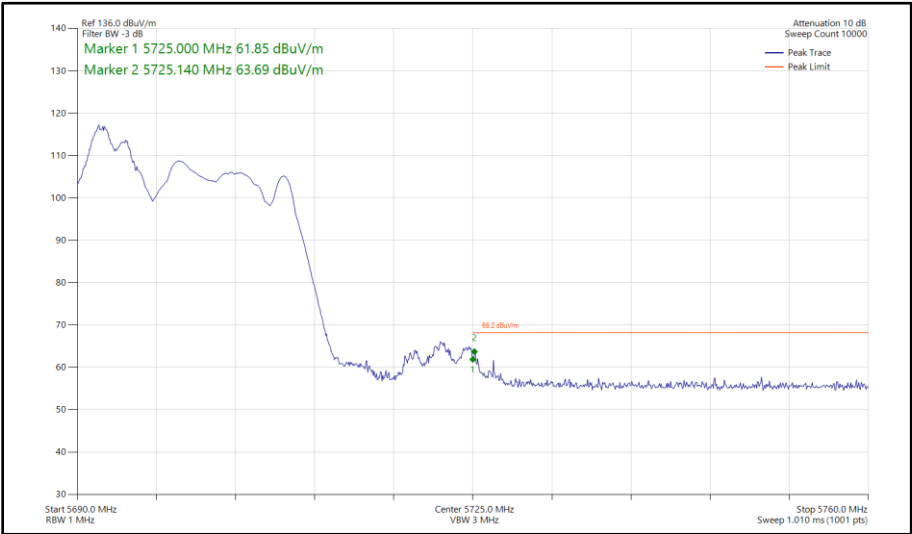
Figure 470 - 802.11ax HE20, RU 52-37, CDD, Core 0 - Core 1 - 5700 MHz Band Edge Frequency 5725 MHz
