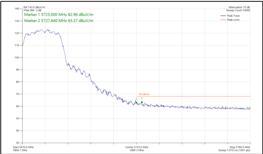
Figure 465 - 802.11n HT20, CDD, Core 0 - Core 1 - 5680 MHz Band Edge Frequency 5725 MHz
