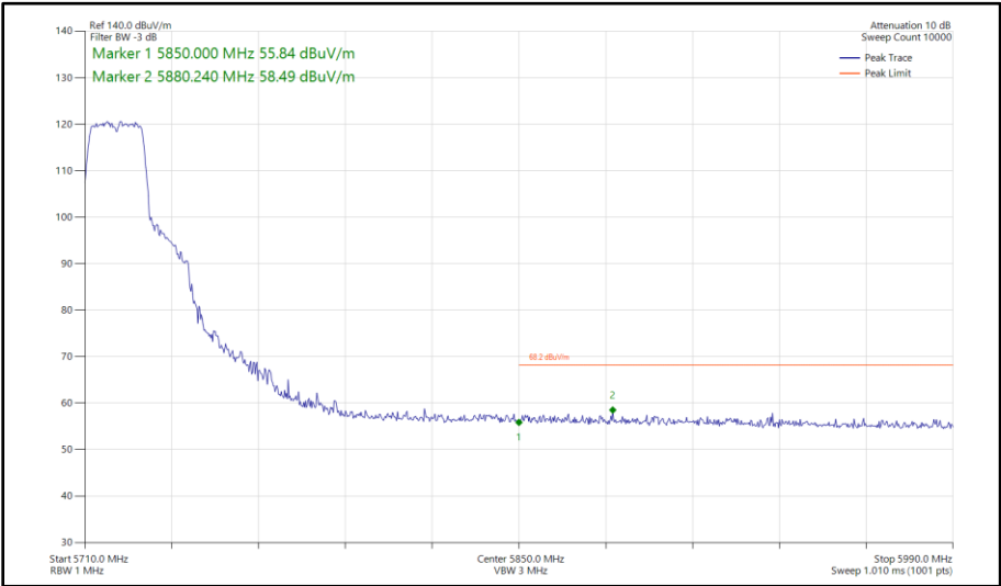
Figure 444 - 802.11n HT20, SISO, Core 1 - 5720 MHz Band Edge Frequency 5850 MHz
