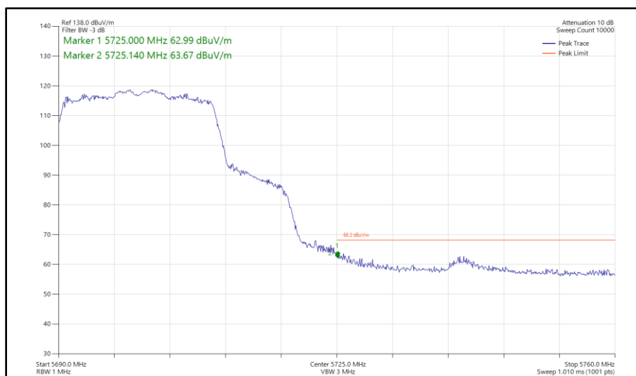
Figure 491 - 802.11ax HE20, SU, SDM, Core 0 - Core 1 - 5700 MHz Band Edge Frequency 5725 MHz
