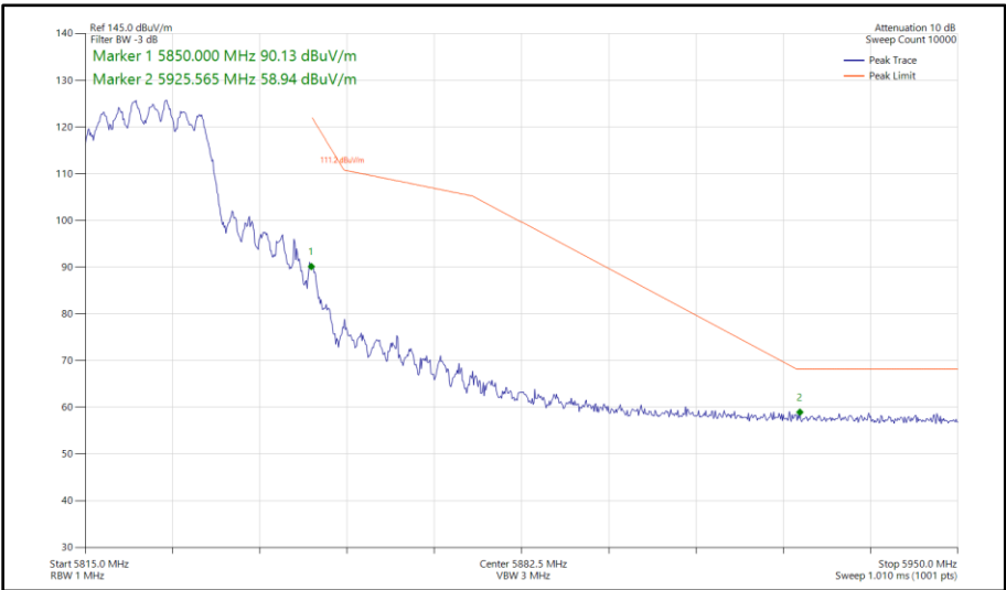
Figure 477 - 802.11ax HE20, SU, CDD, Core 0 - Core 1 - 5825 MHz Band Edge Frequency 5850 MHz
