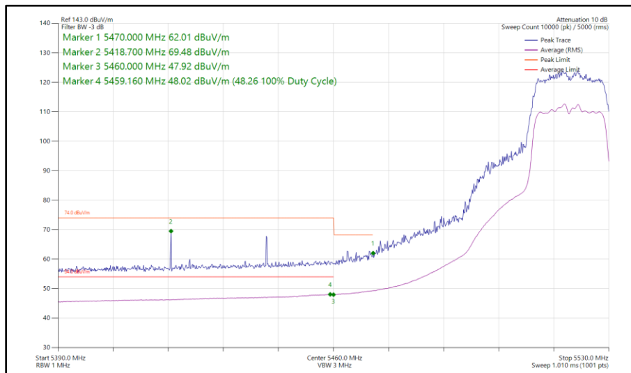
Figure 500 - 802.11ac VHT20, TxBF, Core 0 - Core 1 - 5520 MHz Band Edge Frequency 5470 MHz
