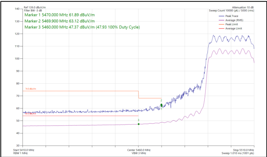
Figure 455 - 802.11ax HE20, SU, CDD, Core 0 - Core 1 - 5500 MHz Band Edge Frequency 5470 MHz
