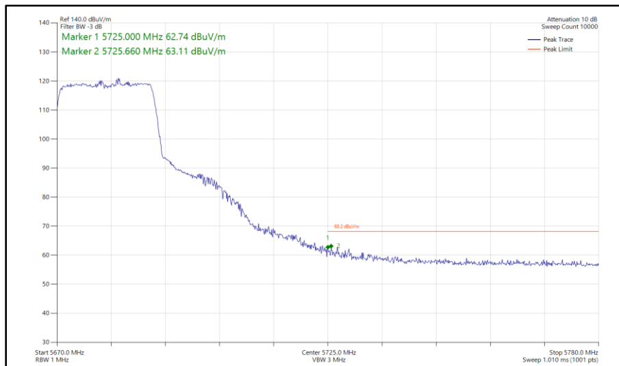
Figure 490 - 802.11ax HE20, SU, SDM, Core 0 - Core 1 - 5680 MHz Band Edge Frequency 5725 MHz
