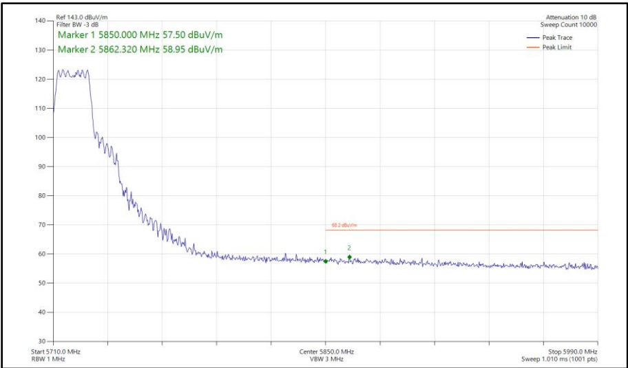
Figure 471 - 802.11n HT20, CDD, Core 0 - Core 1 - 5720 MHz Band Edge Frequency 5850 MHz
