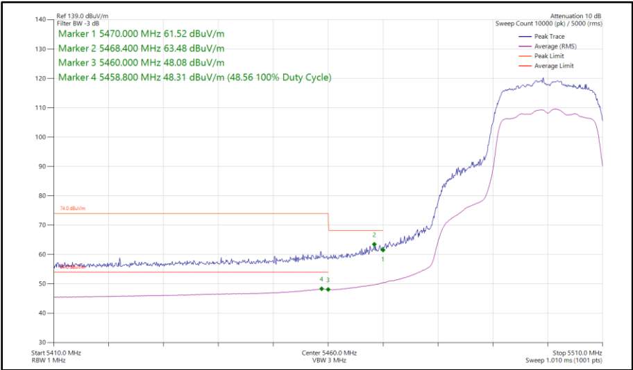
Figure 479 - 802.11n HT20, SDM, Core 0 - Core 1 - 5500 MHz Band Edge Frequency 5470 MHz
