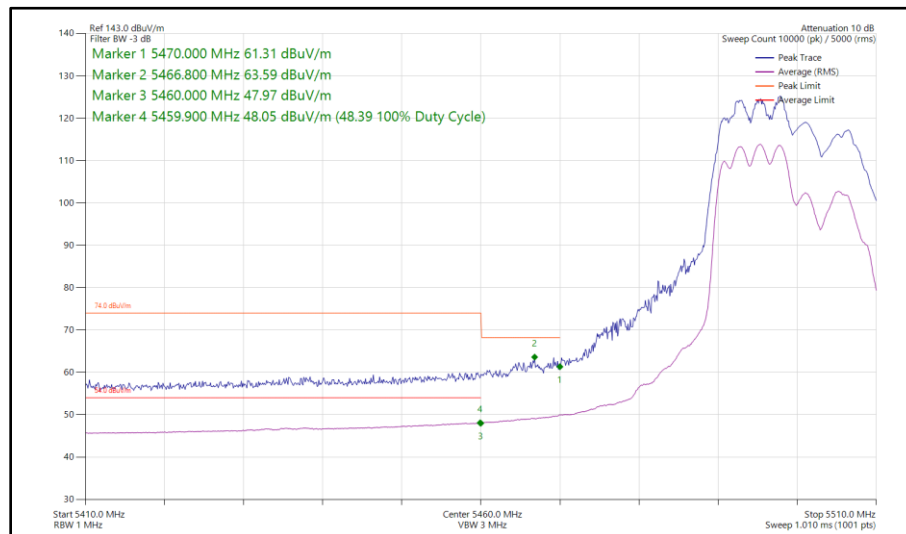
Figure 481 - 802.11ax HE20, RU 106-53, SDM, Core 0 - Core 1 - 5500 MHz Band Edge Frequency 5470 MHz
