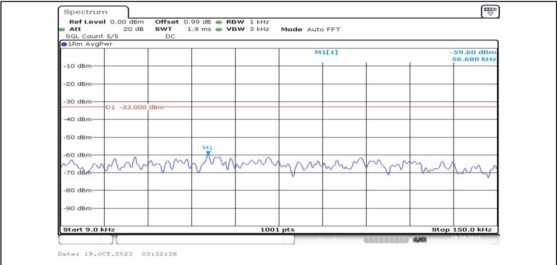
Band13-10MHz-QPSK-23230-1RB#0-Range1:0.009~0.15MHz-PASS
