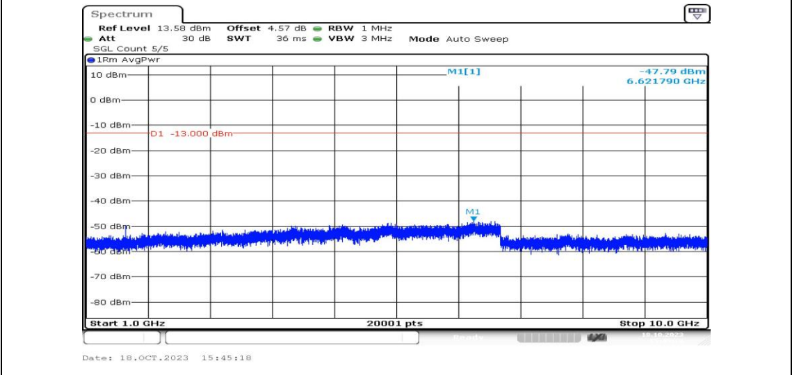
Band13-5MHz-QPSK-23255-1RB#0-Range4:1000~10000MHz-PASS
