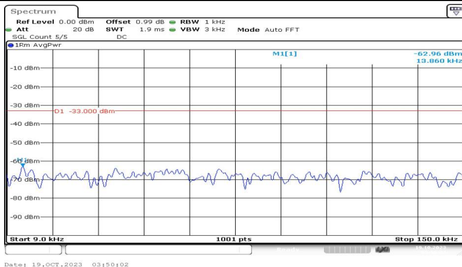
Band13-10MHz-16QAM-23230-1RB#0-Range1:0.009~0.15MHz-PASS
