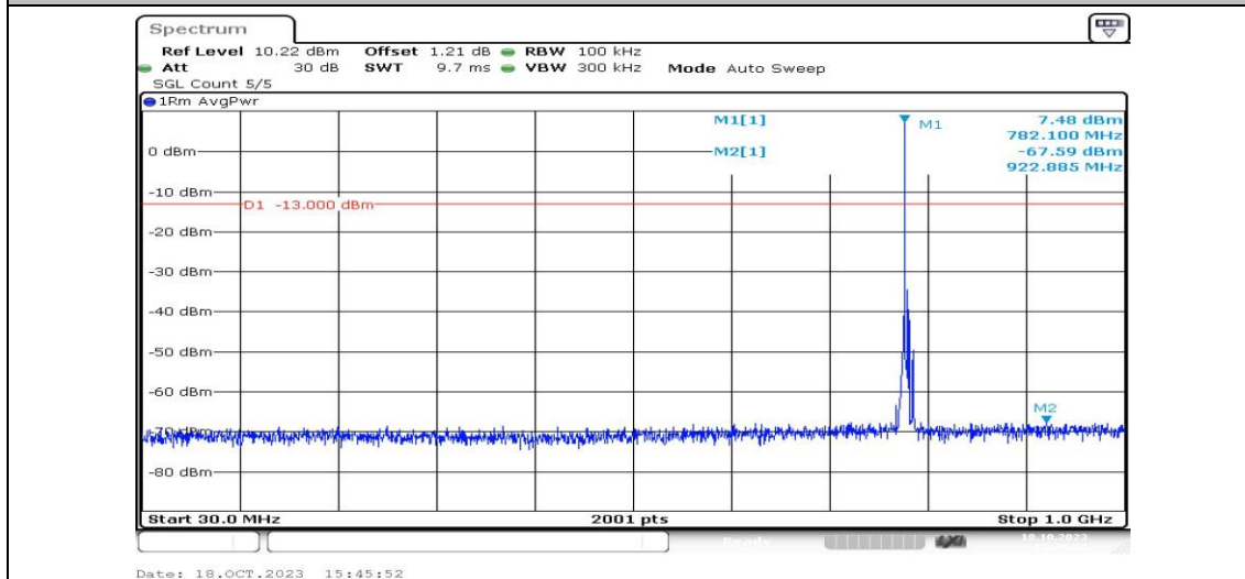
Band13-5MHz-16QAM-23255-1RB#0-Range3:30~1000MHz-PASS
