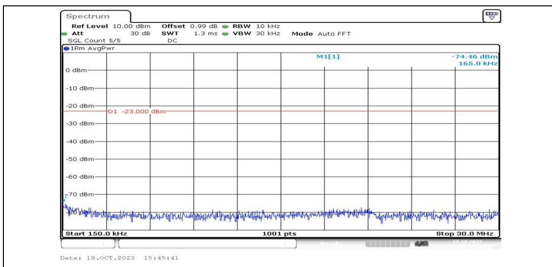
Band13-5MHz-16QAM-23255-1RB#0-Range2:0.15~30MHz-PASS
