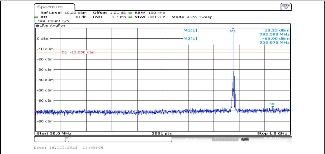
Band13-5MHz-QPSK-23255-1RB#0-Range3:30~1000MHz-PASS
