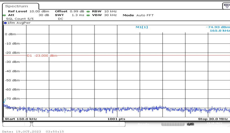
Band13-10MHz-16QAM-23230-1RB#0-Range2:0.15~30MHz-PASS
