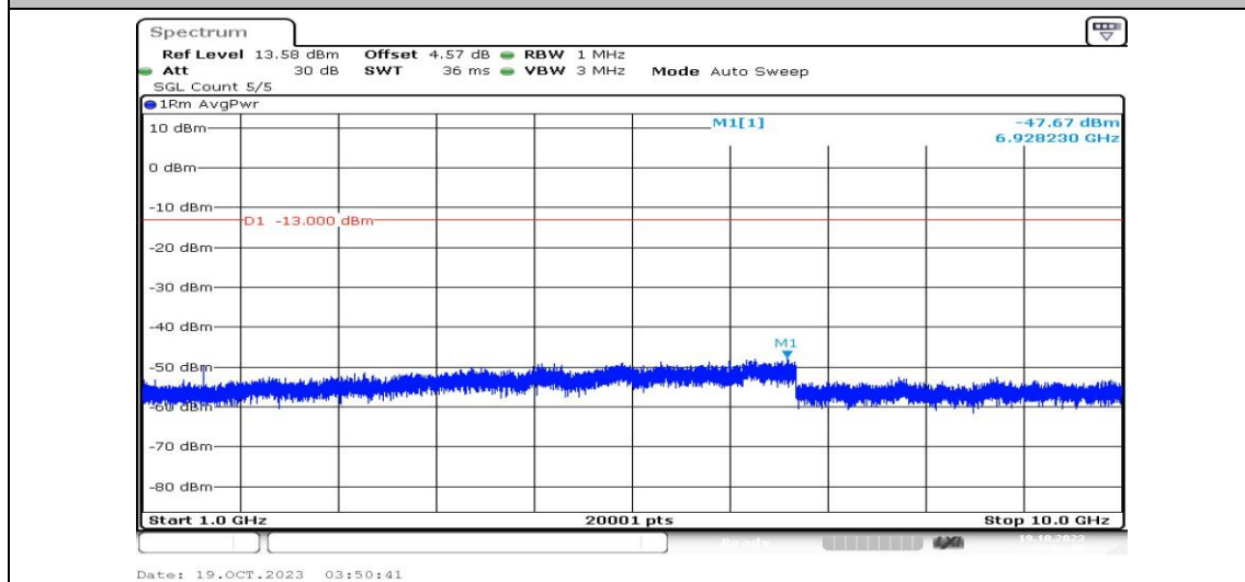
Band13-10MHz-16QAM-23230-1RB#0-Range4:1000~10000MHz-PASS
