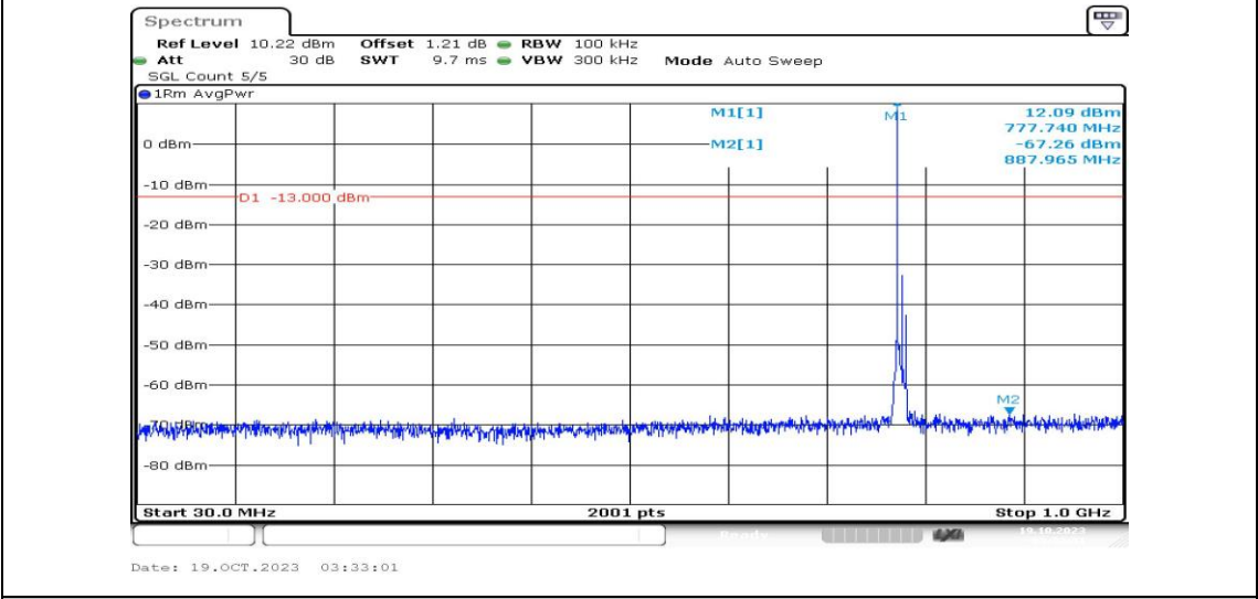
Band13-10MHz-QPSK-23230-1RB#0-Range3:30~1000MHz-PASS
