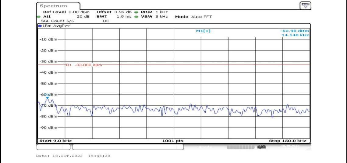
Band13-5MHz-16QAM-23255-1RB#0-Range1:0.009~0.15MHz-PASS
