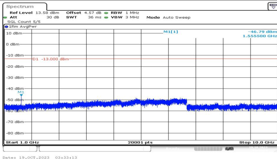
Band13-10MHz-QPSK-23230-1RB#0-Range4:1000~10000MHz-PASS
