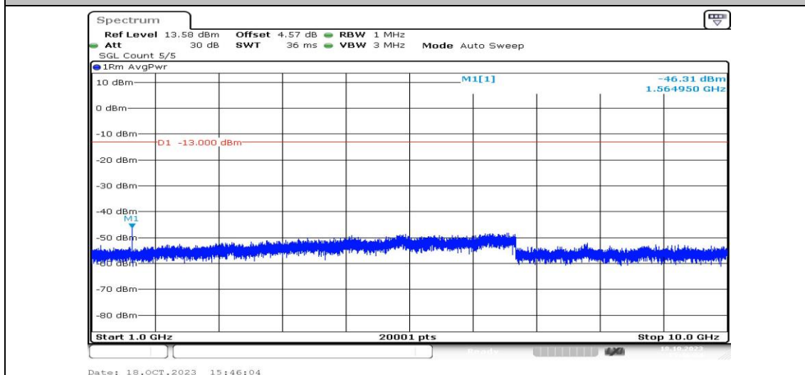
Band13-5MHz-16QAM-23255-1RB#0-Range4:1000~10000MHz-PASS
