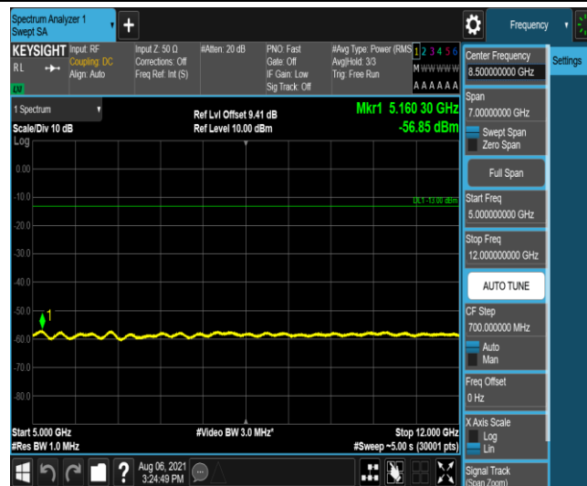
Band2-5MHz-16QAM-18900-6-0-Low-5000-12000--56.85-PASS
