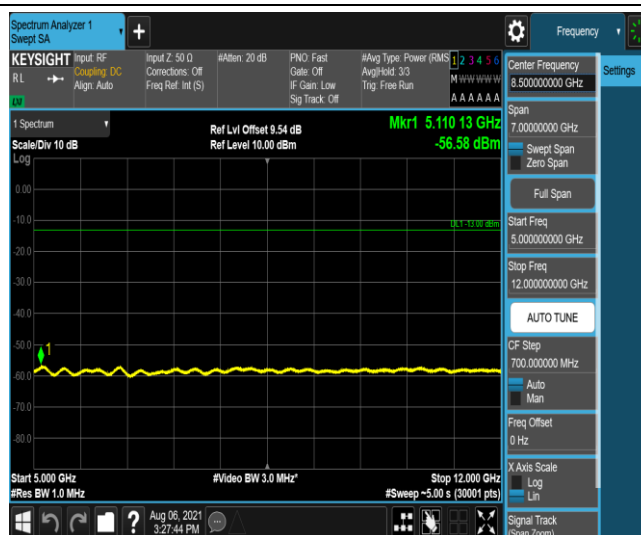
Band2-5MHz-16QAM-19175-1-5-Low-5000-12000--56.58-PASS
