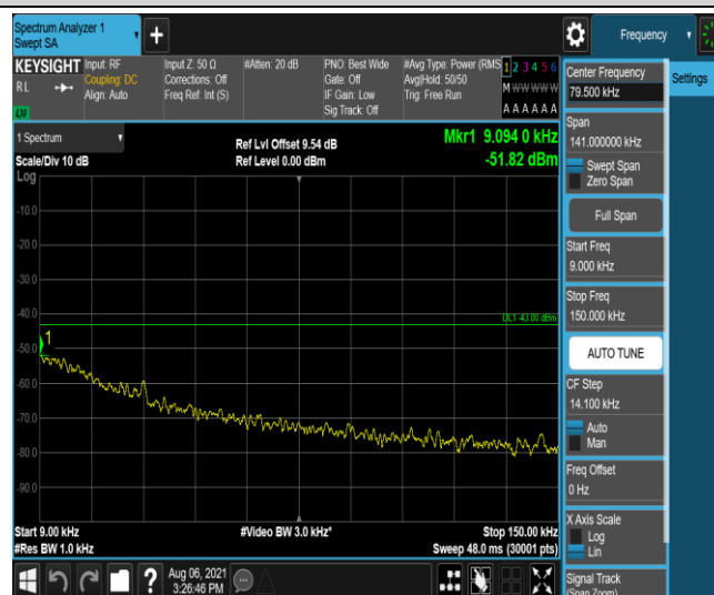
Band2-5MHz-16QAM-19175-1-5-Low-0.009-0.15--51.82-PASS
