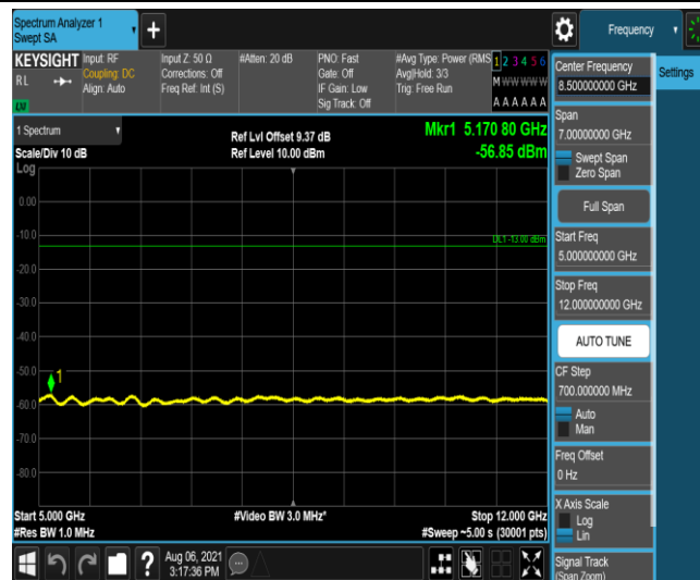
Band2-5MHz-QPSK-18625-6-0-Low-5000-12000--56.85-PASS
