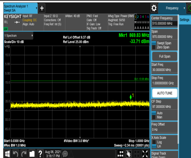
Band2-5MHz-16QAM-18625-6-0-Low-30-1000--33.71-PASS
