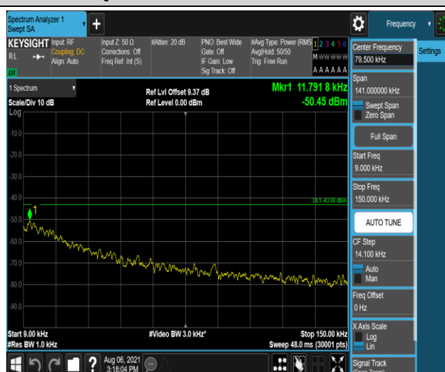
Band2-5MHz-16QAM-18625-6-0-Low-0.009-0.15--50.45-PASS
