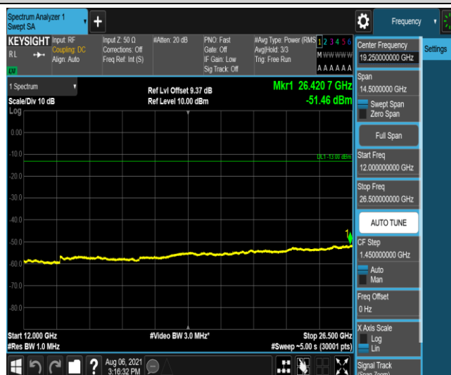
Band2-5MHz-16QAM-18625-1-0-Low-12000-26500--51.46-PASS
