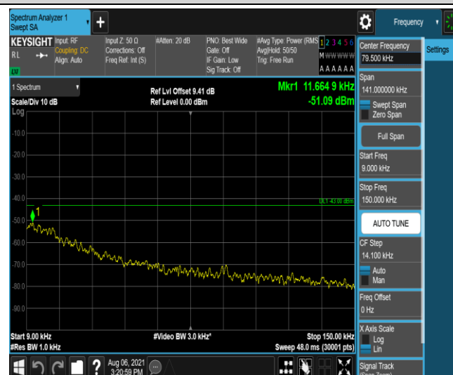
Band2-5MHz-16QAM-18900-1-0-Low-0.009-0.15--51.09-PASS
