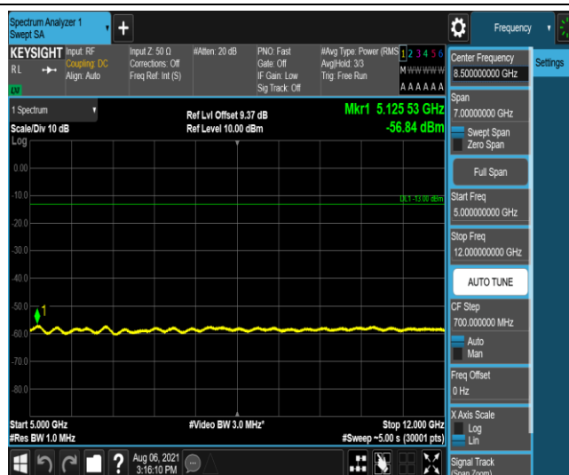
Band2-5MHz-16QAM-18625-1-0-Low-5000-12000--56.84-PASS
