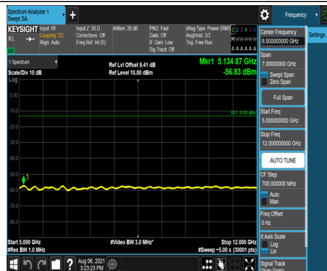
Band2-5MHz-QPSK-18900-6-0-Low-5000-12000--56.83-PASS
