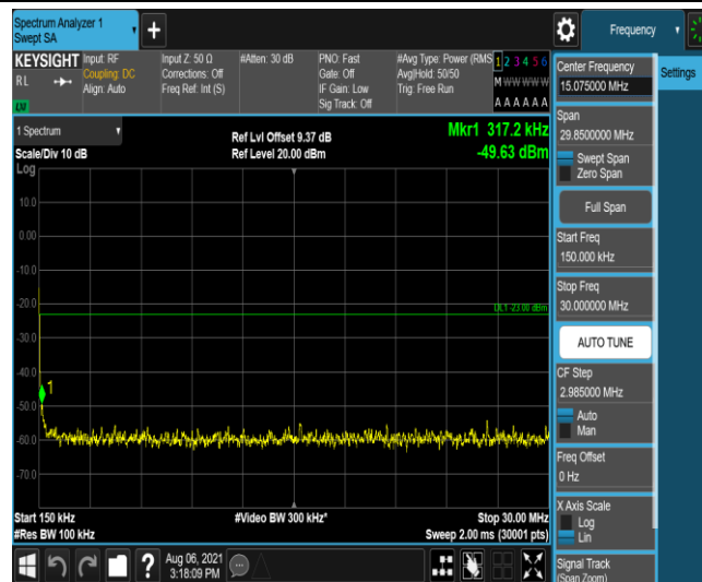
Band2-5MHz-16QAM-18625-6-0-Low-0.15-30--49.63-PASS
