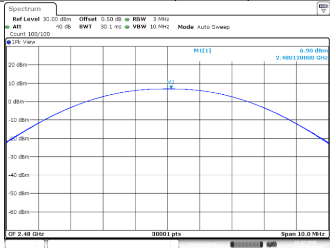
Channel 39 (2480MHz)
