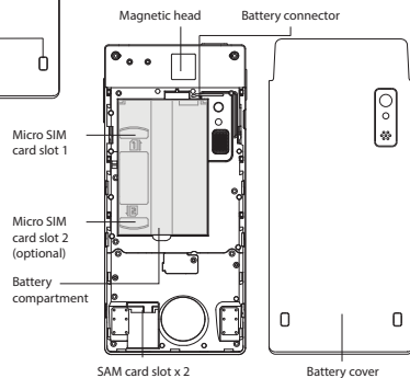
Fig. 3 - Internal View
