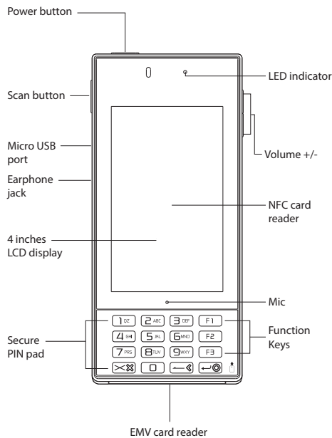
Fig.1- Front View
