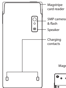
Fig. 2 - Back View
