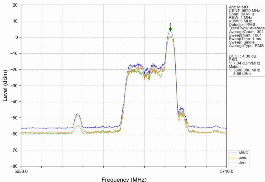
802.11ax(HEW40)_HCH_5670MHz_RU26_Right_MIMO_NTNV
