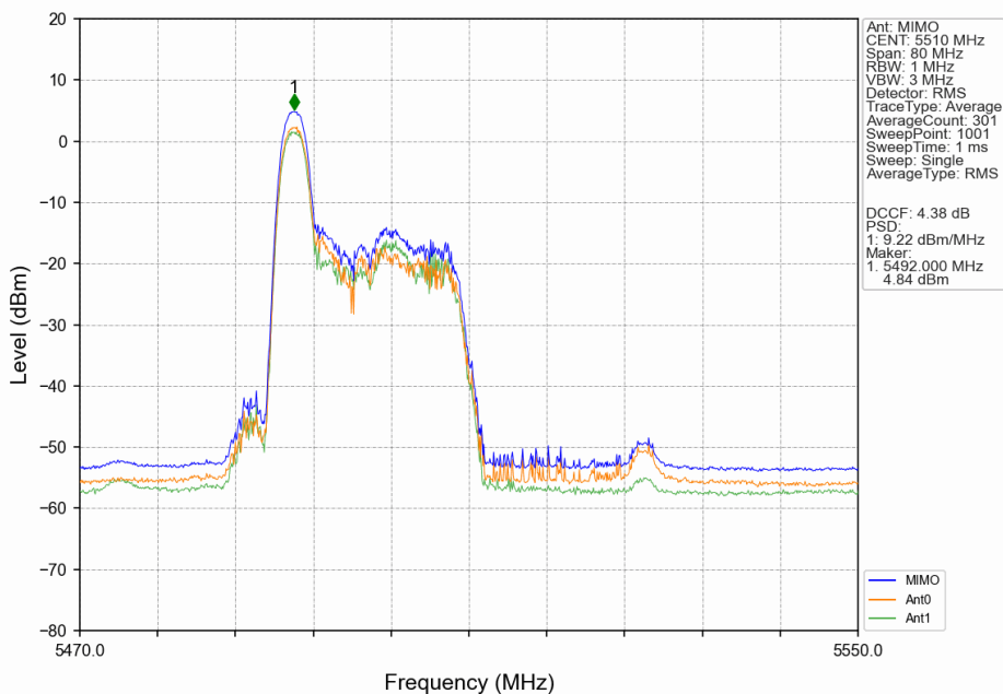
802.11ax(HEW40)_LCH_5510MHz_RU26_Left_MIMO_NTNV
