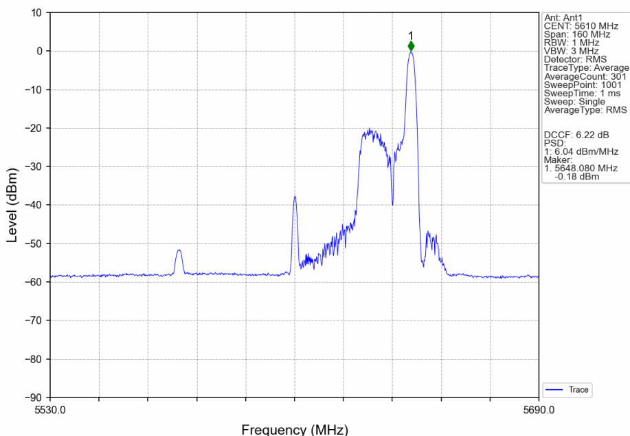
802.11ax(HEW80)_HCH_5610MHz_RU26_Right_MIMO_NTNV
