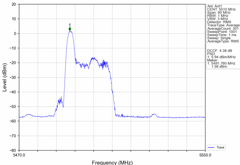
802.11ax(HEW40)_LCH_5510MHz_RU26_Left_MIMO_NTNV
