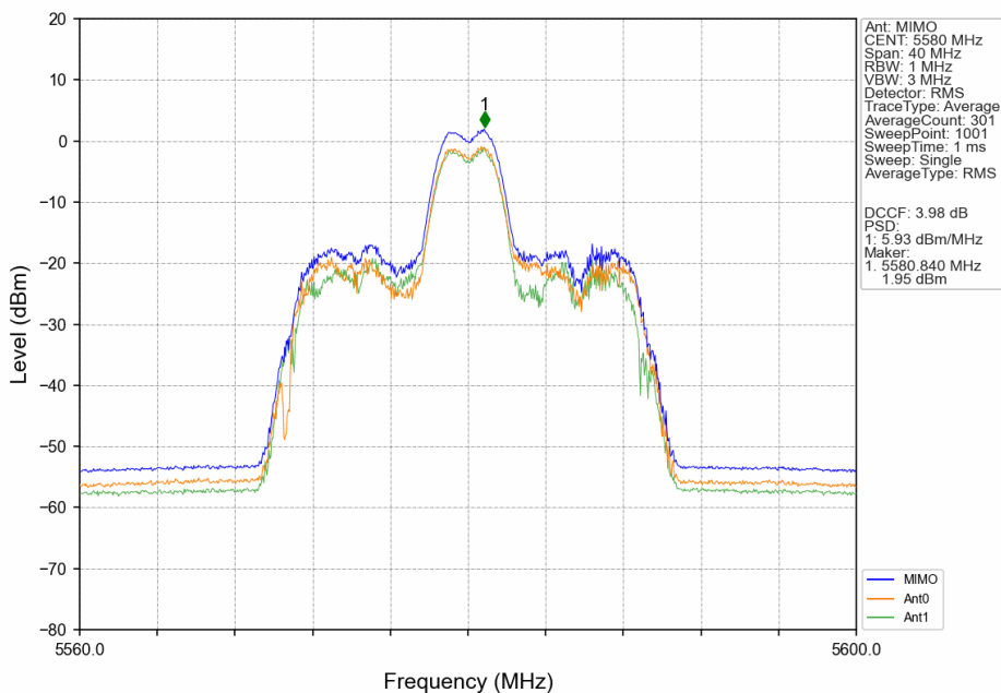
802.11ax(HEW20)_MCH_5580MHz_RU26_Mid_MIMO_NTNV
