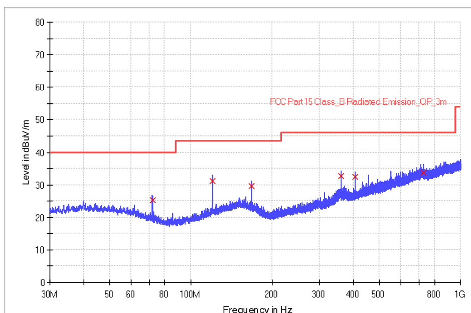
RE_VULB9168_pre_Cont_30-1000
