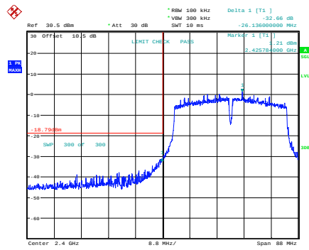
n40_2422MHz
