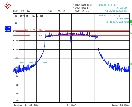
n40_2422MHz
