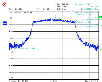
ax40_2437MHz
