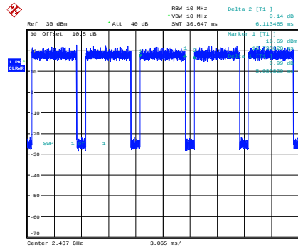
n20_2437MHz
