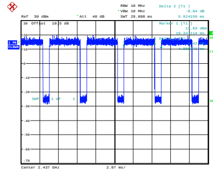
n40_2437MHz
