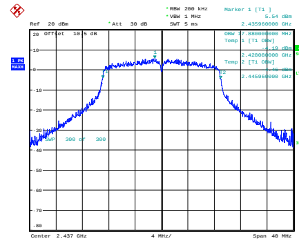
n20_2437MHz
