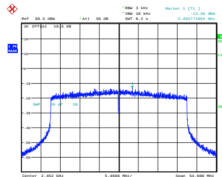
ax40_2452MHz
