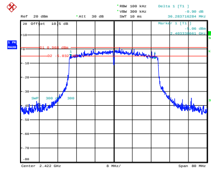
ax40_2422MHz
