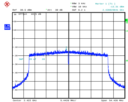
ax40_2422MHz
