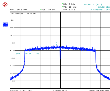
ax40_2437MHz
