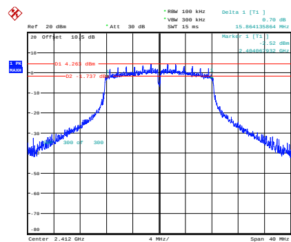
g_2412MHz
