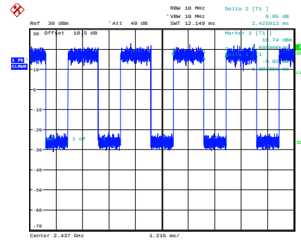
g_2437MHz_
