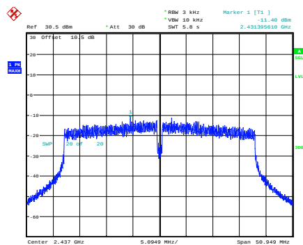
n40_2437MHz
