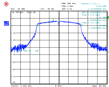
n40_2422MHz
