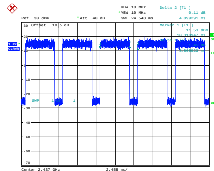
ax40_2437MHz
