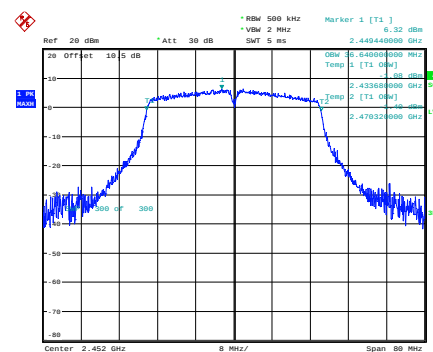
n40_2452MHz
