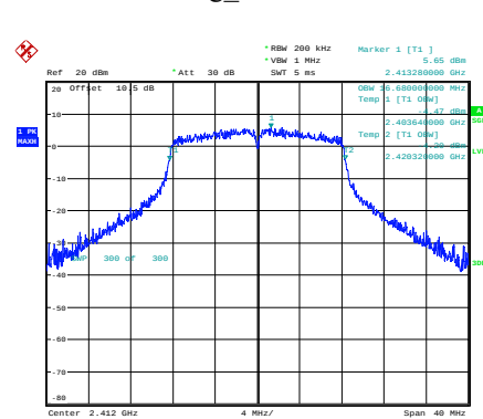
g_2412MHz
