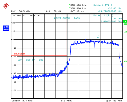
ax40_2422MHz
