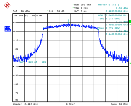
ax40_2422MHz
