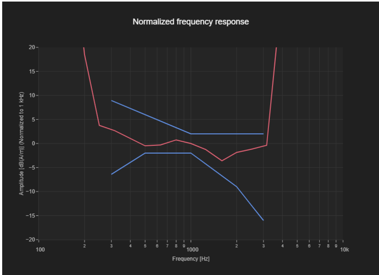
Figure C.1 Frequency Response of B66-N77
