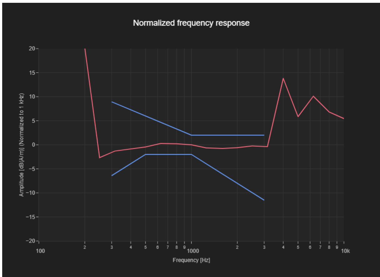
Figure C.2 Frequency Response of B2-N77-OTT
