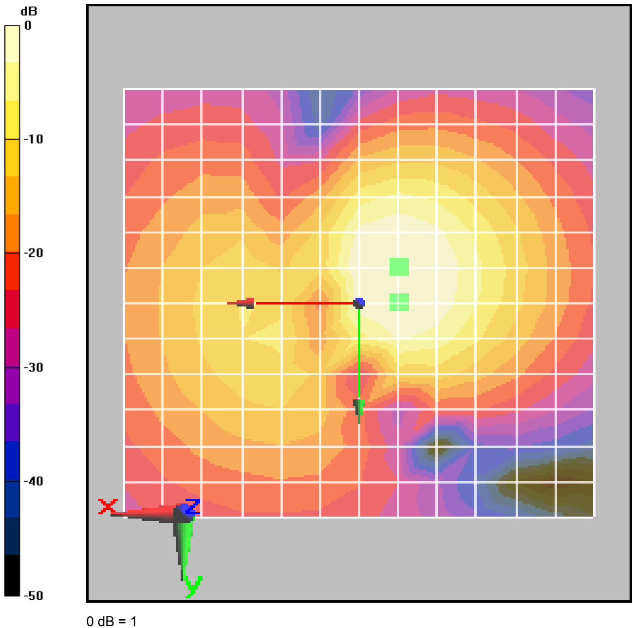
Figure 27 T-Coil WCDMA Band II Y transversal
