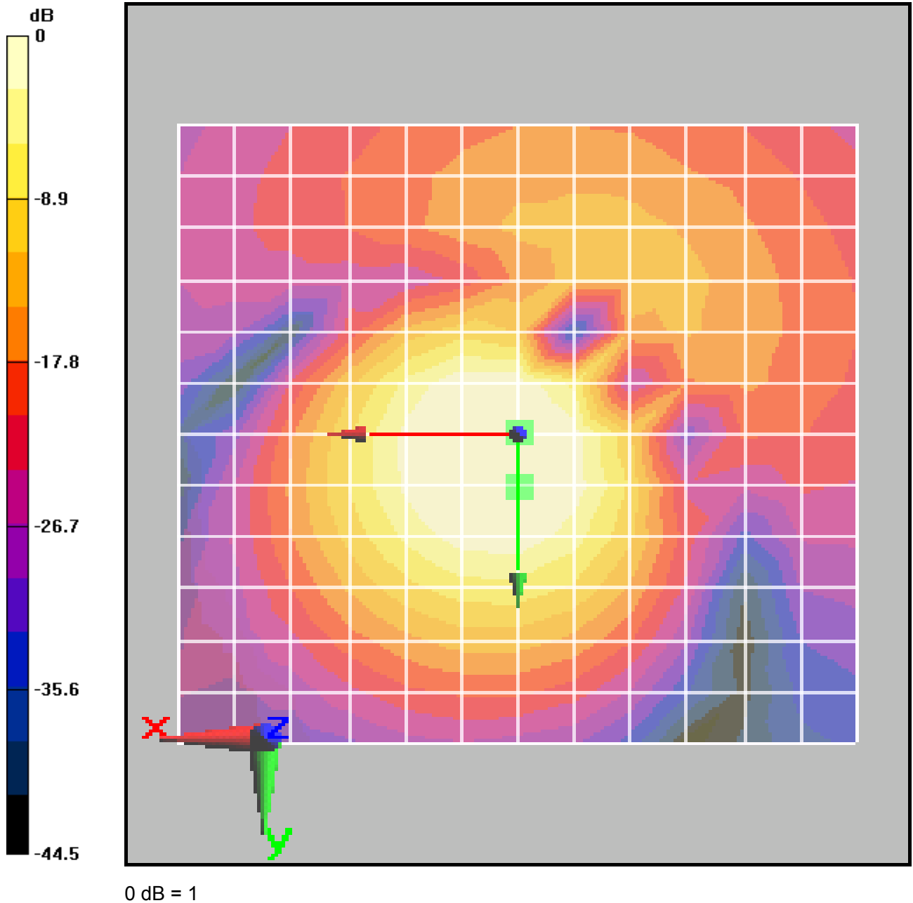
Figure 26 T-Coil WCDMA Band II X longitudinal
