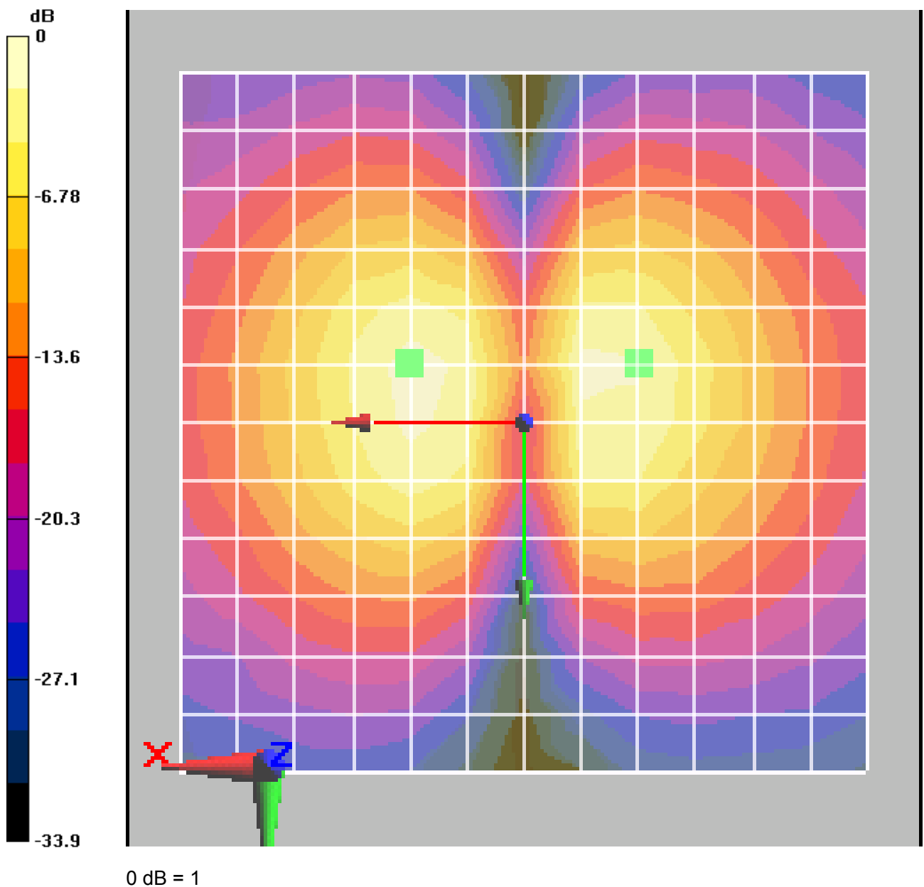
Figure 17 T-Coil GSM 1900 X longitudinal
