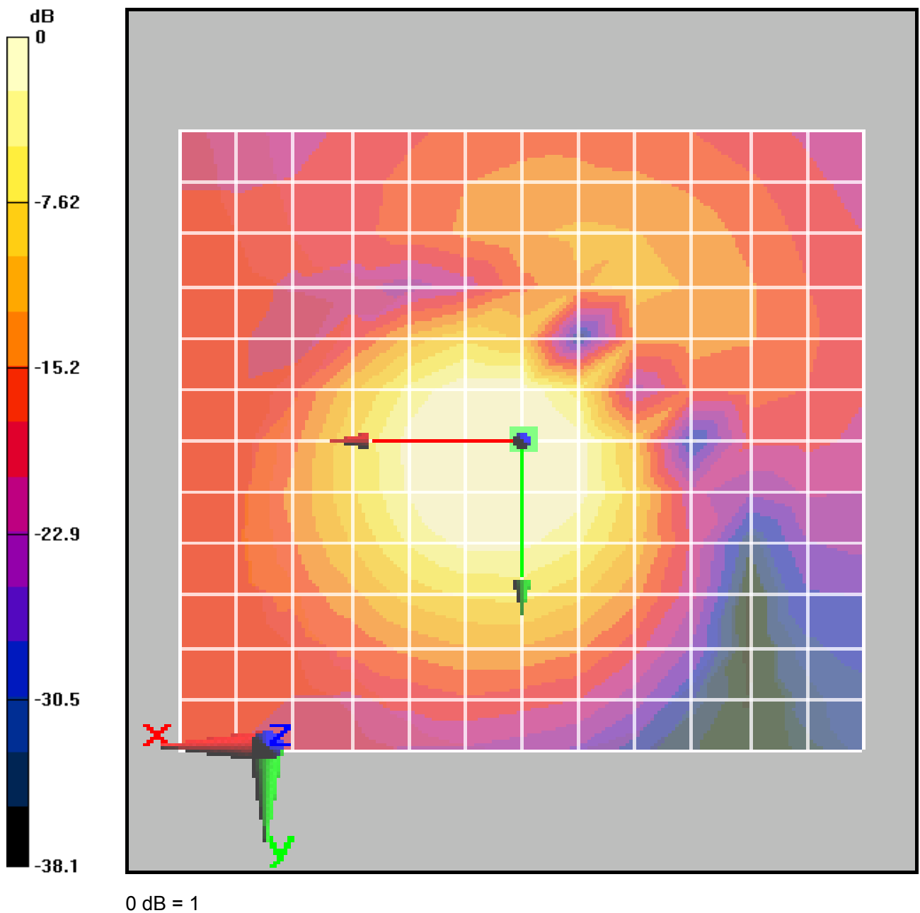
Figure 20 T-Coil GSM 1900 X longitudinal
