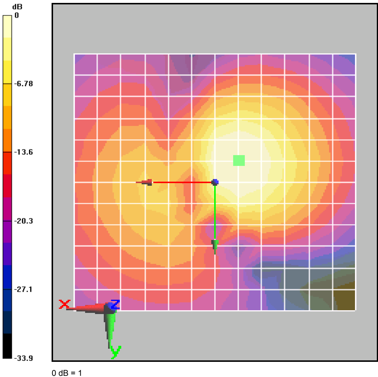
Figure 21 T-Coil GSM 1900 Y transversal
