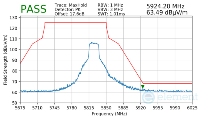
Plot 7-58. (Pk, Ch.165, 802.11n, MCS7)
