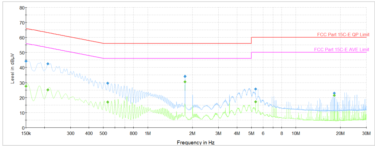
Plot 7-61. AC Line Conducted Plot with 802.11n – Ch.157 (L1), with AC/DC Adapter & magnetic charger
