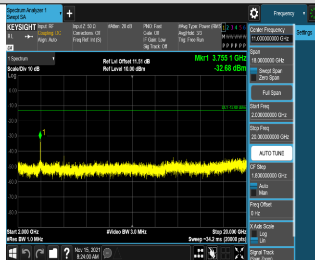
Band2-5MHz-QPSK-18900-1RB#0-Range3:2000~20000MHz
