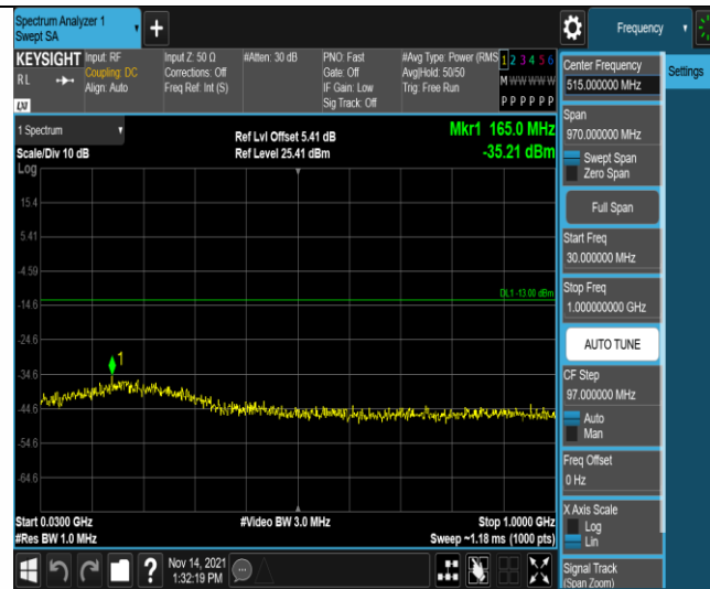
Band2-1.4MHz-QPSK-19193-1RB#0-Range1:30~1000MHz
