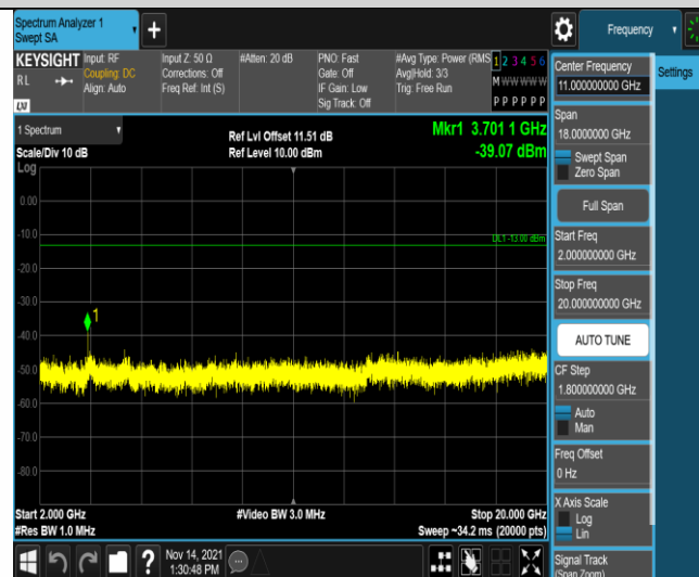
Band2-1.4MHz-16QAM-18607-1RB#0-Range3:2000~20000MHz
