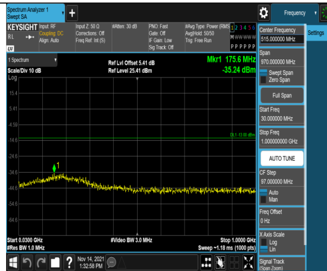
Band2-1.4MHz-16QAM-19193-1RB#0-Range1:30~1000MHz
