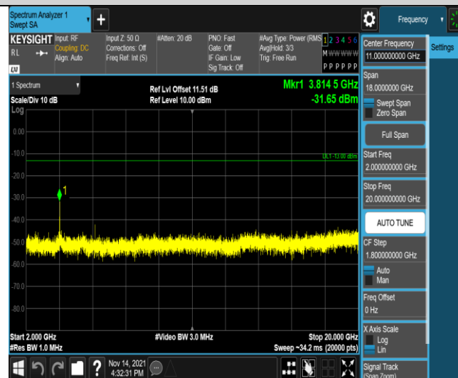
Band2-3MHz-16QAM-19185-1RB#0-Range3:2000~20000MHz
