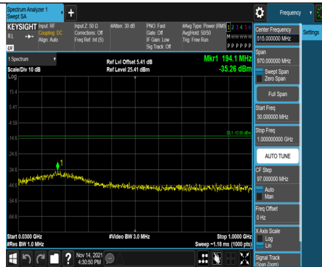
Band2-3MHz-16QAM-18900-1RB#0-Range1:30~1000MHz
