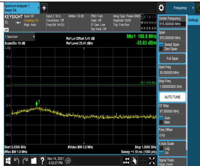
Band2-3MHz-16QAM-19185-1RB#0-Range1:30~1000MHz
