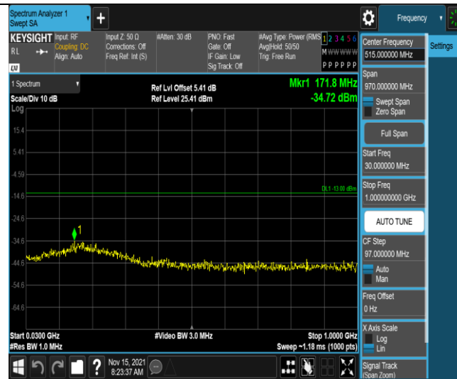
Band2-5MHz-QPSK-18900-1RB#0-Range1:30~1000MHz
