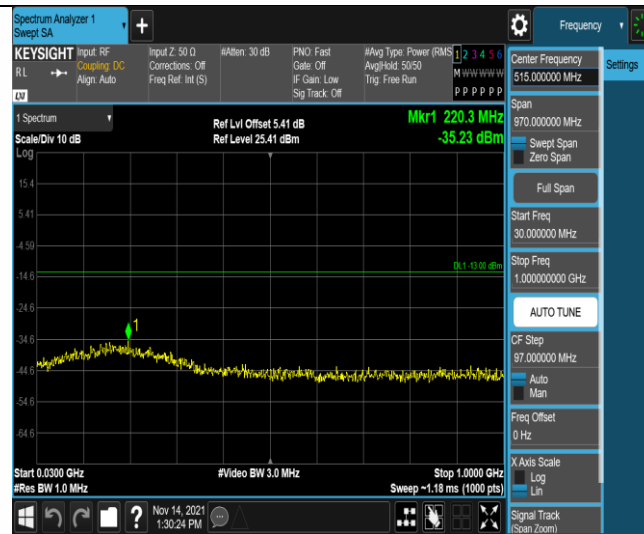
Band2-1.4MHz-16QAM-18607-1RB#0-Range1:30~1000MHz
