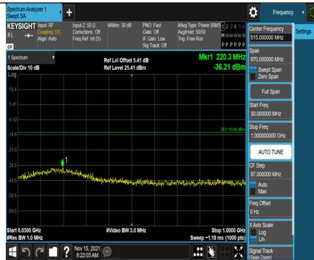
Band2-5MHz-QPSK-18625-1RB#0-Range1:30~1000MHz
