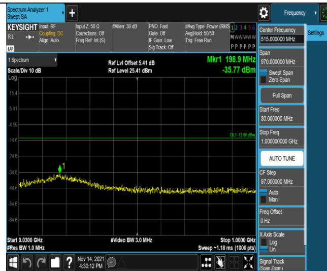
Band2-3MHz-QPSK-18900-1RB#0-Range1:30~1000MHz
