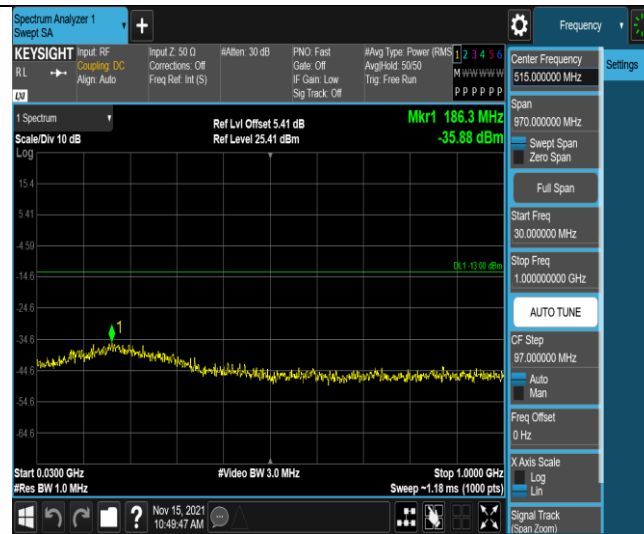
Band2-10MHz-QPSK-18650-1RB#0-Range1:30~1000MHz
