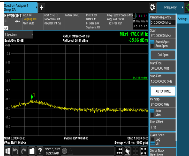
Band2-5MHz-16QAM-18900-1RB#0-Range1:30~1000MHz
