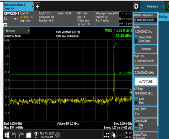
Band2-5MHz-16QAM-18625-1RB#0-Range2:1000~2000MHz
