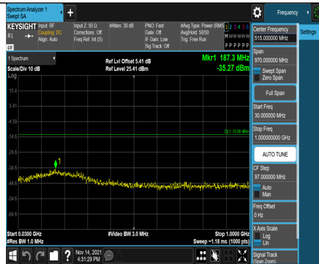
Band2-3MHz-QPSK-19185-1RB#0-Range1:30~1000MHz
