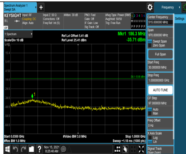
Band2-5MHz-16QAM-19175-1RB#0-Range1:30~1000MHz
