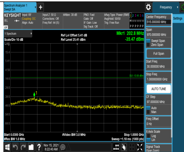
Band2-5MHz-16QAM-18625-1RB#0-Range1:30~1000MHz
