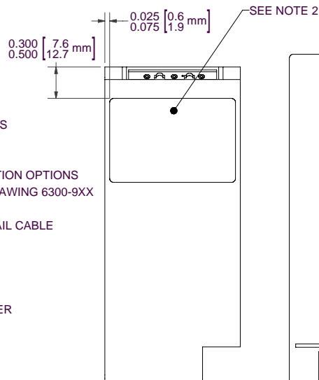
FRONT VIEW SHOWN WITHOUT BEZEL ASSEMBLY FOR CLARITY
