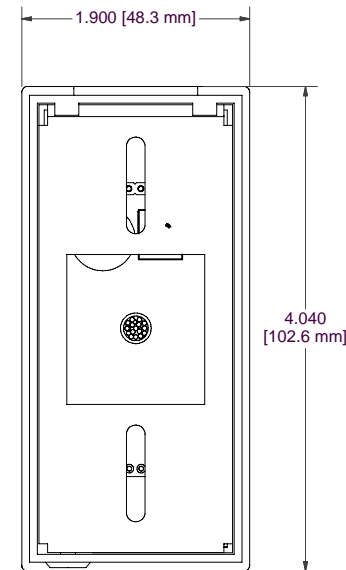
BACK VIEW PIGTAIL VERISON SHOWN
