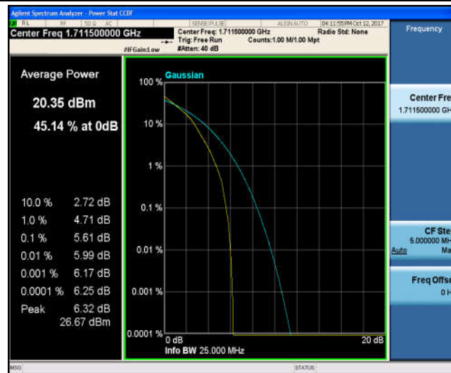
Band4_3MHz_16QAM_19965_1RB#0_6.13_13_PASS
