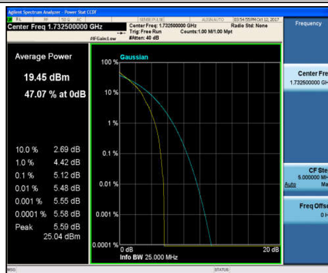
Band4_1.4MHz_16QAM_20175_1RB#0_5.44_13_PASS
