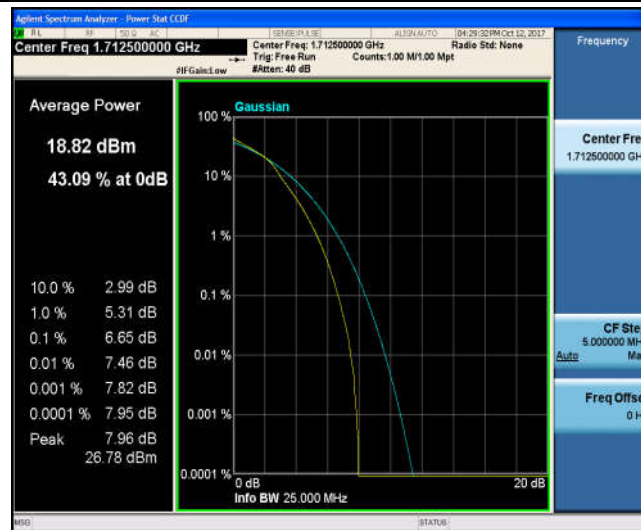
Band4_5MHz_QPSK_20175_1RB#0_5.17_13_PASS
