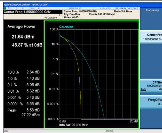
Band2_10MHz_16QAM_18650_1RB#0_6.03_13_PASS
