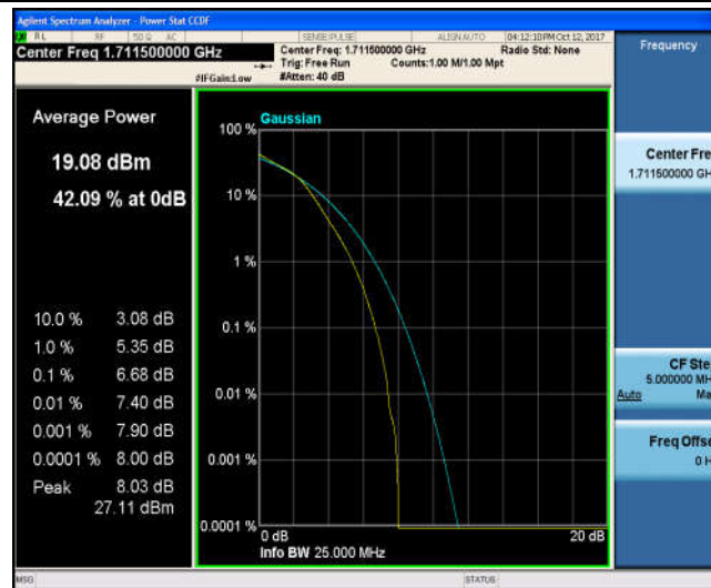
Band4_3MHz_QPSK_20175_1RB#0_5.11_13_PASS
