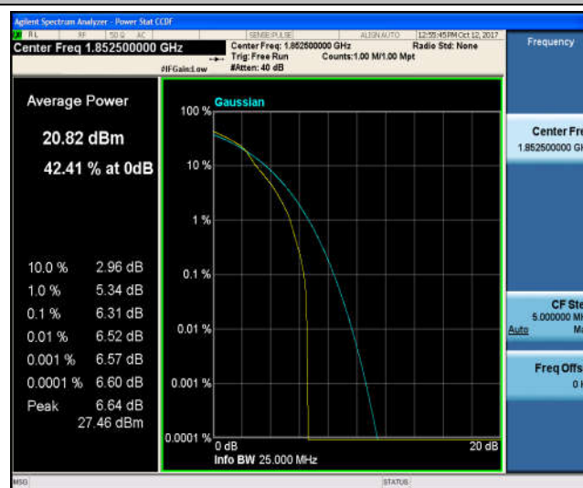
Band2_5MHz_QPSK_18625_25RB#0_5.62_13_PASS
