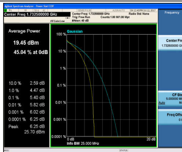
Band4_3MHz_16QAM_20175_15RB#0_6.17_13_PASS
