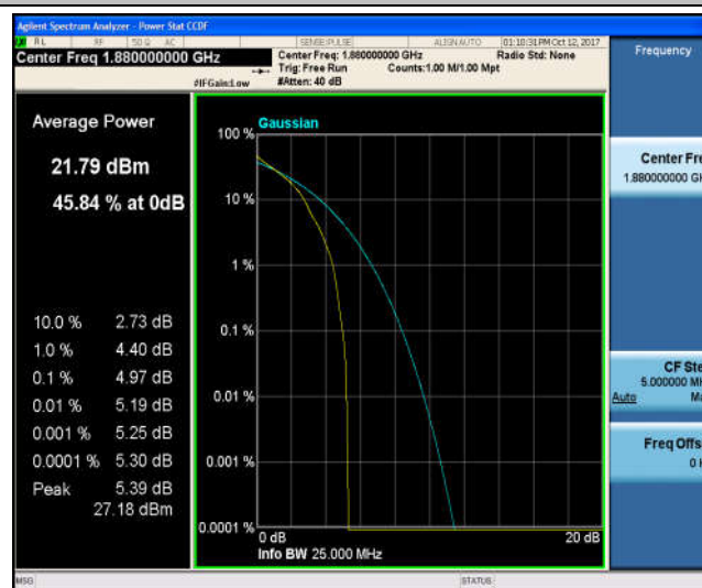
Band2_10MHz_16QAM_18900_1RB#0_5.67_13_PASS
