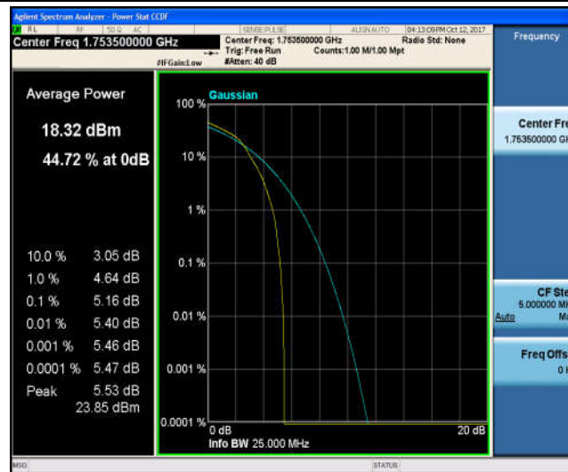
Band4_3MHz_QPSK_20385_15RB#0_5.18_13_PASS
