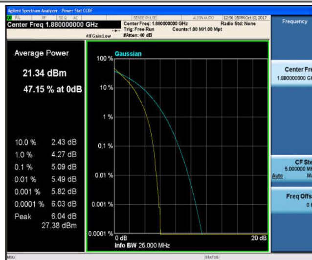
Band2_5MHz_16QAM_18900_25RB#0_5.98_13_PASS
