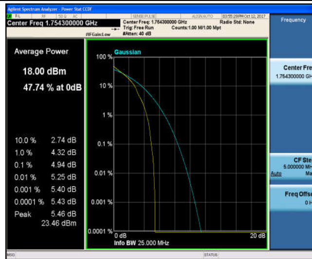
Band4_1.4MHz_16QAM_20393_1RB#0_5.40_13_PASS
