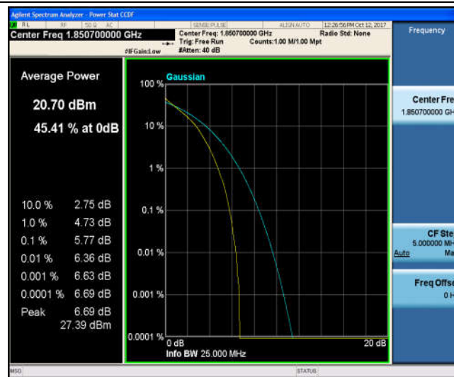
Band2_1.4MHz_16QAM_18607_6RB#0_6.69_13_PASS
