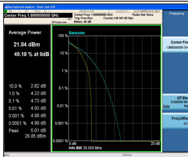
Band2_1.4MHz_16QAM_18900_1RB#0_5.29_13_PASS
