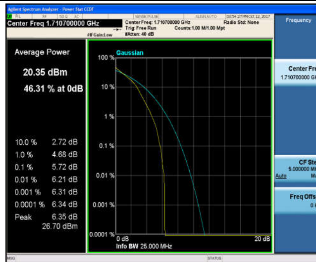
Band4_1.4MHz_16QAM_19957_1RB#0_6.35_13_PASS
