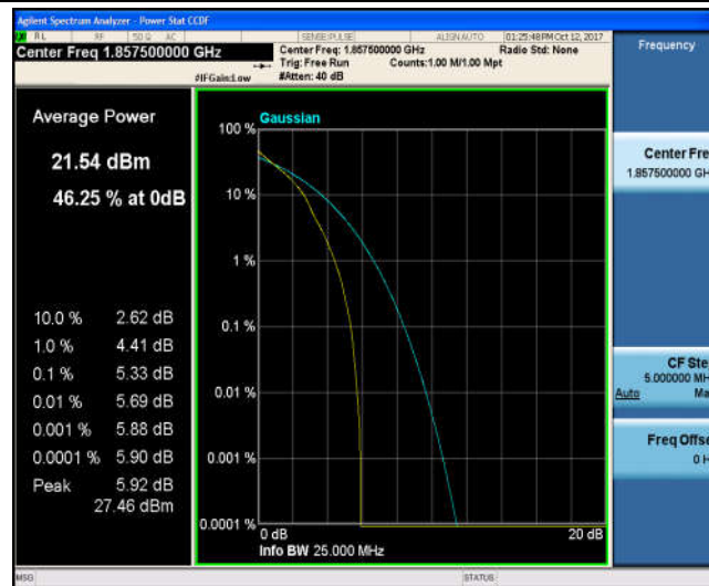
Band2_15MHz_16QAM_18675_1RB#0_6.44_13_PASS
