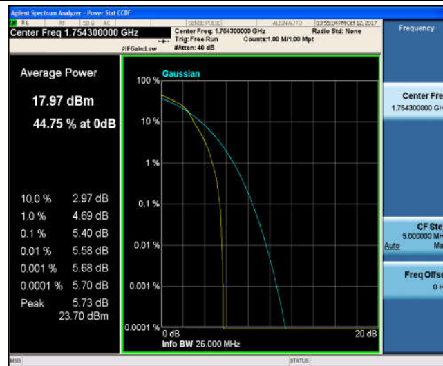
Band4_1.4MHz_QPSK_20393_6RB#0_5.11_13_PASS
