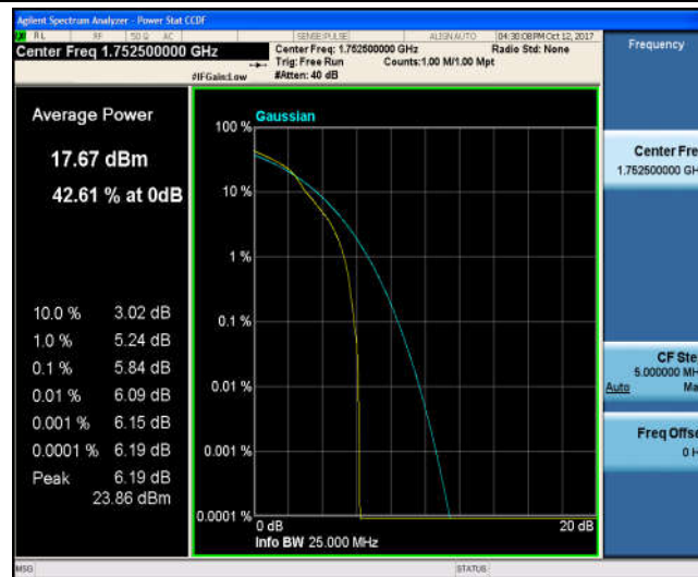
Band4_5MHz_QPSK_20375_25RB#0_5.25_13_PASS
