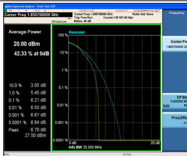
Band2_1.4MHz_QPSK_18607_6RB#0_5.77_13_PASS
