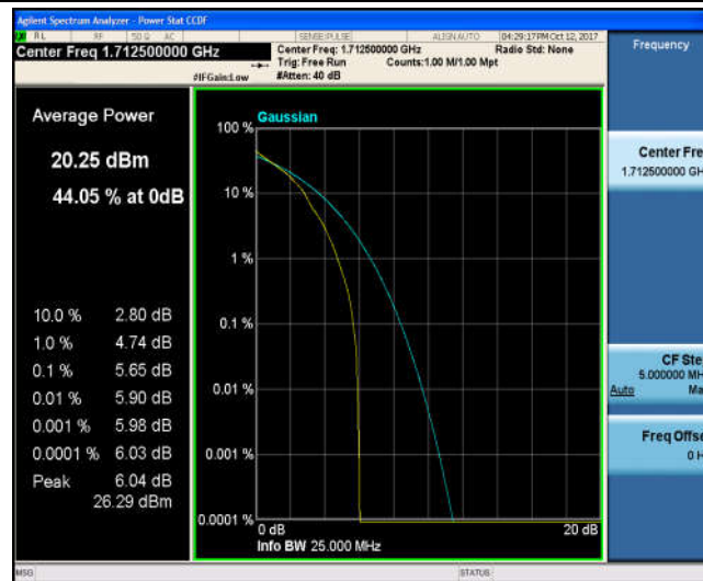
Band4_5MHz_16QAM_19975_1RB#0_6.56_13_PASS
