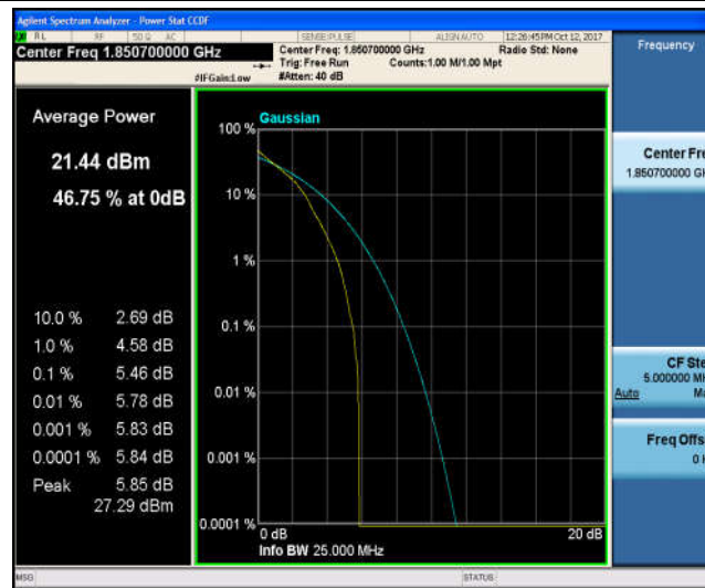
Band2_1.4MHz_16QAM_18607_1RB#0_6.21_13_PASS
