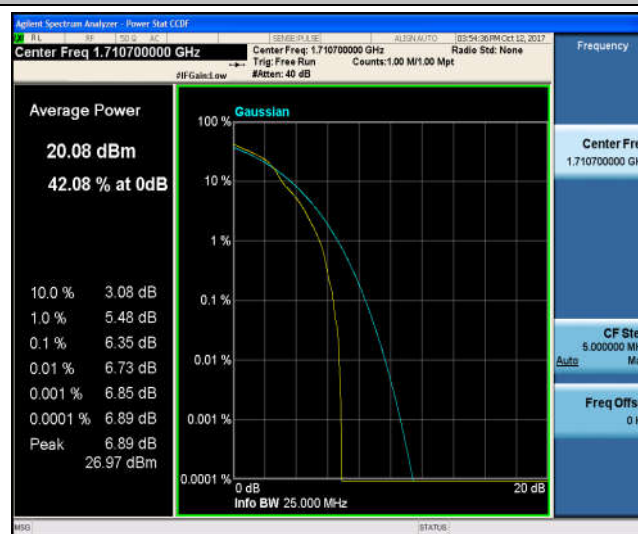
Band4_1.4MHz_QPSK_19957_6RB#0_5.92_13_PASS
