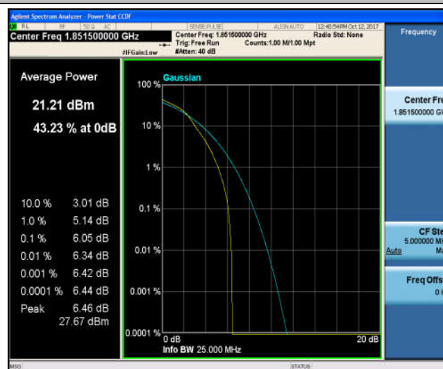
Band2_3MHz_QPSK_18615_15RB#0_5.68_13_PASS
