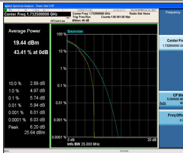
Band4_5MHz_QPSK_20175_25RB#0_5.42_13_PASS
