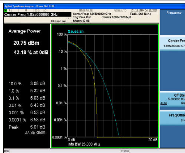
Band2_10MHz_QPSK_18650_50RB#0_5.58_13_PASS
