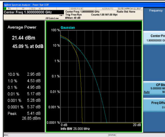
Band2_20MHz_QPSK_19100_100RB#0_5.28_13_PASS
