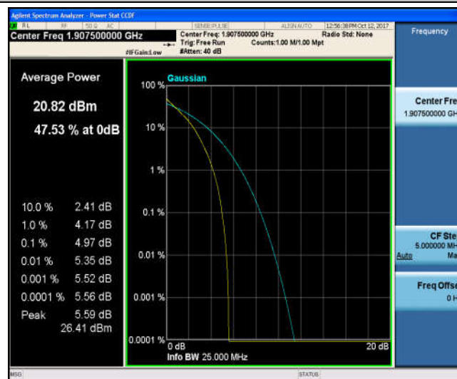
Band2_5MHz_16QAM_19175_25RB#0_5.84_13_PASS
