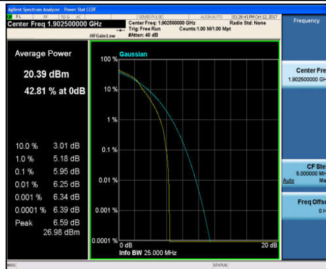
Band2_15MHz_QPSK_19125_75RB#0_5.46_13_PASS
