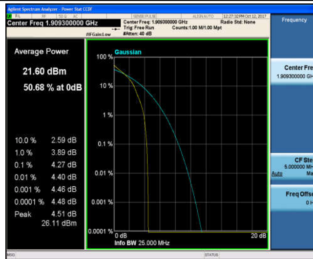
Band2_1.4MHz_16QAM_19193_1RB#0_5.14_13_PASS
