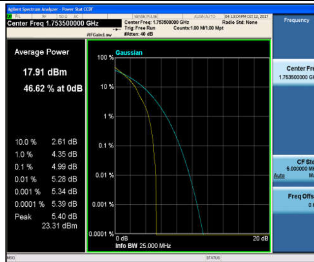
Band4_3MHz_16QAM_20385_1RB#0_5.16_13_PASS
