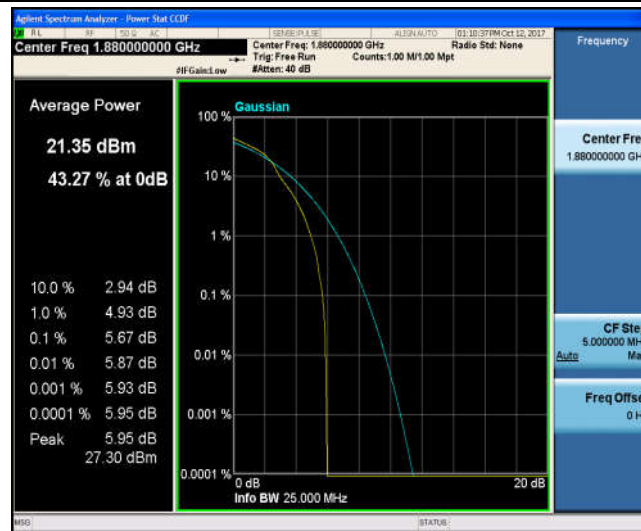
Band2_10MHz_QPSK_18900_50RB#0_5.02_13_PASS
