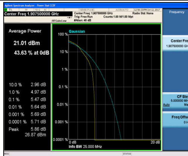
Band2_5MHz_QPSK_19175_25RB#0_4.97_13_PASS
