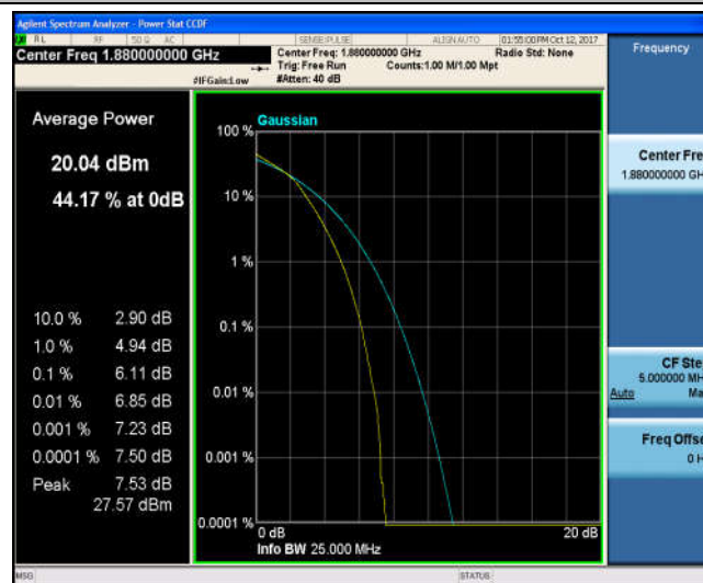
Band2_20MHz_QPSK_19100_1RB#0_4.70_13_PASS
