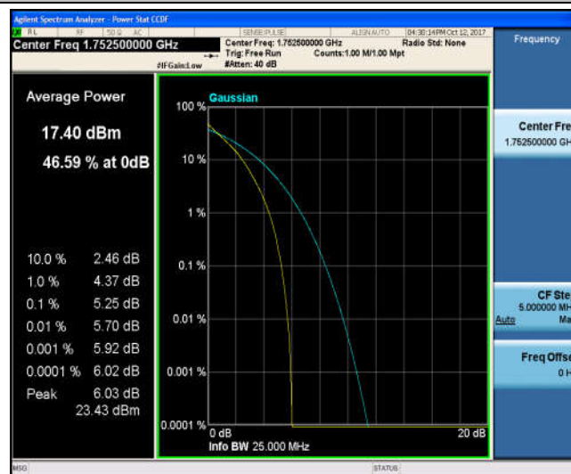
Band4_5MHz_16QAM_20375_25RB#0_6.05_13_PASS
