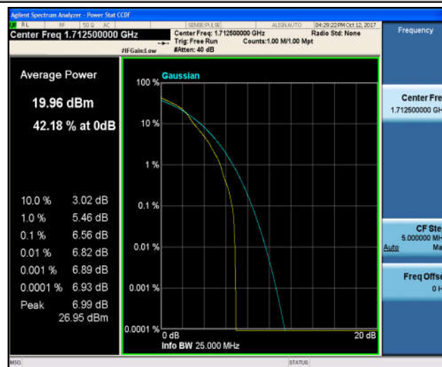
Band4_5MHz_QPSK_19975_25RB#0_5.75_13_PASS
