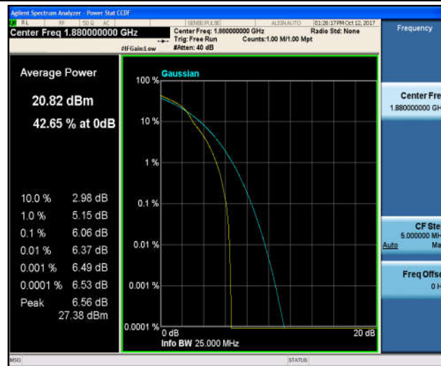
Band2_15MHz_QPSK_18900_75RB#0_5.42_13_PASS
