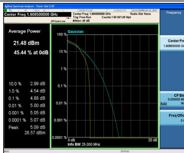
Band2_3MHz_QPSK_19185_15RB#0_4.89_13_PASS
