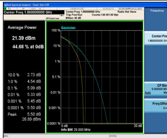
Band2_20MHz_16QAM_18700_1RB#0_5.28_13_PASS
