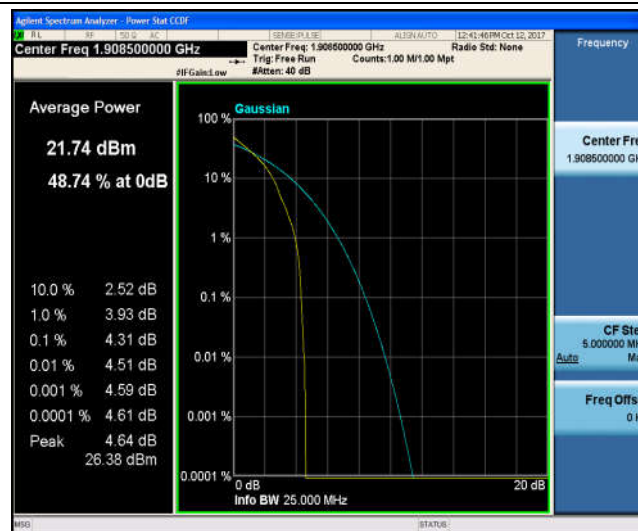
Band2_3MHz_16QAM_19185_1RB#0_4.88_13_PASS
