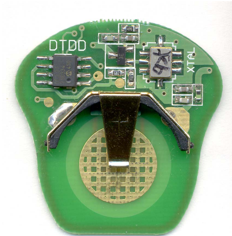
TRANSMITTER FRONT
