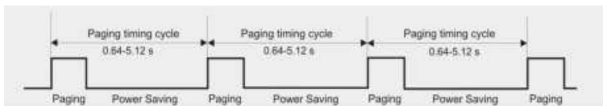
Figure 25: Power saving and paging in WCDMA networks
