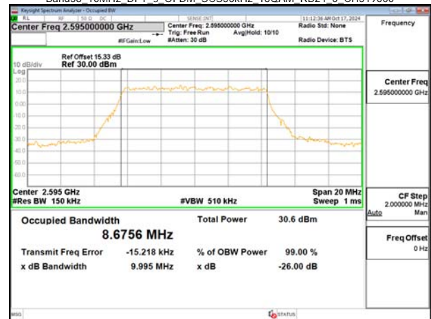
Band38_10MHz_DFT_s_OFDM_SCS30kHz_16QAM_RB24_0_CH519000
