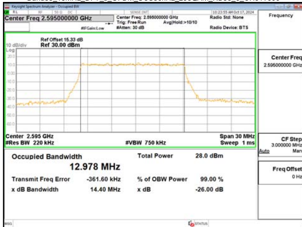
Band38_15MHz_DFT_s_OFDM_SCS30kHz_256QAM_RB36_0_CH519000
