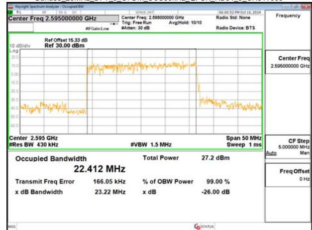
Band38_25MHz_DFT_s_OFDM_SCS30kHz_QPSK_RB64_0_CH519000
