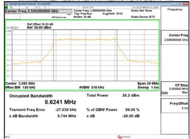
Band38_10MHz_DFT_s_OFDM_SCS30kHz_256QAM_RB24_0_CH519000
