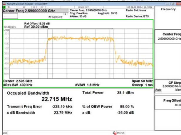
Band38_25MHz_DFT_s_OFDM_SCS30kHz_BPSK_RB64_0_CH519000
