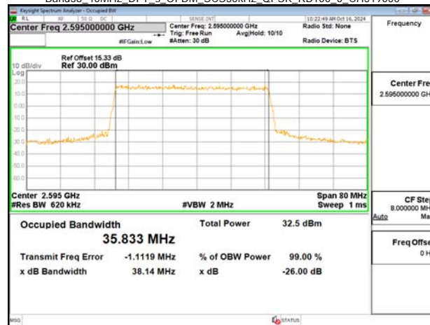
Band38_40MHz_DFT_s_OFDM_SCS30kHz_QPSK_RB100_0_CH519000
