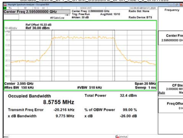
Band38_10MHz_DFT_s_OFDM_SCS30kHz_BPSK_RB24_0_CH519000
