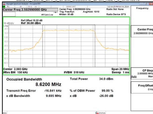
Band41_10MHz_DFT_s_OFDM_SCS30kHz_QPSK_RB24_0_CH518598
