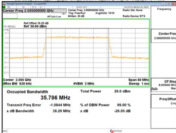
Band38_40MHz_DFT_s_OFDM_SCS30kHz_256QAM_RB100_0_CH519000
