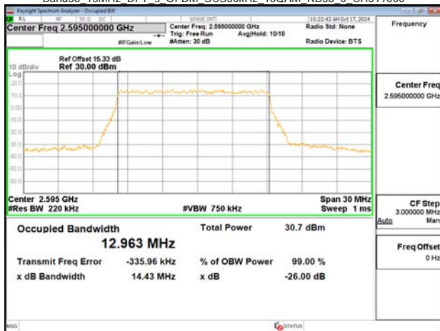
Band38_15MHz_DFT_s_OFDM_SCS30kHz_16QAM_RB36_0_CH519000
