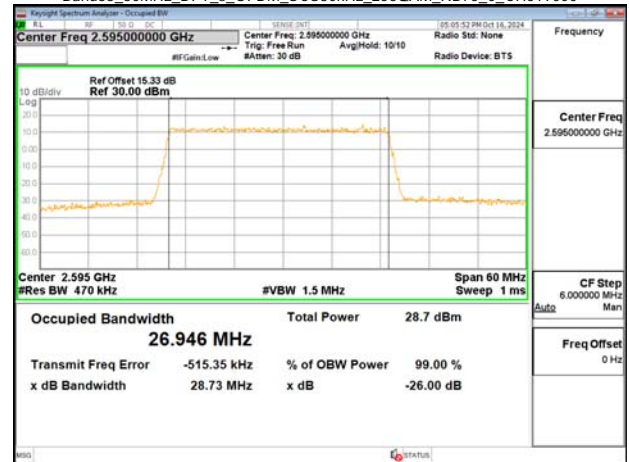
Band38_30MHz_DFT_s_OFDM_SCS30kHz_256QAM_RB75_0_CH519000
