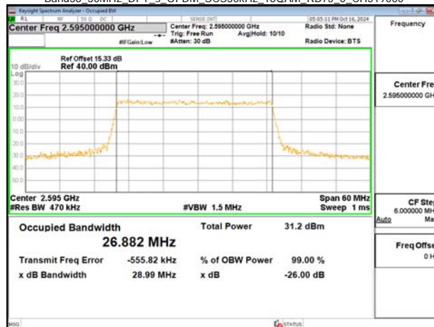
Band38_30MHz_DFT_s_OFDM_SCS30kHz_16QAM_RB75_0_CH519000
