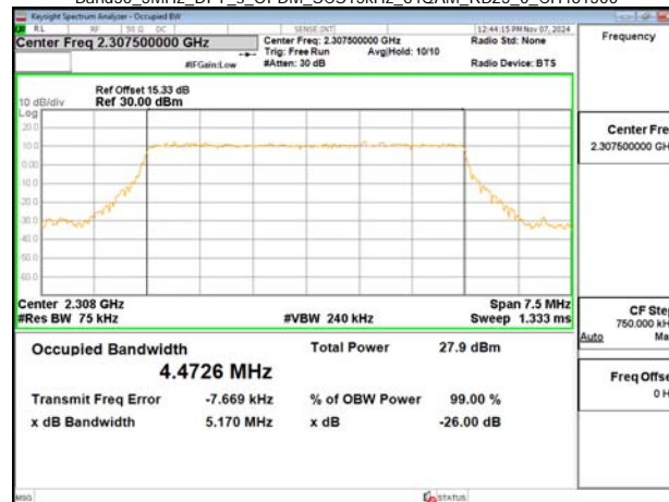
Band30_5MHz_DFT_s_OFDM_SCS15kHz_64QAM_RB25_0_CH461500
