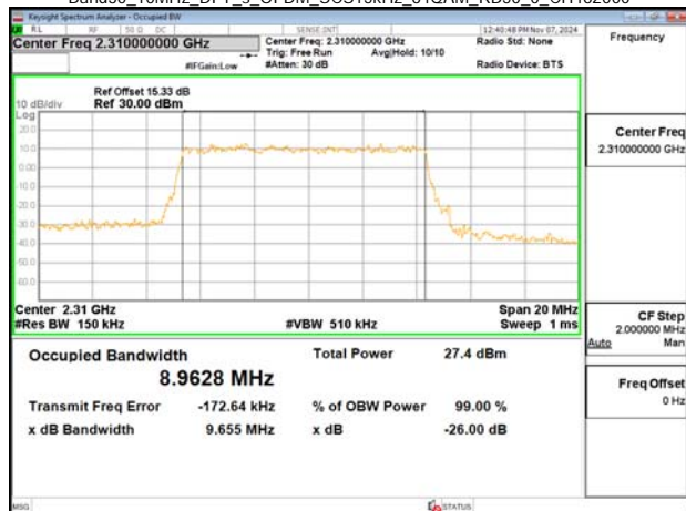
Band30_10MHz_DFT_s_OFDM_SCS15kHz_64QAM_RB50_0_CH462000
