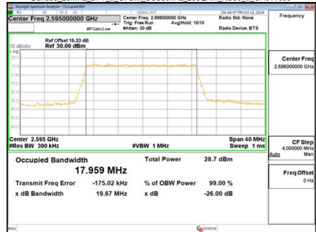
Band38_20MHz_DFT_s_OFDM_SCS30kHz_256QAM_RB50_0_CH519000
