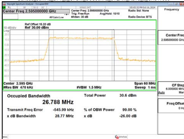
Band38_30MHz_DFT_s_OFDM_SCS30kHz_64QAM_RB75_0_CH519000
