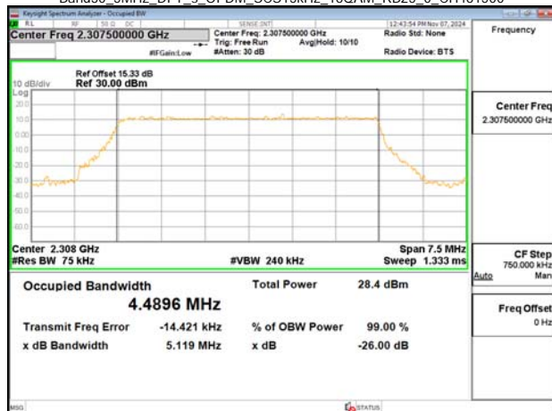
Band30_5MHz_DFT_s_OFDM_SCS15kHz_16QAM_RB25_0_CH461500
