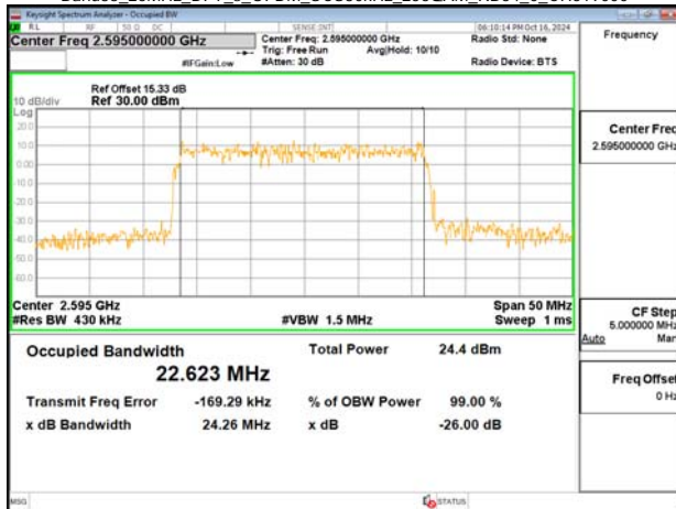
Band38_25MHz_DFT_s_OFDM_SCS30kHz_256QAM_RB64_0_CH519000
