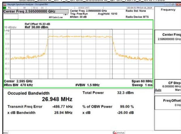
Band38_30MHz_DFT_s_OFDM_SCS30kHz_QPSK_RB75_0_CH519000
