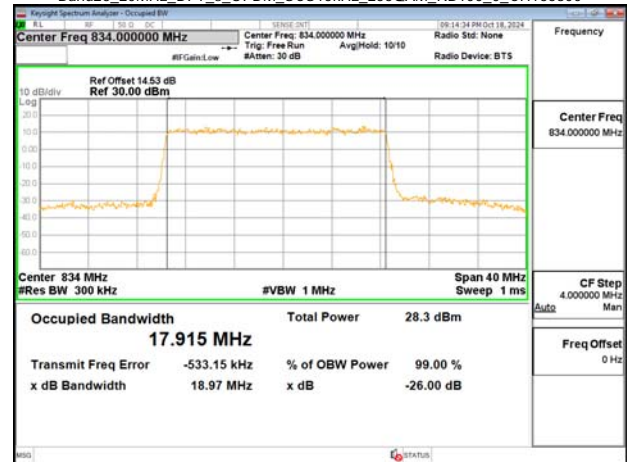
Band26_20MHz_DFT_s_OFDM_SCS15kHz_256QAM_RB100_0_CH166800
