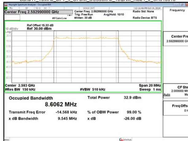
Band41_10MHz_DFT_s_OFDM_SCS30kHz_16QAM_RB24_0_CH518598
