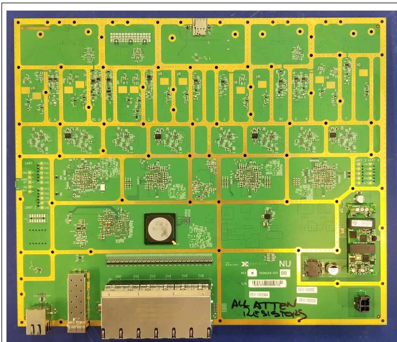
PCB side 2
