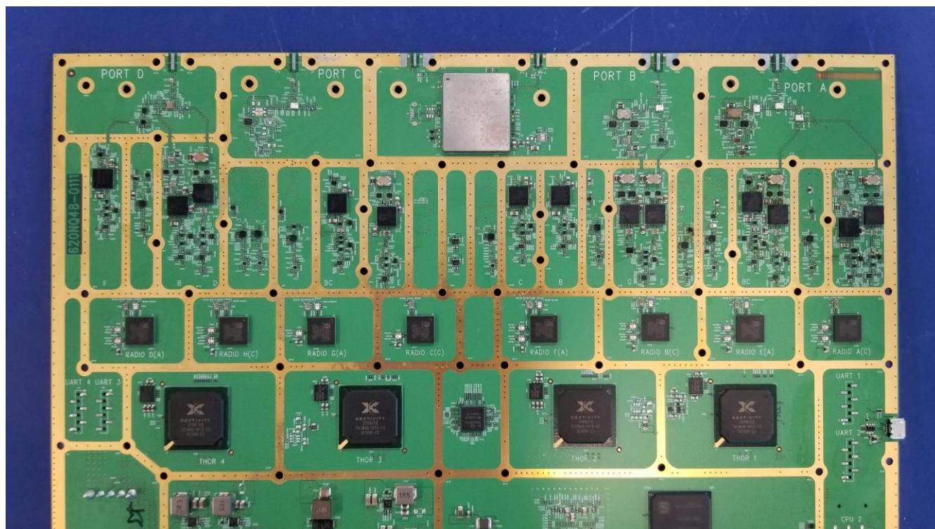
PCB Side 1_Radio
