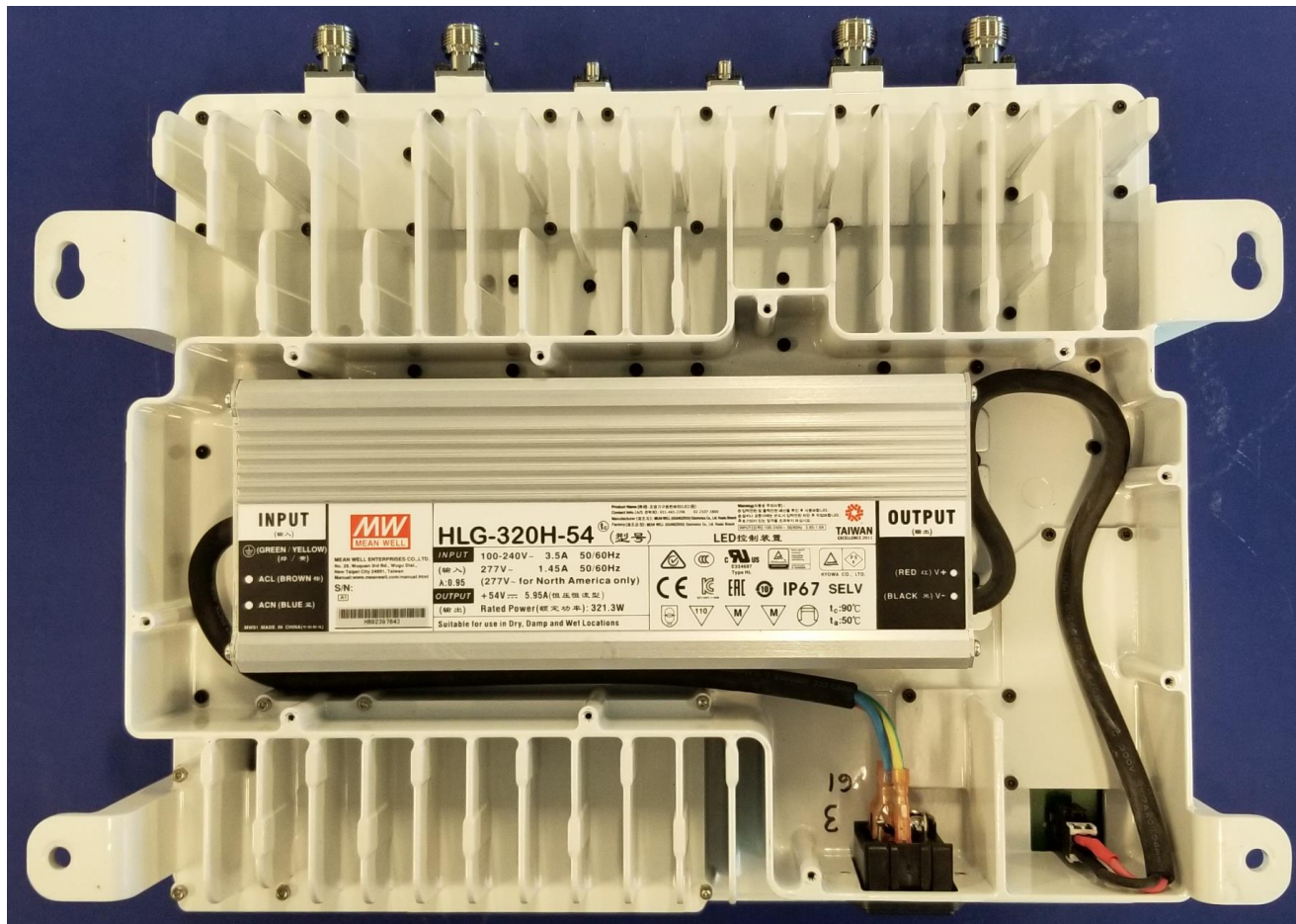
Bottom Cover off
