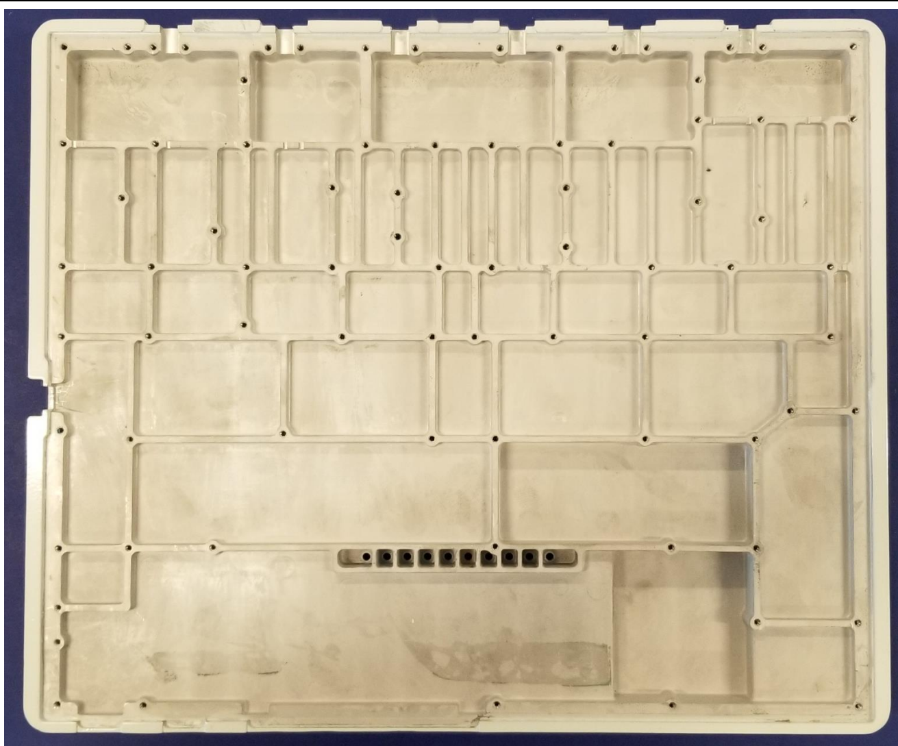
Housing_Top_Internal
