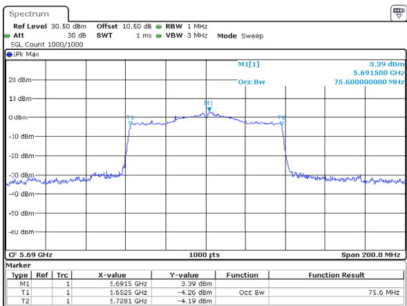
802.11ac80_5690MHz_Chain 1
