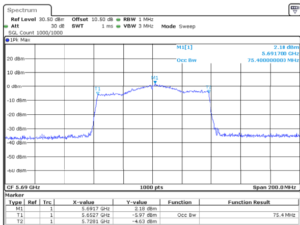
802.11ac80_5690MHz_Chain 2
