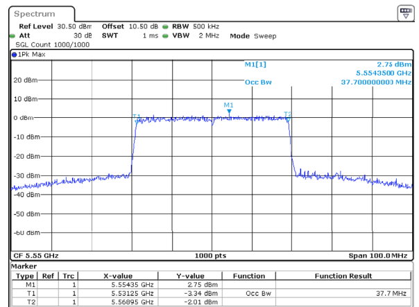
802.11ax40_5550MHz_RU_Full_Chain 1
