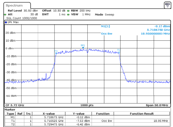
802.11ax20_5720MHz_RU_Full_Chain 2
