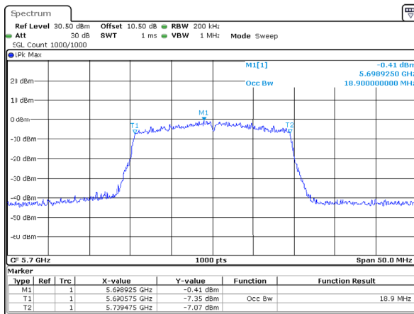
802.11ax20_5700MHz_RU_Full_Chain 2
