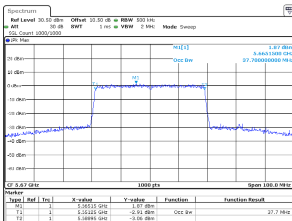
802.11ax40_5670MHz_RU_Full_Chain 1
