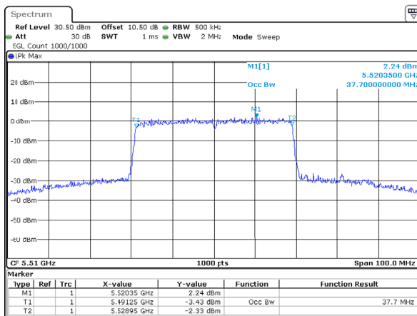
802.11ax40_5510MHz_RU_Full_Chain 1
