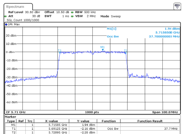
802.11ax40_5710MHz_RU_Full_Chain 1
