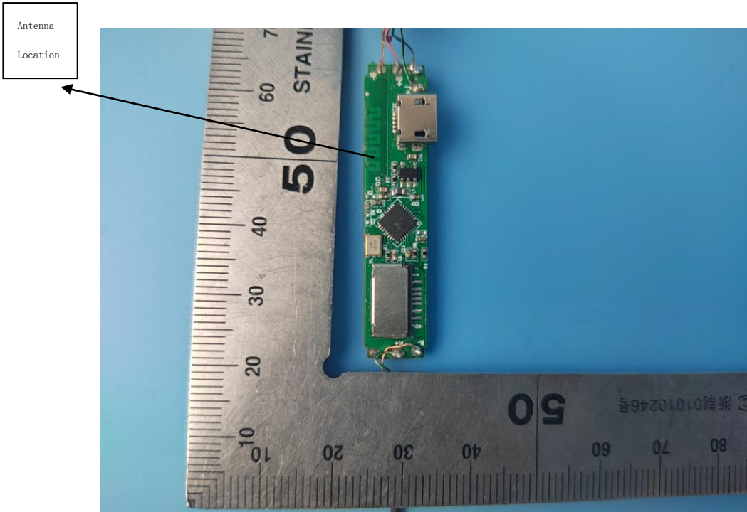
INTERNAL PHOTO OF SAMPLE PCB
