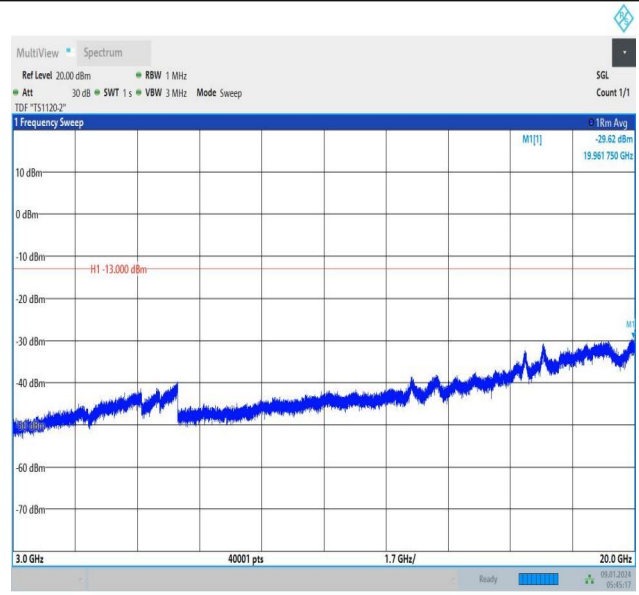
Band66_5MHz_16QAM_131997_1RB#0_3000~20000_3000~20000
