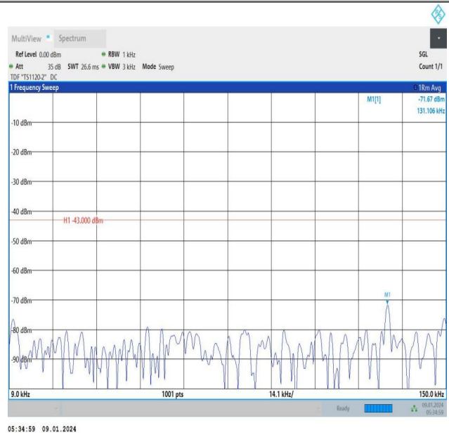
Band66_3MHz_16QAM_131987_15RB#0_0.009~0.15_0.009~0.15
