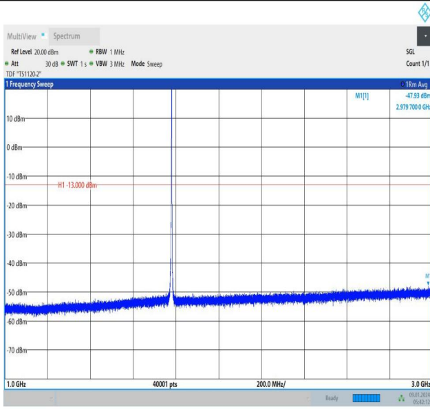
Band66_3MHz_16QAM_132657_1RB#14_1000~3000_1000~3000
