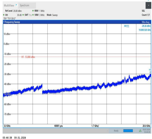
Band66_5MHz_16QAM_131997_1RB#24_3000~20000_3000~20000
