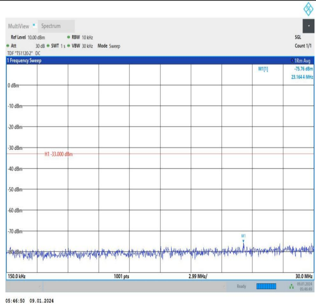
Band66_5MHz_QPSK_131997_25RB#0_0.15~30_0.15~30
