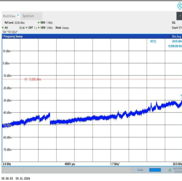
Band66_3MHz_QPSK_131987_15RB#0_3000~20000_3000~20000
