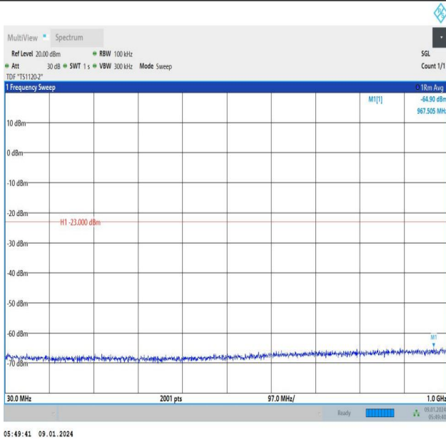
Band66_5MHz_QPSK_132322_1RB#24_30~1000_30~1000
