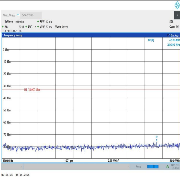
Band66_3MHz_16QAM_131987_15RB#0_0.15~30_0.15~30
