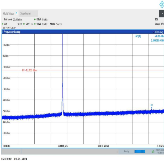
Band66_5MHz_16QAM_132322_1RB#0_1000~3000_1000~3000
