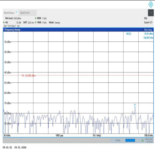
Band66_3MHz_16QAM_132657_1RB#14_0.009~0.15_0.009~0.15
