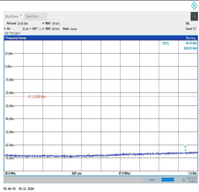
Band66_5MHz_16QAM_132322_1RB#0_30~1000_30~1000
