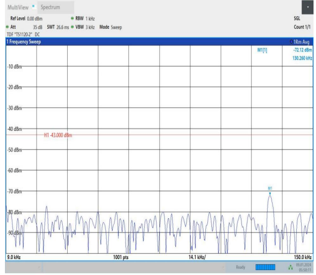
Band66_5MHz_16QAM_132322_1RB#24_0.009~0.15_0.009~0.15
