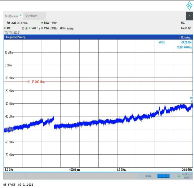
Band66_5MHz_16QAM_131997_25RB#0_3000~20000_3000~20000
