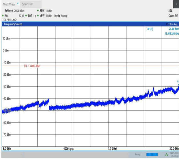
Band66_5MHz_QPSK_132322_1RB#24_3000~20000_3000~20000
