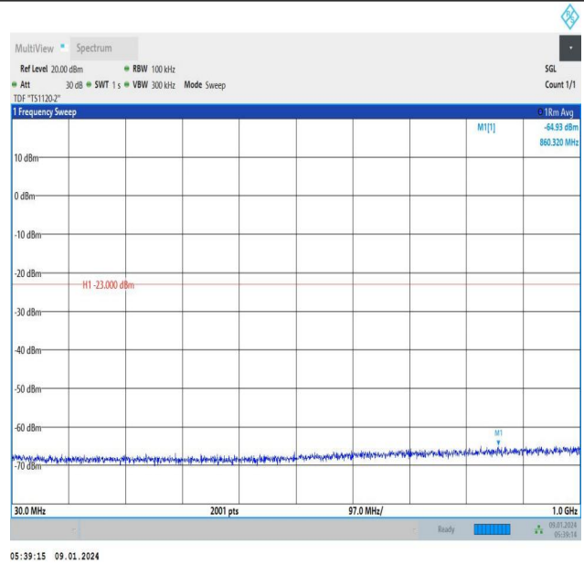
Band66_3MHz_16QAM_132322_15RB#0_30~1000_30~1000
