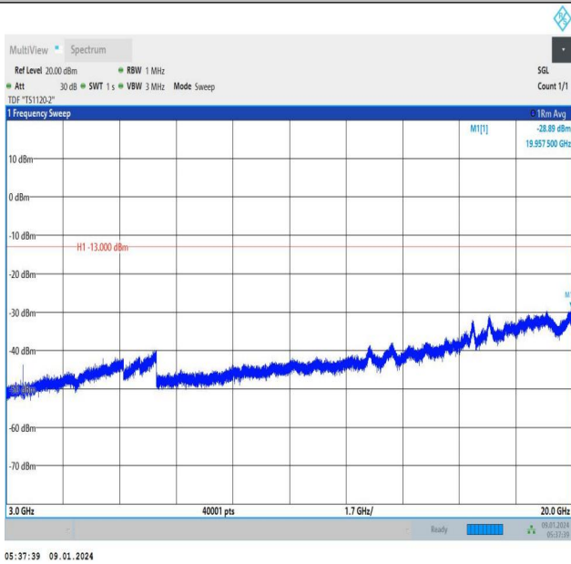
Band66_3MHz_QPSK_132322_1RB#14_3000~20000_3000~20000
