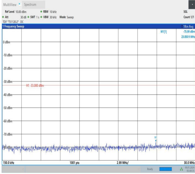
Band66_3MHz_16QAM_132657_1RB#0_0.15~30_0.15~30
