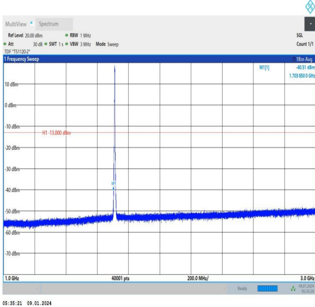
Band66_3MHz_16QAM_131987_15RB#0_1000~3000_1000~3000
