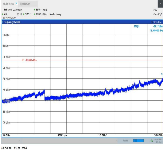
Band66_3MHz_QPSK_132322_1RB#0_3000~20000_3000~20000
