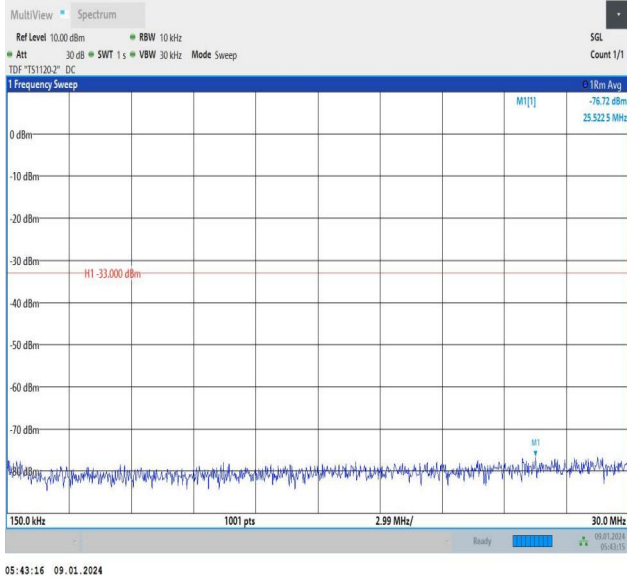
Band66_3MHz_16QAM_132657_15RB#0_0.15~30_0.15~30
