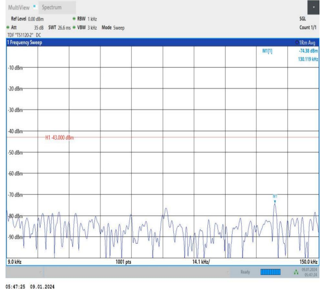
Band66_5MHz_16QAM_131997_25RB#0_0.009~0.15_0.009~0.15
