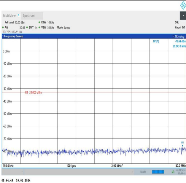
Band66_5MHz_16QAM_131997_1RB#0_0.15~30_0.15~30
