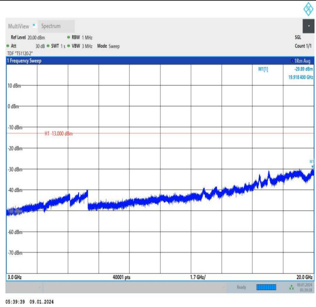
Band66_3MHz_16QAM_132322_15RB#0_3000~20000_3000~20000
