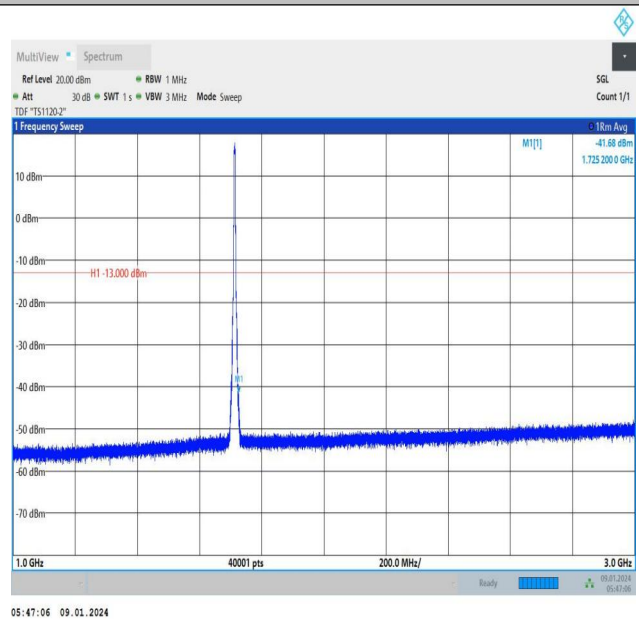
Band66_5MHz_QPSK_131997_25RB#0_1000~3000_1000~3000
