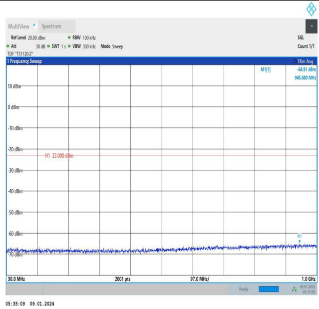
Band66_3MHz_16QAM_131987_15RB#0_30~1000_30~1000
