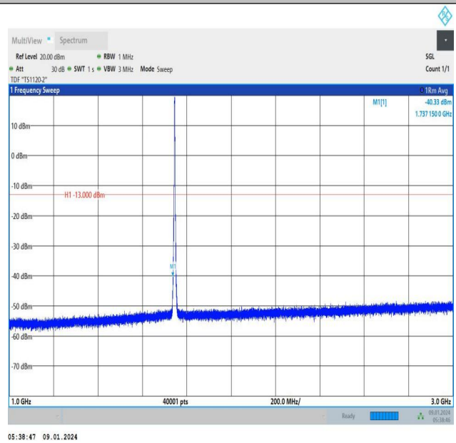
Band66_3MHz_QPSK_132322_15RB#0_1000~3000_1000~3000
