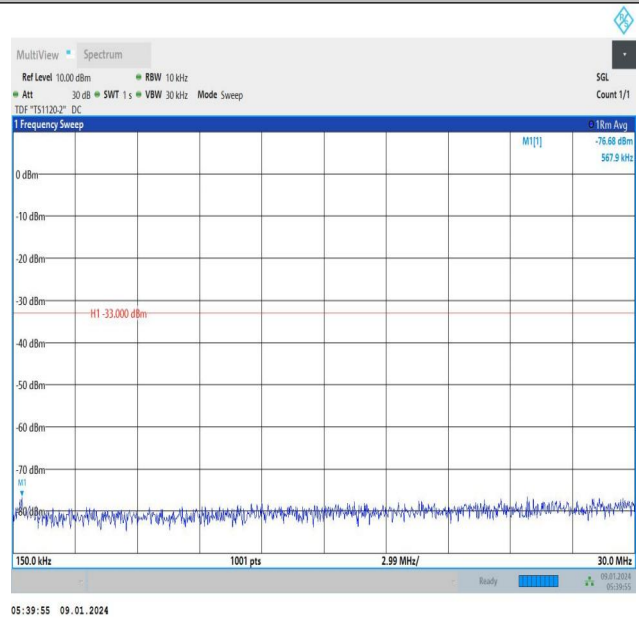
Band66_3MHz_QPSK_132657_1RB#0_0.15~30_0.15~30
