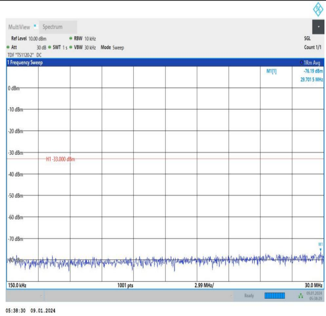
Band66_3MHz_QPSK_132322_15RB#0_0.15~30_0.15~30
