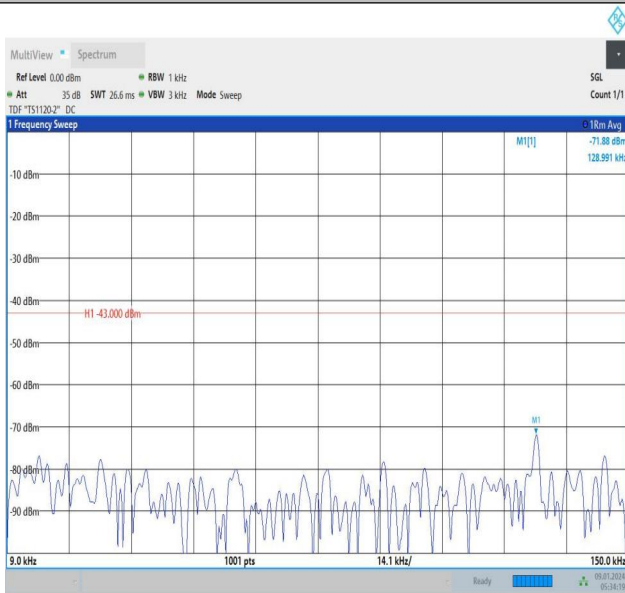
Band66_3MHz_16QAM_131987_1RB#14_1000~3000_1000~3000
