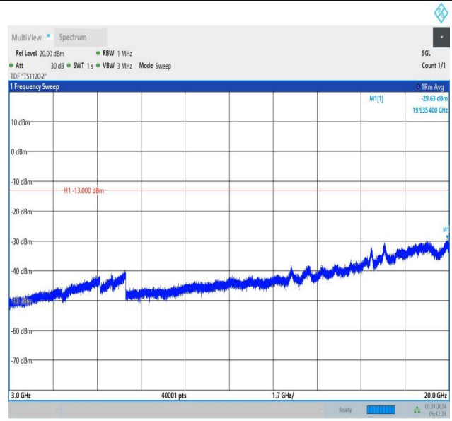
Band66_3MHz_16QAM_132657_1RB#14_3000~20000_3000~20000
