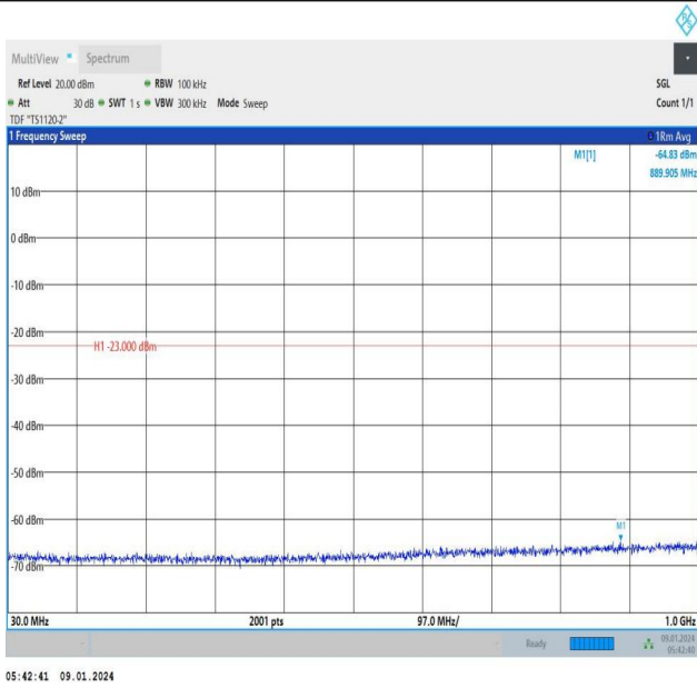
Band66_3MHz_QPSK_132657_15RB#0_30~1000_30~1000
