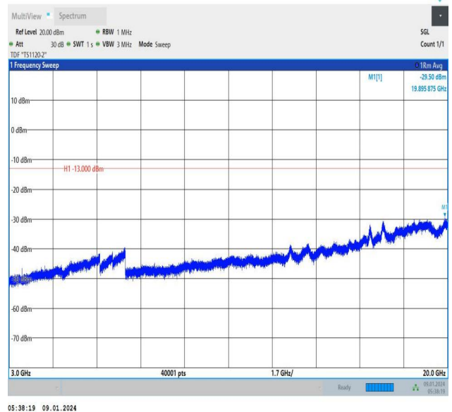
Band66_3MHz_16QAM_132322_1RB#14_3000~20000_3000~20000
