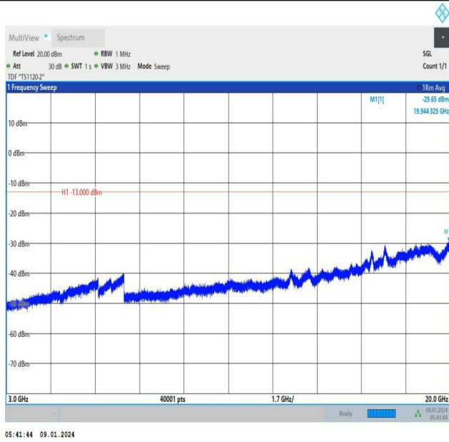
Band66_3MHz_QPSK_132657_1RB#14_3000~20000_3000~20000
