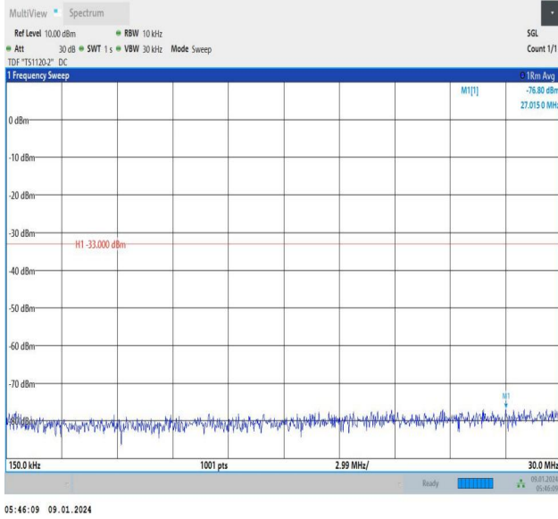
Band66_5MHz_16QAM_131997_1RB#24_0.15~30_0.15~30
