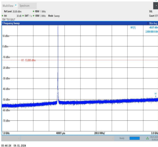
Band66_5MHz_16QAM_131997_1RB#24_1000~3000_1000~3000
