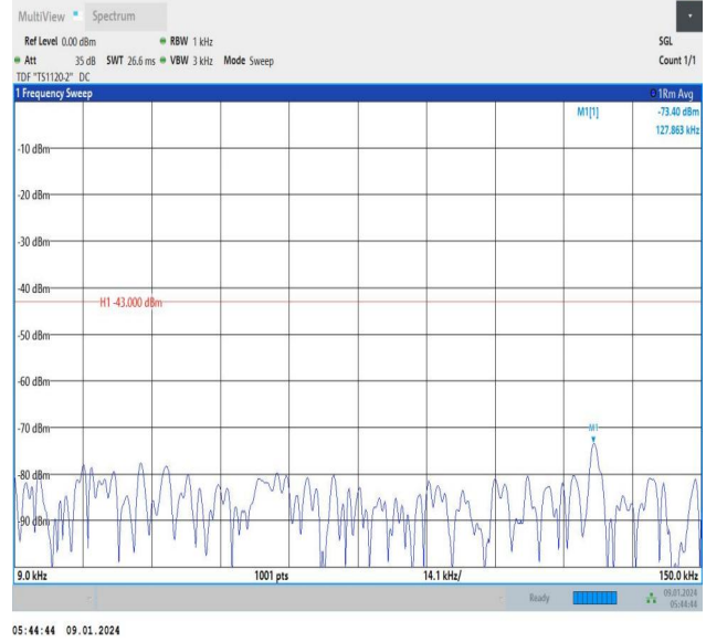
Band66_5MHz_16QAM_131997_1RB#0_0.009~0.15_0.009~0.15
