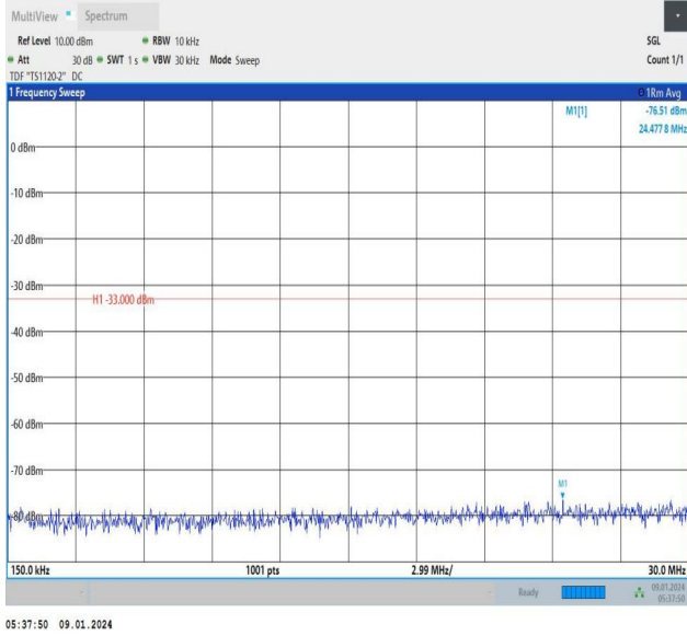
Band66_3MHz_16QAM_132322_1RB#14_0.15~30_0.15~30
