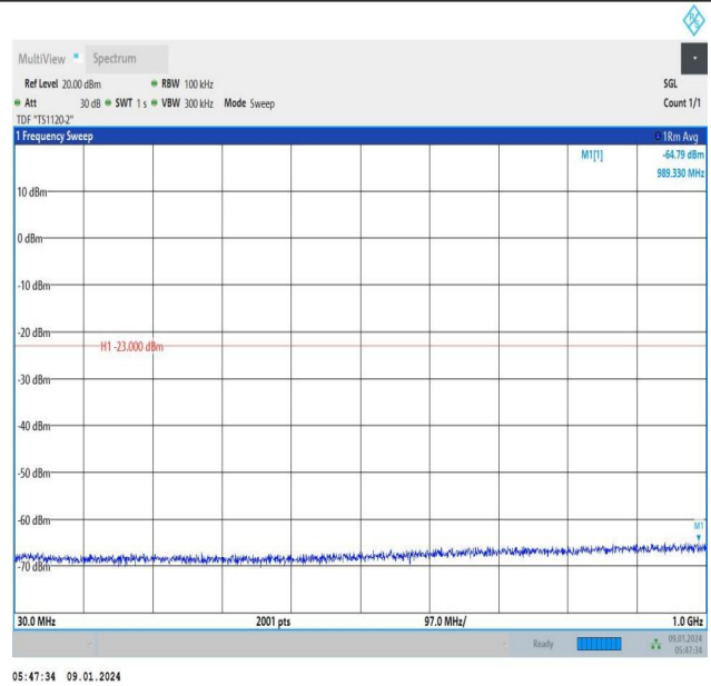
Band66_5MHz_16QAM_131997_25RB#0_30~1000_30~1000
