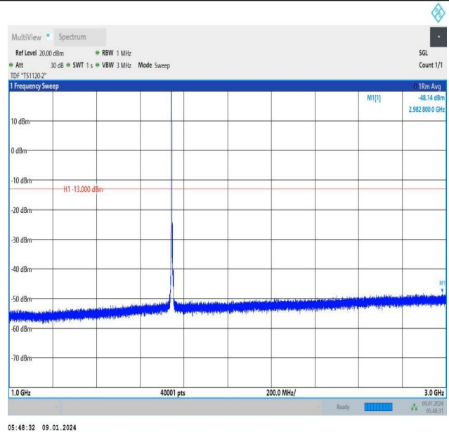
Band66_5MHz_QPSK_132322_1RB#0_1000~3000_1000~30 00
