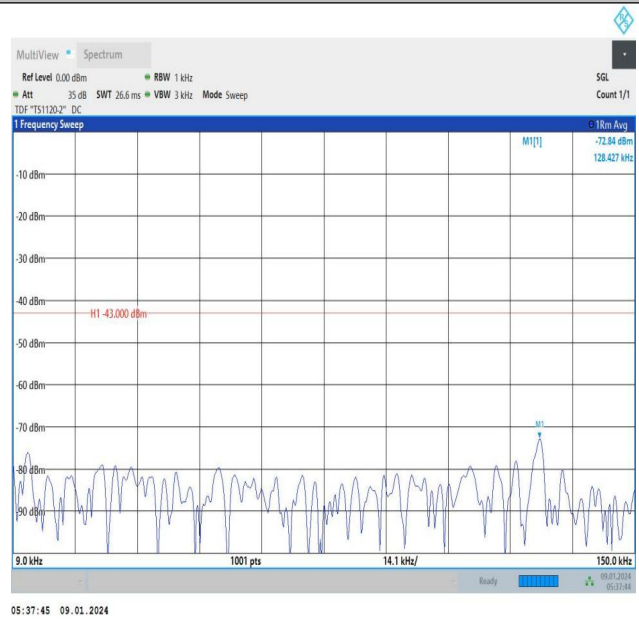
Band66_3MHz_16QAM_132322_1RB#14_0.009~0.15_0.009~0.15
