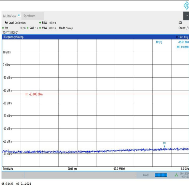
Band66_3MHz_QPSK_131987_15RB#0_30~1000_30~1000
