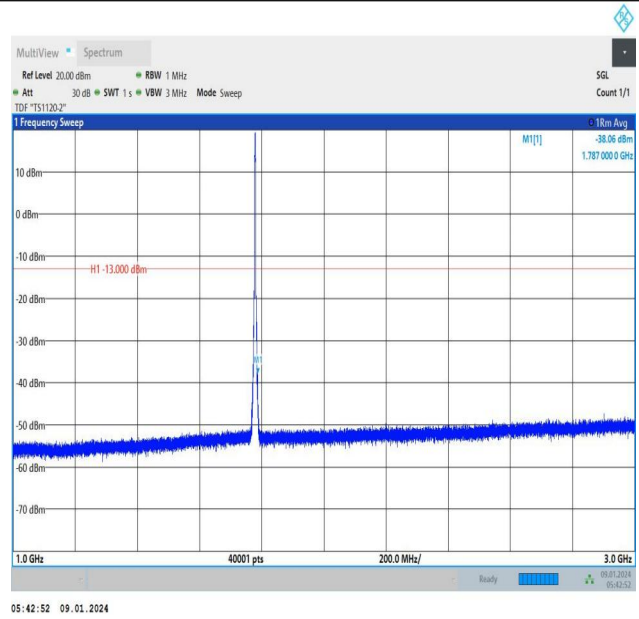
Band66_3MHz_QPSK_132657_15RB#0_1000~3000_1000~3000
