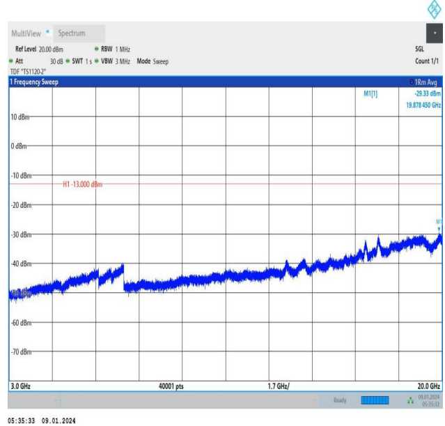
Band66_3MHz_16QAM_131987_15RB#0_3000~20000_3000~20000
