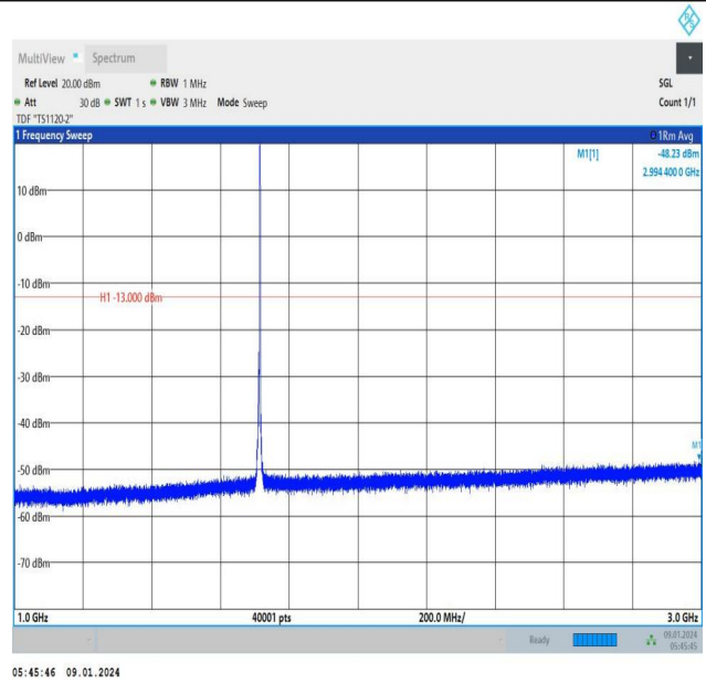
Band66_5MHz_QPSK_131997_1RB#24_1000~3000_1000~3000
