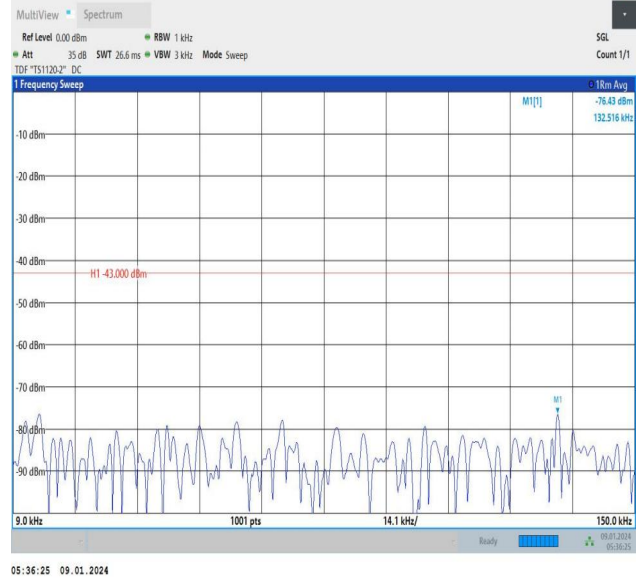
Band66_3MHz_16QAM_132322_1RB#0_0.009~0.15_0.009~0.15
