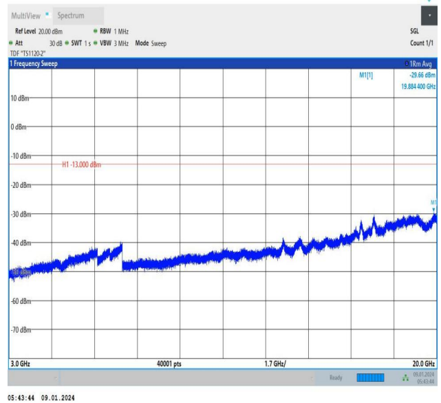
Band66_3MHz_16QAM_132657_15RB#0_3000~20000_3000~20000
