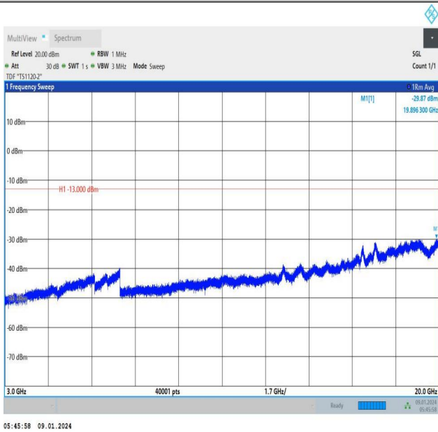
Band66_5MHz_QPSK_131997_1RB#24_3000~20000_3000~20000
