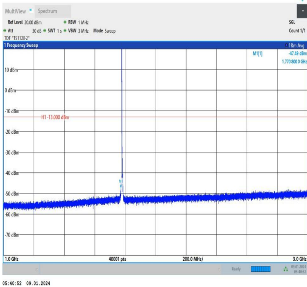
Band66_3MHz_16QAM_132657_1RB#0_1000~3000_1000~3000
