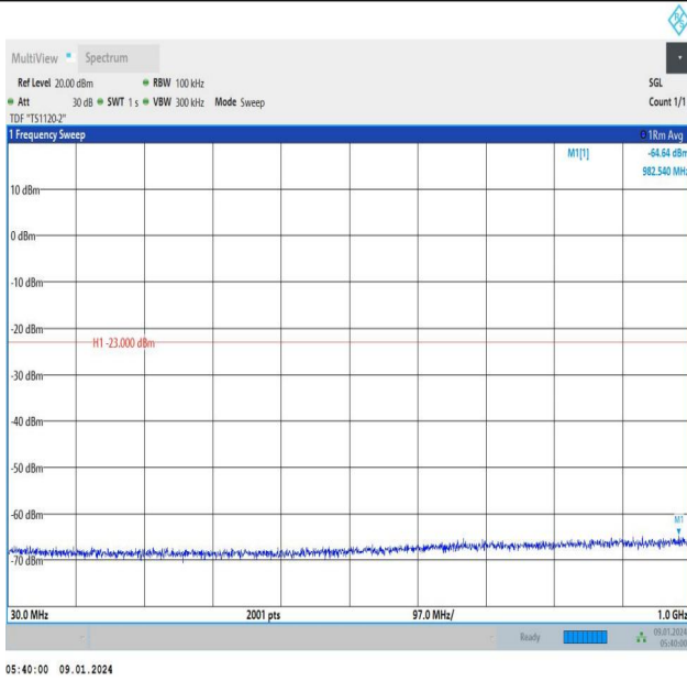
Band66_3MHz_QPSK_132657_1RB#0_30~1000_30~1000
