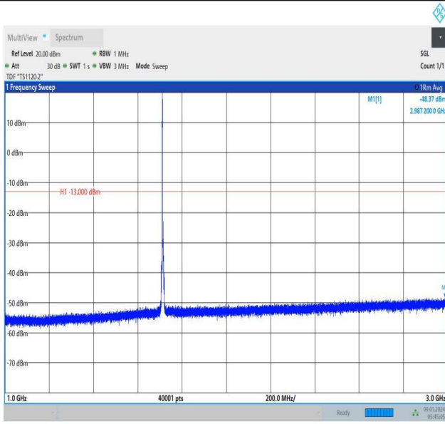
Band66_5MHz_16QAM_131997_1RB#0_1000~3000_1000~3000
