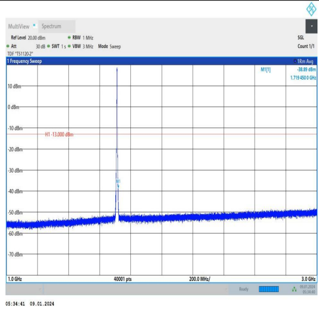
Band66_3MHz_QPSK_131987_15RB#0_1000~3000_1000~3000
