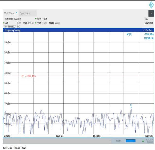
Band66_5MHz_16QAM_131997_1RB#24_0.009~0.15_0.009~0.15
