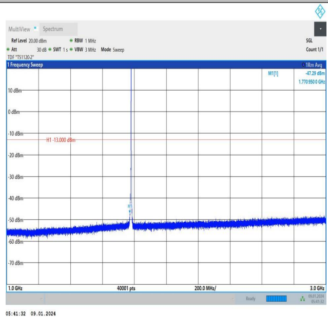
Band66_3MHz_QPSK_132657_1RB#14_1000~3000_1000~3000
