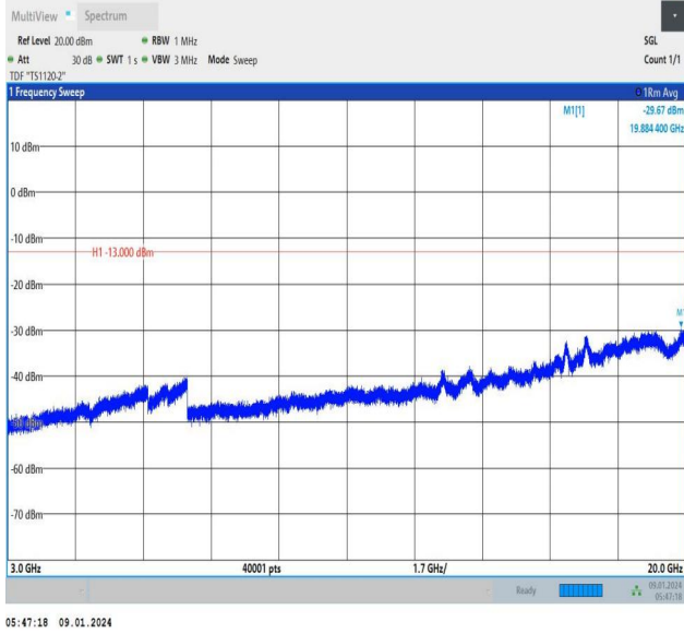
Band66_5MHz_QPSK_131997_25RB#0_3000~20000_3000~20000
