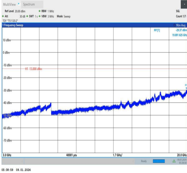
Band66_3MHz_QPSK_132322_15RB#0_3000~20000_3000~20000
