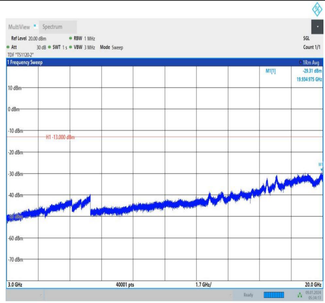
Band66_3MHz_16QAM_131987_1RB#14_3000~20000_3000~20000
