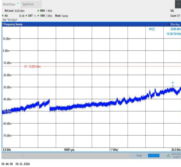
Band66_5MHz_QPSK_131997_1RB#0_3000~20000_3000~20000
