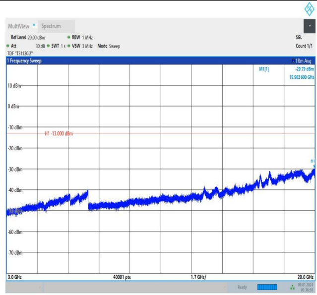
Band66_3MHz_16QAM_132322_1RB#0_3000~20000_3000~20000
