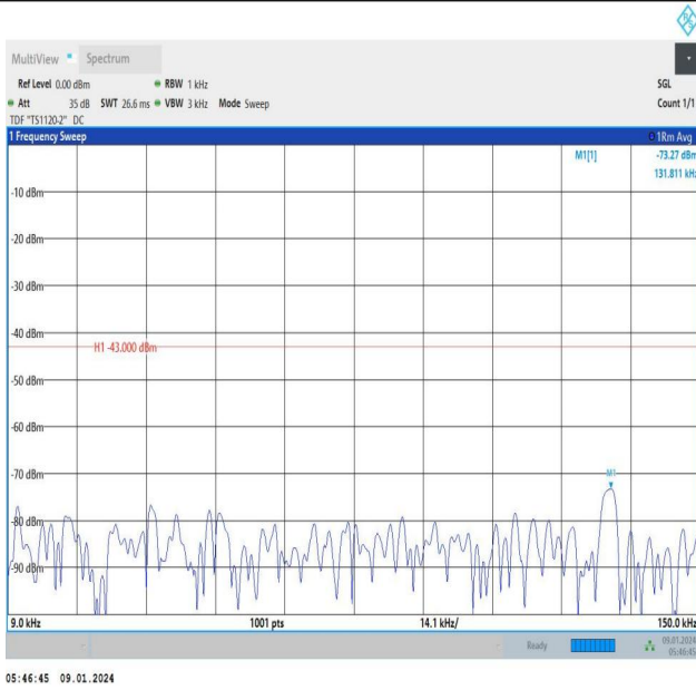
Band66_5MHz_QPSK_131997_25RB#0_0.009~0.15_0.009~0.15
