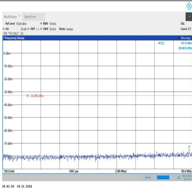
Band66_3MHz_16QAM_132657_1RB#14_0.15~30_0.15~30
