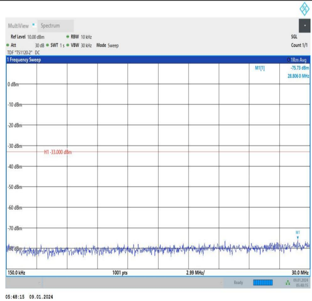
Band66_5MHz_QPSK_132322_1RB#0_0.15~30_0.15~30
