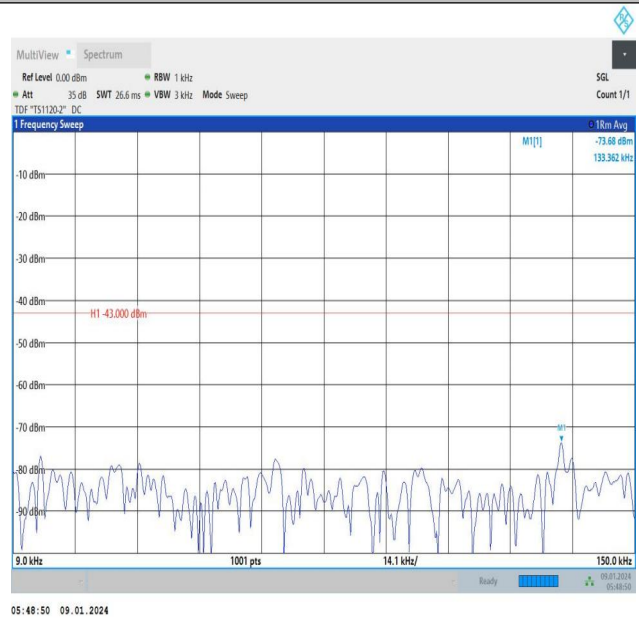
Band66_5MHz_16QAM_132322_1RB#0_0.009~0.15_0.009~0 .15
