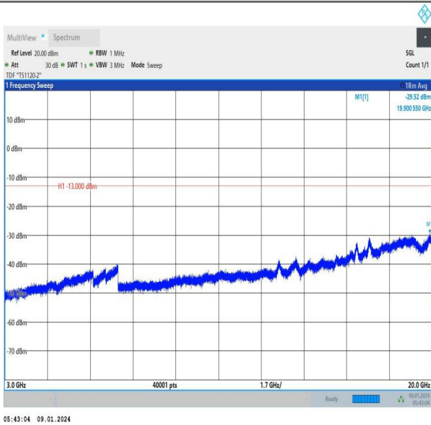
Band66_3MHz_QPSK_132657_15RB#0_3000~20000_3000~20000
