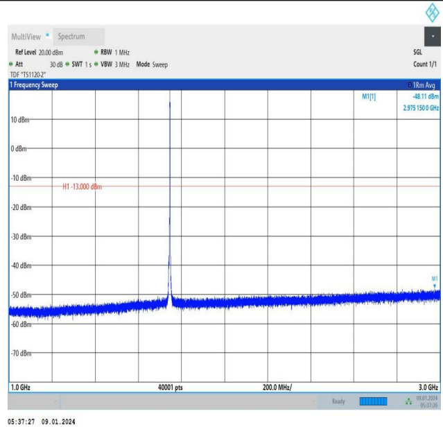
Band66_3MHz_QPSK_132322_1RB#14_1000~3000_1000~3000
