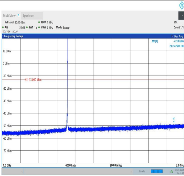
Band66_3MHz_16QAM_131987_1RB#14_1000~3000_1000~3000
