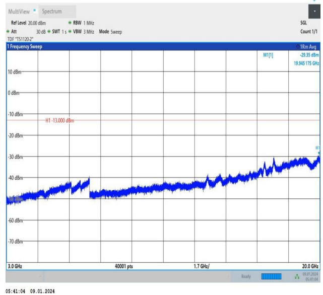
Band66_3MHz_16QAM_132657_1RB#0_3000~20000_3000~20000
