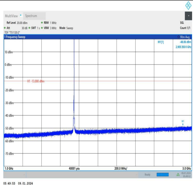
Band66_5MHz_QPSK_132322_1RB#24_1000~3000_1000~3000
