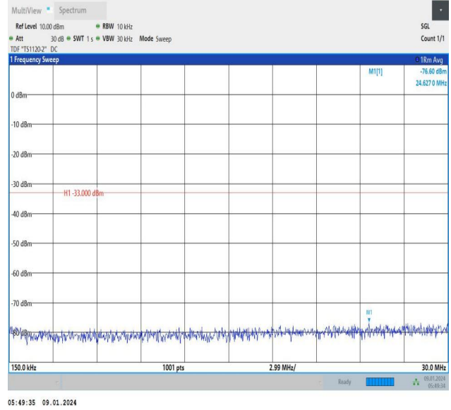
Band66_5MHz_QPSK_132322_1RB#24_0.15~30_0.15~30
