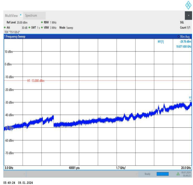
Band66_5MHz_16QAM_132322_1RB#0_3000~20000_3000~20000
