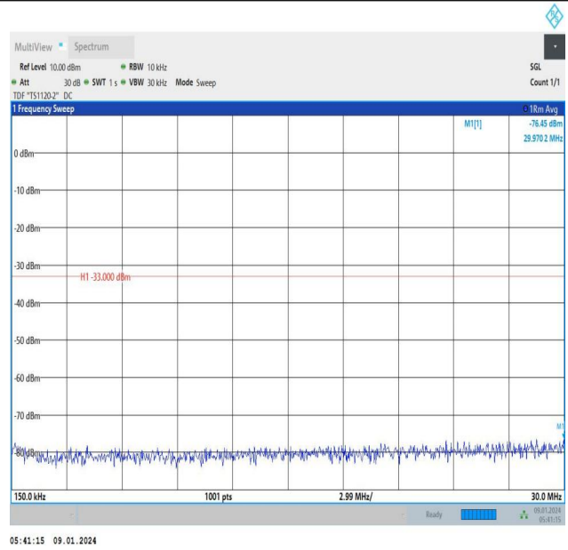
Band66_3MHz_QPSK_132657_1RB#14_0.15~30_0.15~30
