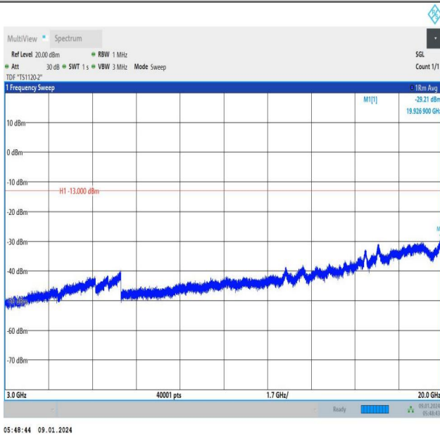
Band66_5MHz_QPSK_132322_1RB#0_3000~20000_3000~2 0000
