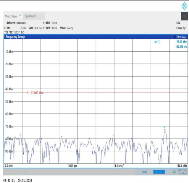
Band66_3MHz_16QAM_132657_15RB#0_0.009~0.15_0.009~0.15
