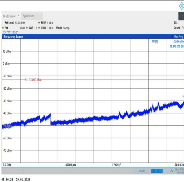
Band66_3MHz_QPSK_132657_1RB#0_3000~20000_3000~2 0000
