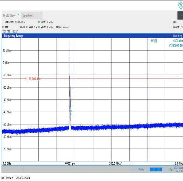
Band66_3MHz_16QAM_132322_15RB#0_1000~3000_1000~3000
