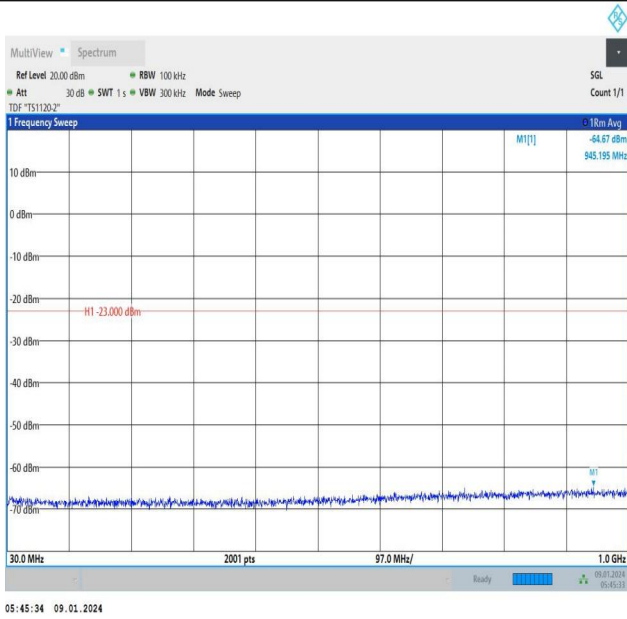
Band66_5MHz_QPSK_131997_1RB#24_30~1000_30~1000
