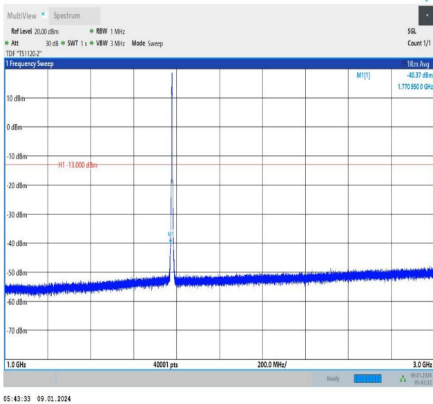
Band66_3MHz_16QAM_132657_15RB#0_1000~3000_1000~3000
