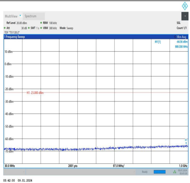
Band66_3MHz_16QAM_132657_1RB#14_30~1000_30~1000
