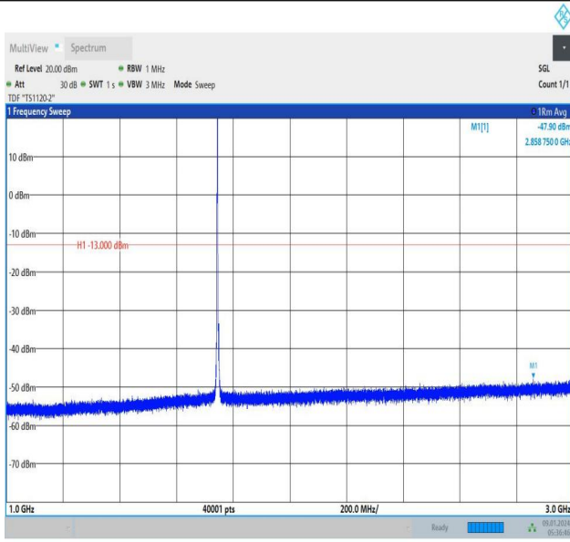
Band66_3MHz_16QAM_132322_1RB#0_1000~3000_1000~3000
