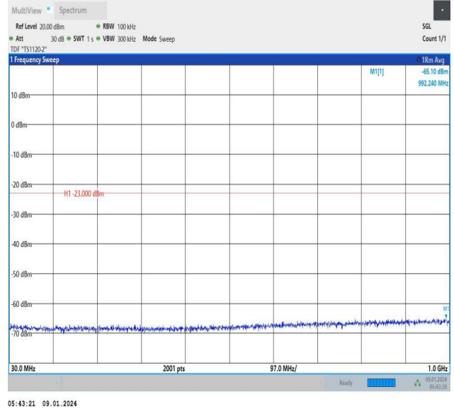
Band66_3MHz_16QAM_132657_15RB#0_30~1000_30~1000
