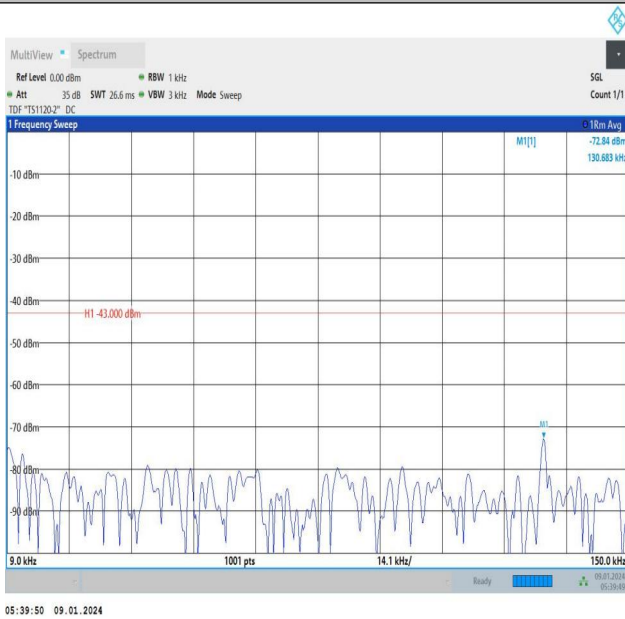
Band66_3MHz_QPSK_132657_1RB#0_0.009~0.15_0.009~0.15
