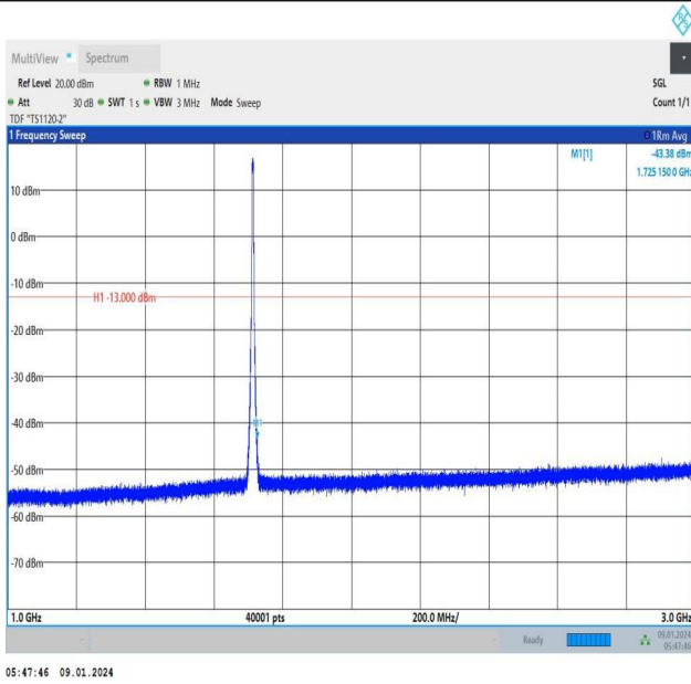
Band66_5MHz_16QAM_131997_25RB#0_1000~3000_1000~3000
