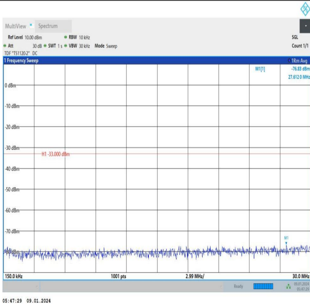
Band66_5MHz_16QAM_131997_25RB#0_0.15~30_0.15~30
