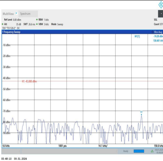
Band66_5MHz_QPSK_132322_1RB#0_0.009~0.15_0.009~0.15
