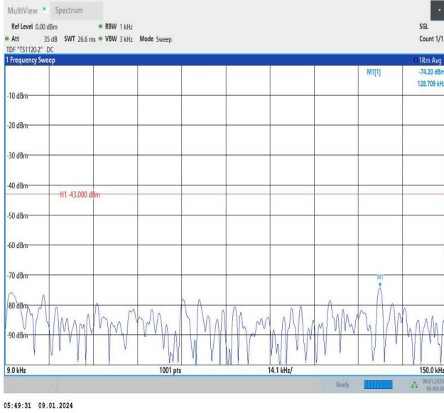
Band66_5MHz_QPSK_132322_1RB#24_0.009~0.15_0.009~0.15
