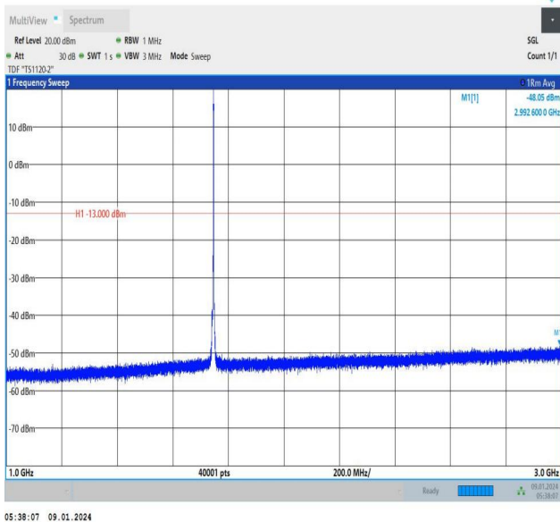
Band66_3MHz_16QAM_132322_1RB#14_1000~3000_1000~3000
