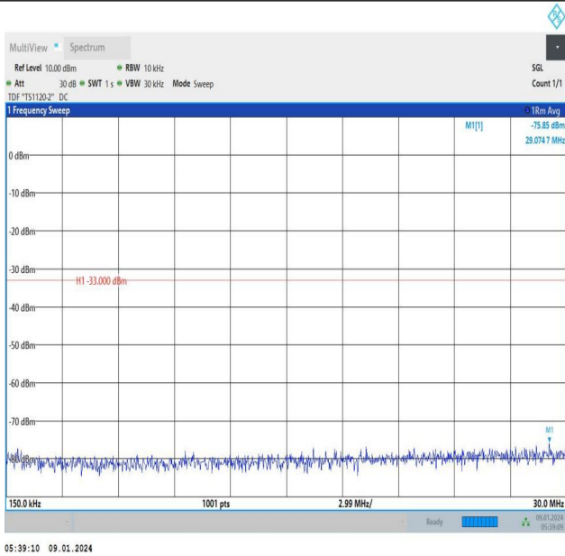
Band66_3MHz_16QAM_132322_15RB#0_0.15~30_0.15~30
