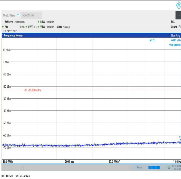
Band66_5MHz_QPSK_132322_1RB#0_30~1000_30~1000
