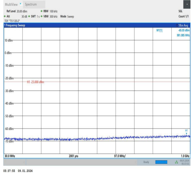
Band66_3MHz_16QAM_132322_1RB#14_30~1000_30~1000
