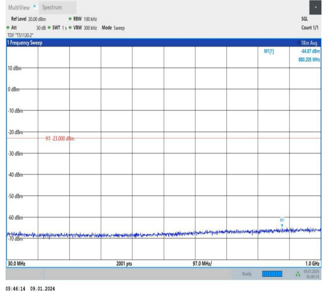
Band66_5MHz_16QAM_131997_1RB#24_30~1000_30~1000
