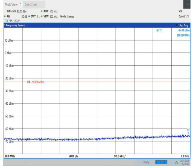
Band66_3MHz_16QAM_132657_1RB#0_30~1000_30~1000
