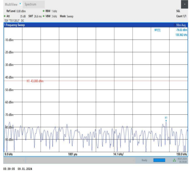
Band66_3MHz_16QAM_132322_15RB#0_0.009~0.15_0.009~0.15
