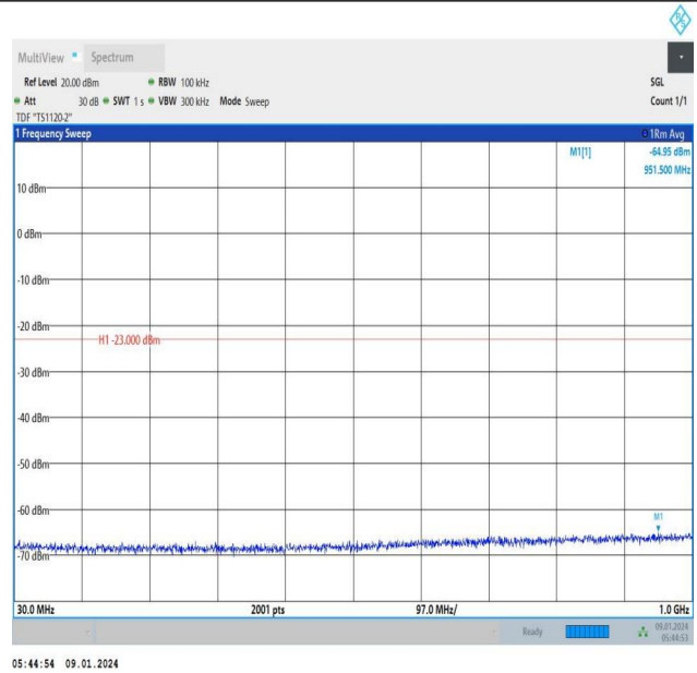
Band66_5MHz_16QAM_131997_1RB#0_30~1000_30~1000
