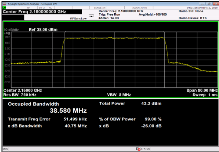
Figure 717: 256QAM 40MHz B.W.; 2160.0MHz, 15kHz - Output
