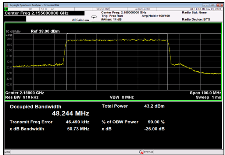
Figure 726: 256QAM 50MHz B.W.; 2155.0MHz, 15kHz - Output
