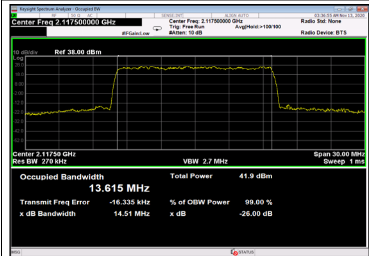
Figure 685: 256QAM 15MHz B.W.; 2117.5MHz, 30kHz - Output
