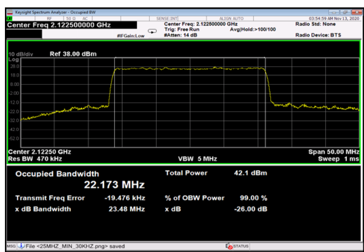
Figure 704: 256QAM 25MHz B.W.; 2122.5MHz, 60kHz - Output
