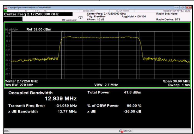
Figure 692: 256QAM 15MHz B.W.; 2172.5MHz, 60kHz - Output
