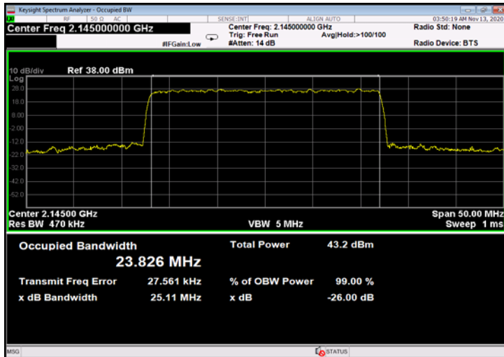
Figure 705: 256QAM 25MHz B.W.; 2145.0MHz, 15kHz - Output
