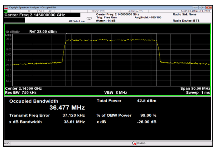
Figure 716: 256QAM 40MHz B.W.; 2145.0MHz, 60kHz - Output
