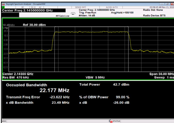
Figure 707: 256QAM 25MHz B.W.; 2145.0MHz, 60kHz - Output
