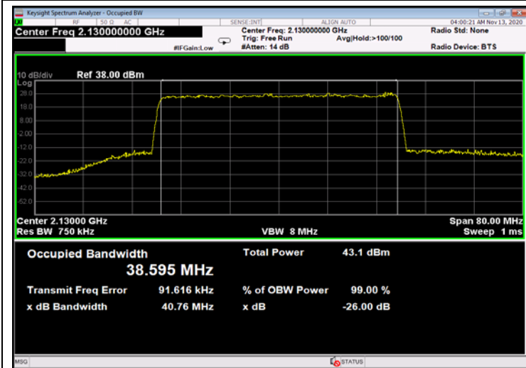
Figure 711: 256QAM 40MHz B.W.; 2130.0MHz, 15kHz - Output
