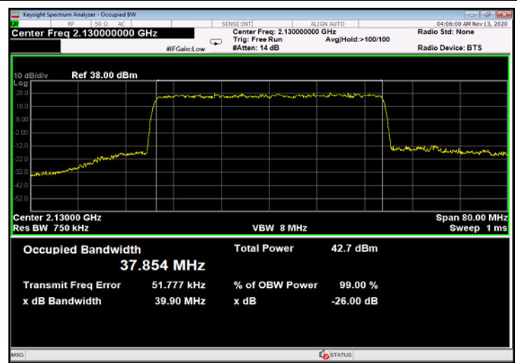
Figure 712: 256QAM 40MHz B.W.; 2130.0MHz, 30kHz - Output
