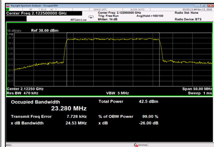
Figure 703: 256QAM 25MHz B.W.; 2122.5MHz, 30kHz - Output
