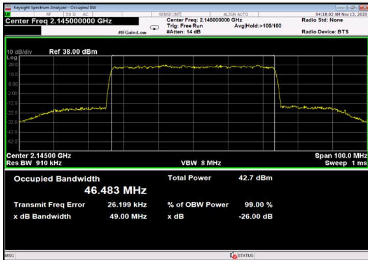
Figure 725: 256QAM 50MHz B.W.; 2145.0MHz, 60kHz - Output
