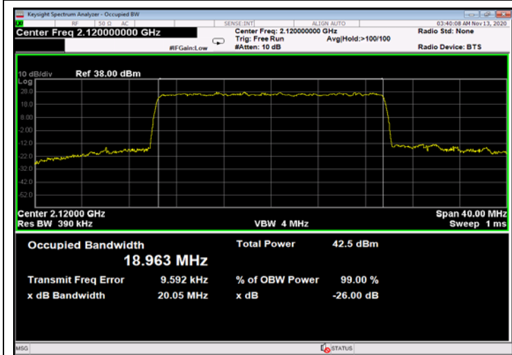
Figure 693: 256QAM 20MHz B.W.; 2120.0MHz, 15kHz - Output
