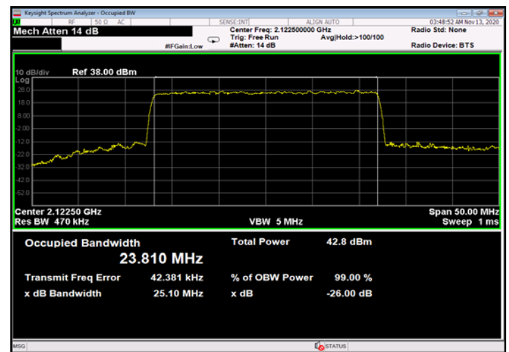
Figure 702: 256QAM 25MHz B.W.; 2122.5MHz, 15kHz - Output
