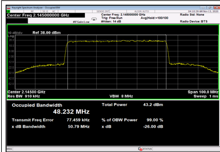
Figure 723: 256QAM 50MHz B.W.; 2145.0MHz, 15kHz - Output
