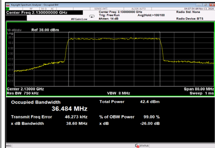
Figure 713: 256QAM 40MHz B.W.; 2130.0MHz, 60kHz - Output
