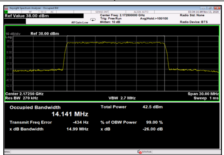
Figure 690: 256QAM 15MHz B.W.; 2172.5MHz, 15kHz - Output
