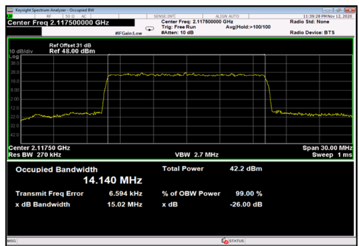
Figure 750: QPSK 15MHz B.W.; 2117.5MHz, 15kHz - Output
