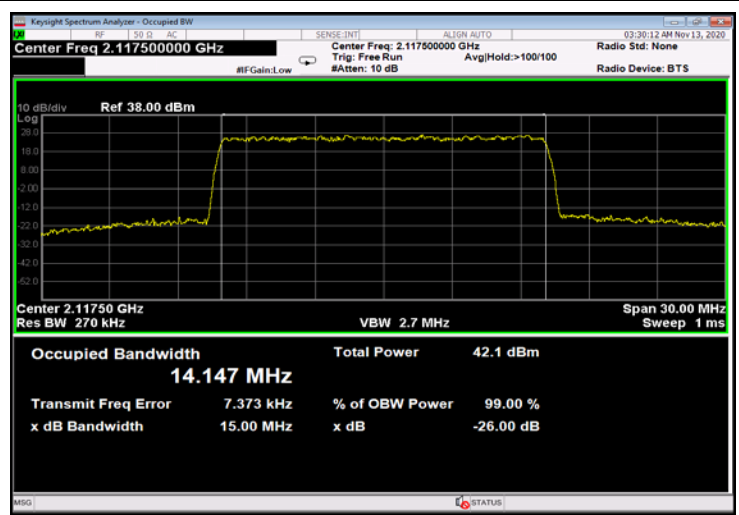
Figure 684: 256QAM 15MHz B.W.; 2117.5MHz, 15kHz - Output
