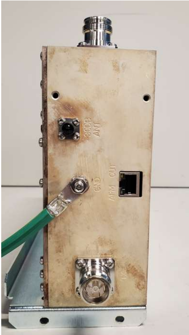
Site TX Filter
