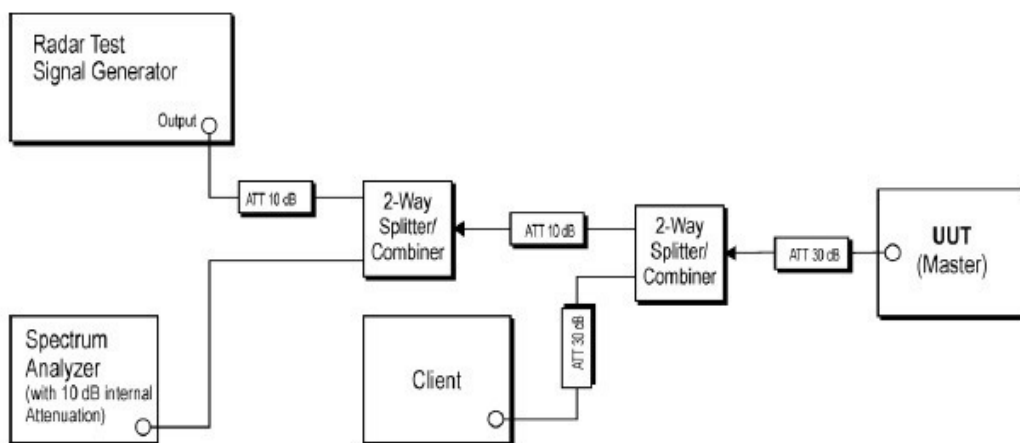
DFS master
