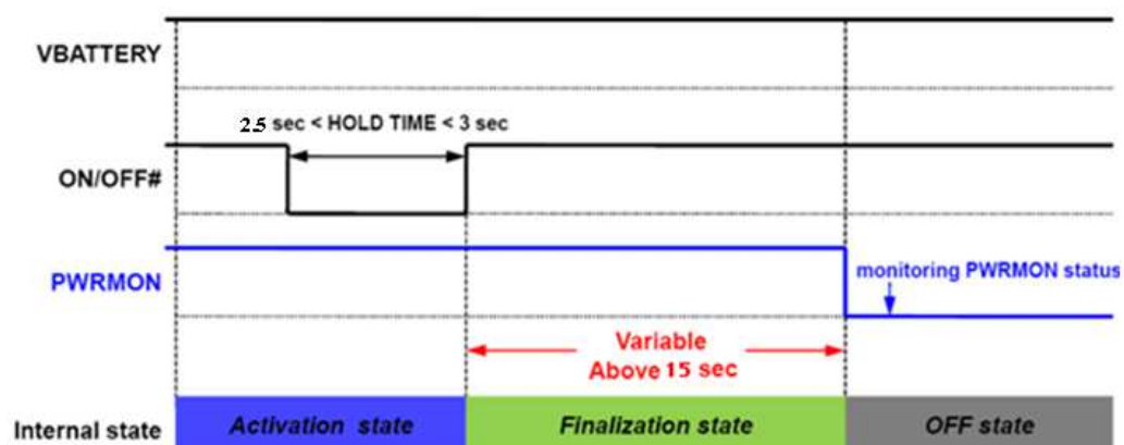
Figure 7: Hardware Shutdown
