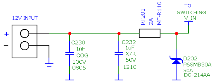
Figure 11: Example of Switching Regulator with 12V Input – Part 1
