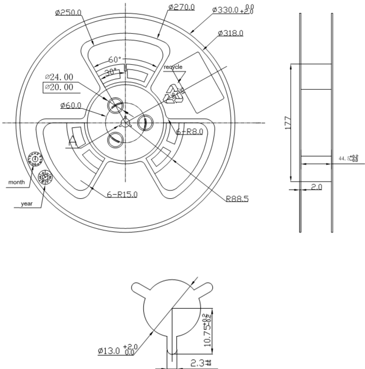
Figure 33: Reel Detail
