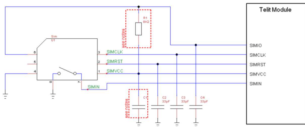
Figure 28: SIM Schematics
