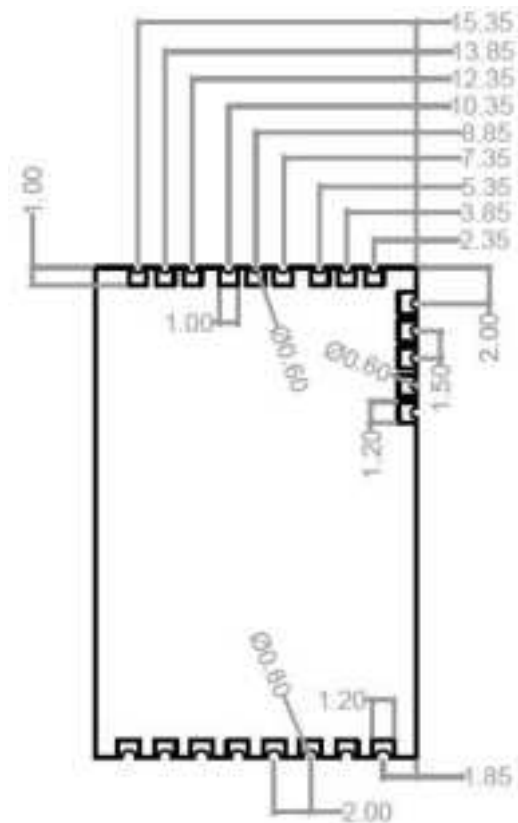
Bottom View
