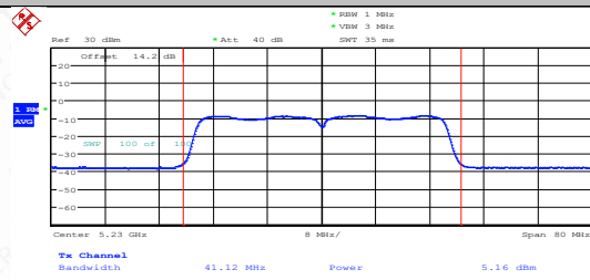
11AC40SISO-Ant1-5230-PASS
