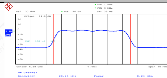
11N20MIMO-Ant2-5580-PASS
