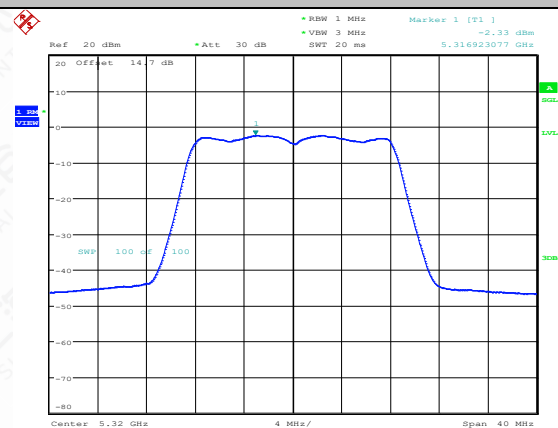
11A-Ant1-5320-PASS
