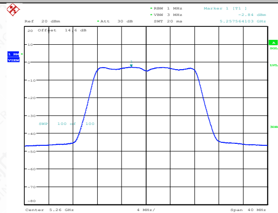
11A-CDD-Ant1-5260-PASS
