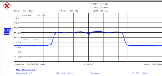
11AC40MIMO-Ant1-5310-PASS
