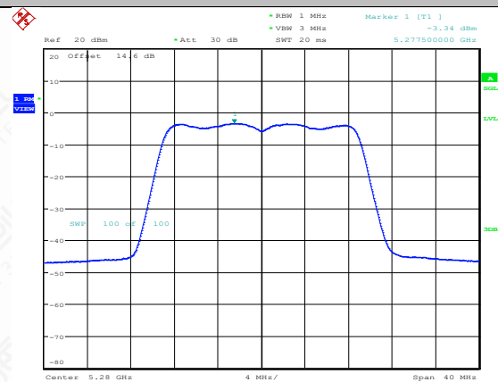
11N20SISO-Ant1-5280-PASS
