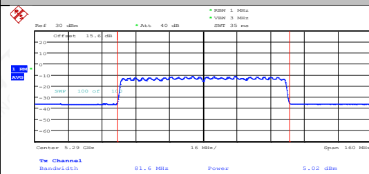
11AX80MIMO-Ant2-5290-PASS
