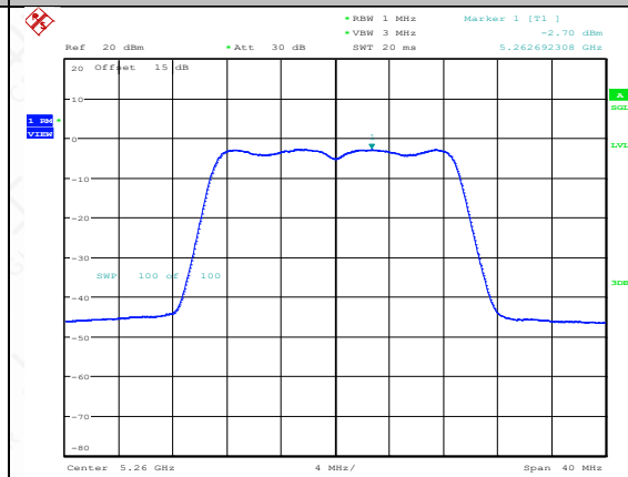
11N20MIMO-Ant2-5260-PASS
