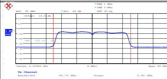
11AC40SISO-Ant2-5230-PASS
