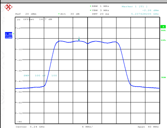
11N20MIMO-Ant2-5240-PASS
