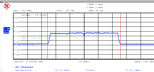
11AC80MIMO-Ant1-5530-PASS
