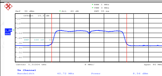
11N40MIMO-Ant2-5310-PASS
