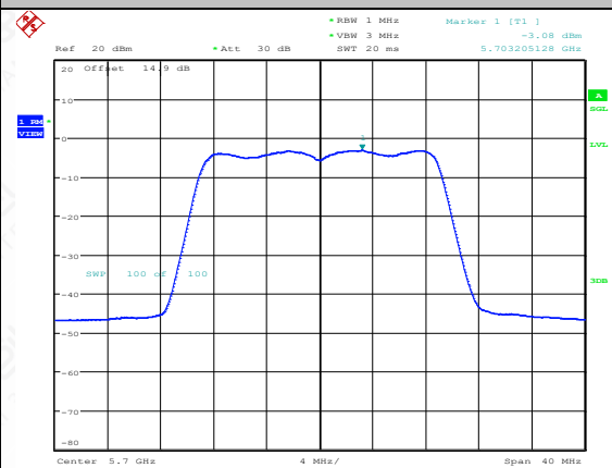
11N20SISO-Ant2-5700-PASS
