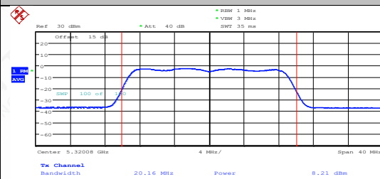
11AC20MIMO-Ant2-5320-PASS
