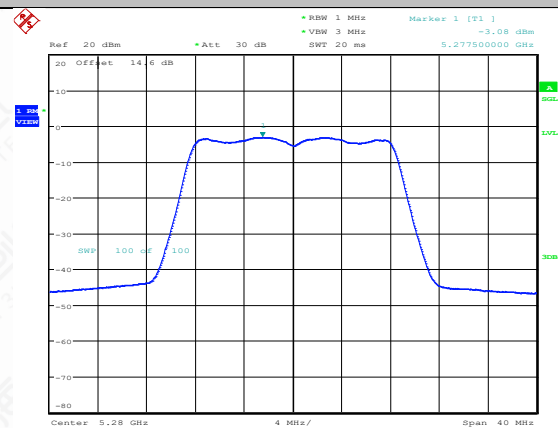
11A-Ant1-5280-PASS
