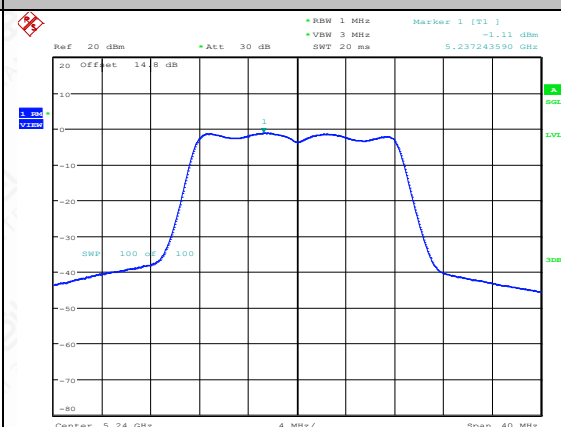
11A-CDD-Ant2-5240-PASS
