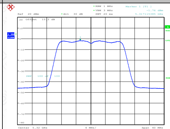
11N20MIMO-Ant2-5320-PASS
