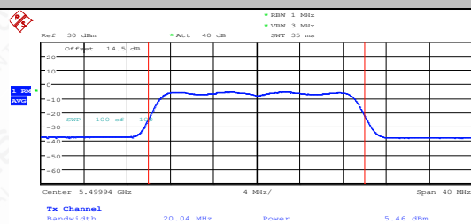
11AC20MIMO-Ant1-5500-PASS
