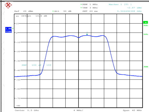
11N20MIMO-Ant2-5500-PASS
