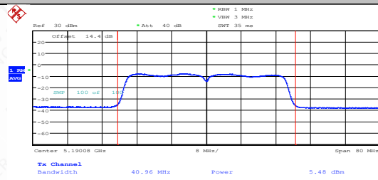
11AC40MIMO-Ant1-5190-PASS
