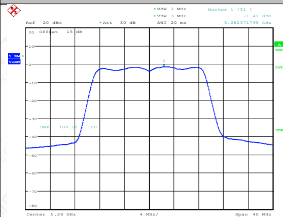
11N20SISO-Ant2-5280-PASS
