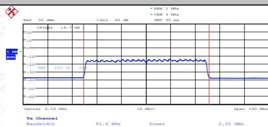
11AX80MIMO-Ant1-5530-PASS
