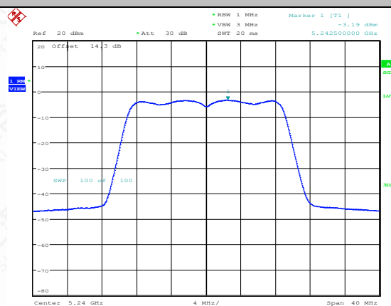
11N20MIMO-Ant1-5240-PASS
