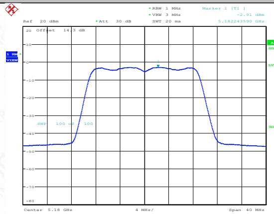
11N20MIMO-Ant1-5180-PASS
