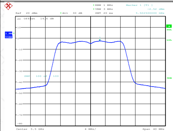
11N20SISO-Ant2-5500-PASS
