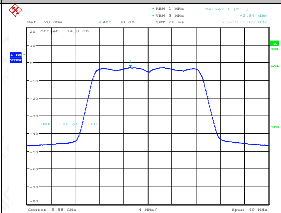
11N20MIMO-Ant2-5580-PASS
