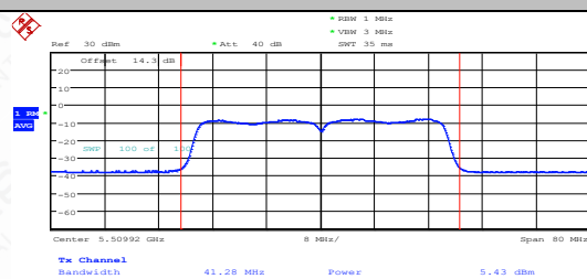
11N40MIMO-Ant1-5510-PASS
