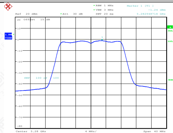
11A-CDD-Ant1-5280-PASS
