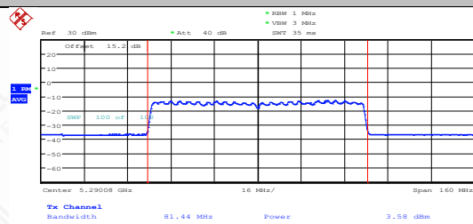
11AX80MIMO-Ant1-5290-PASS
