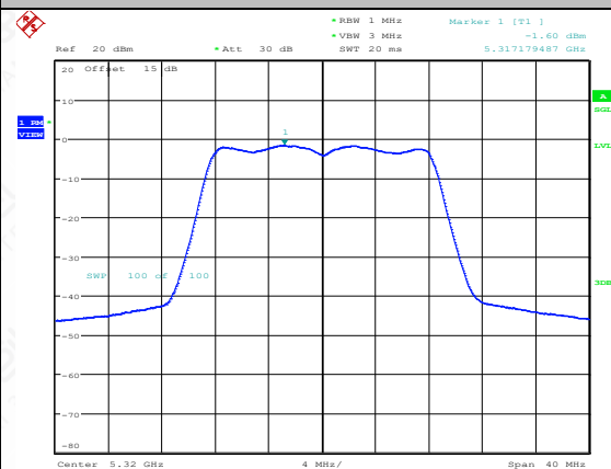
11A-CDD-Ant2-5320-PASS
