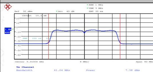
11AC40SISO-Ant2-5310-PASS
