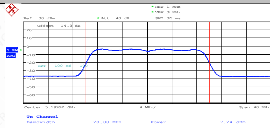
11AC20MIMO-Ant1-5200-PASS
