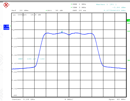
11N20MIMO-Ant1-5280-PASS
