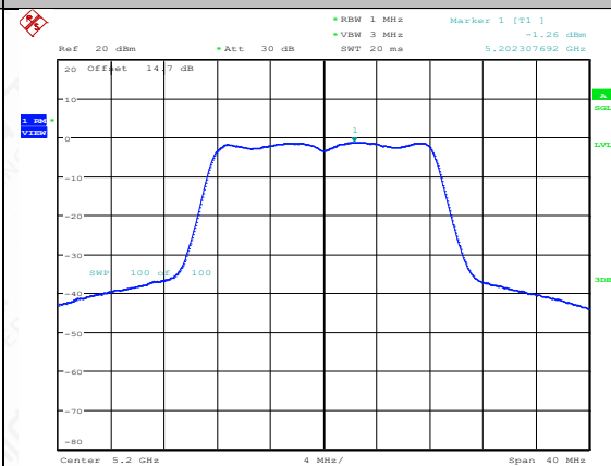
11A-CDD-Ant2-5200-PASS
