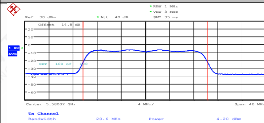
11AX20MIMO-Ant2-5580-PASS
