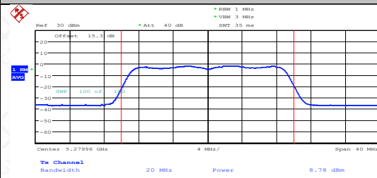
11AC20MIMO-Ant2-5280-PASS
