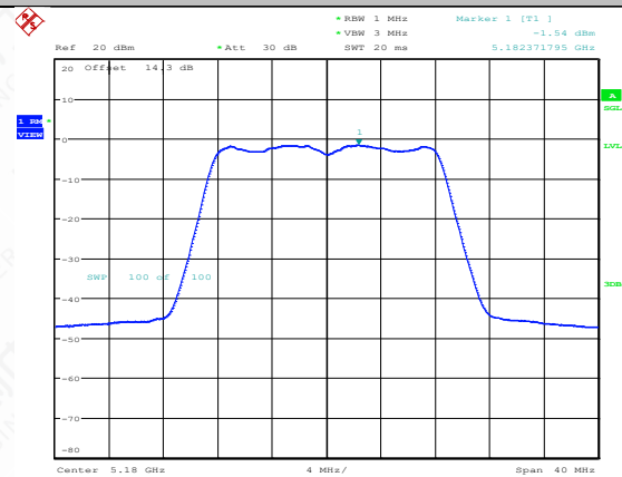
11A-CDD-Ant1-5180-PASS
