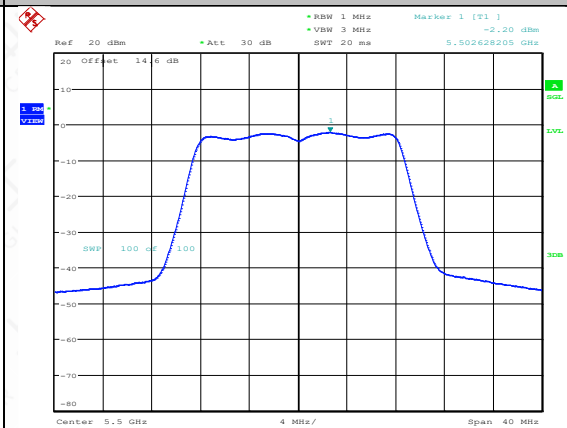
11A-Ant2-5500-PASS
