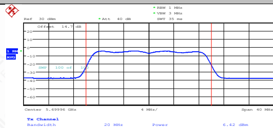
11AC20MIMO-Ant1-5700-PASS
