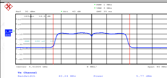
11AC40MIMO-Ant2-5510-PASS
