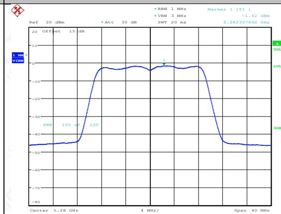
11N20MIMO-Ant2-5280-PASS
