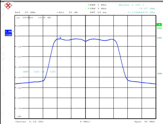
11N20MIMO-Ant2-5180-PASS
