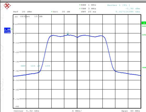
11N20SISO-Ant2-5320-PASS
