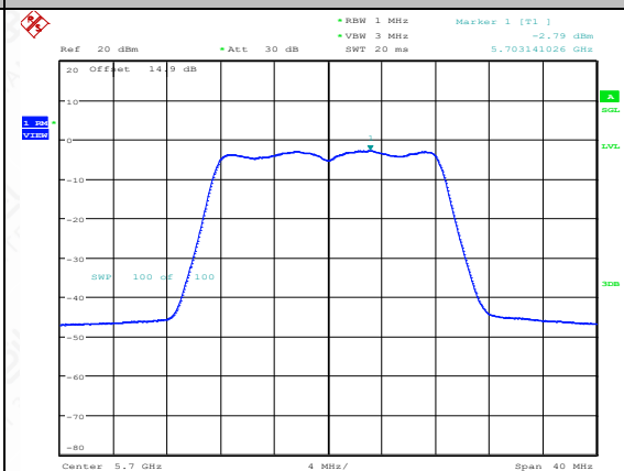
11A-Ant2-5700-PASS
