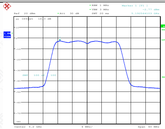
11N20SISO-Ant1-5200-PASS
