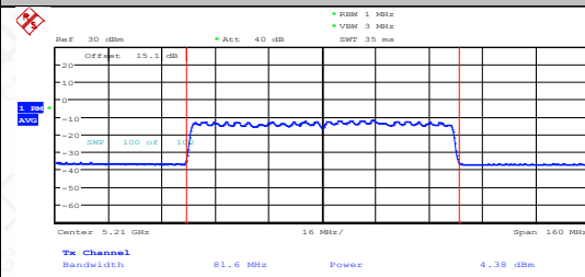
11AX80MIMO-Ant2-5210-PASS
