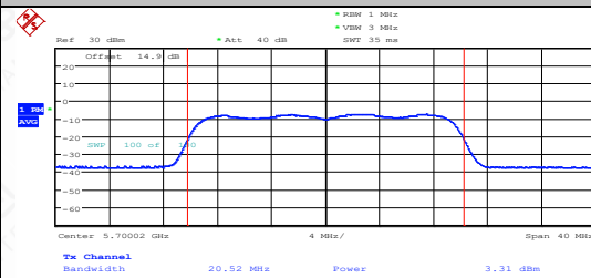
11AX20MIMO-Ant2-5700-PASS
