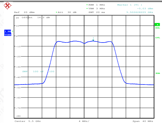
11A-Ant1-5500-PASS
