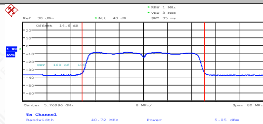
11AC40SISO-Ant1-5270-PASS
