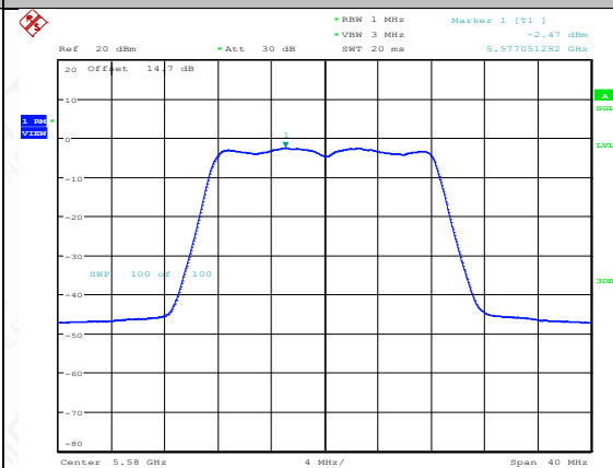
11A-CDD-Ant2-5580-PASS
