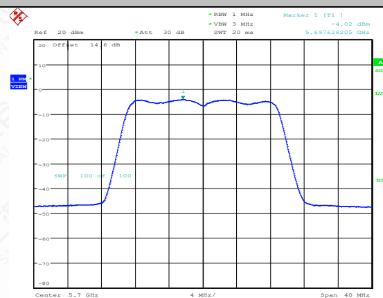
11N20MIMO-Ant1-5700-PASS
