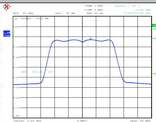
11N20SISO-Ant1-5240-PASS
