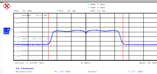
11N40MIMO-Ant1-5310-PASS
