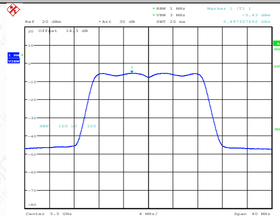
11N20MIMO-Ant1-5500-PASS
