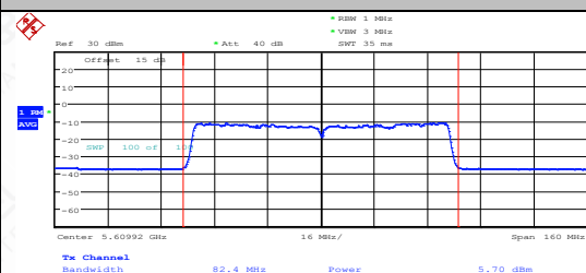
11AC80MIMO-Ant2-5610-PASS
