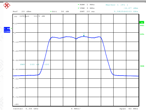
11A-Ant1-5580-PASS
