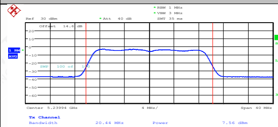
11AC20MIMO-Ant2-5240-PASS
