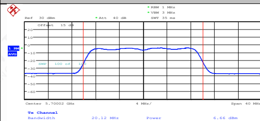
11AC20MIMO-Ant2-5700-PASS
