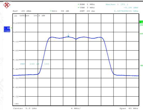
11N20SISO-Ant1-5500-PASS
