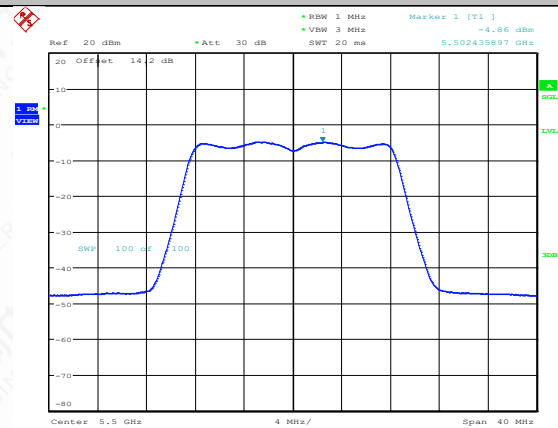
11A-CDD-Ant1-5500-PASS
