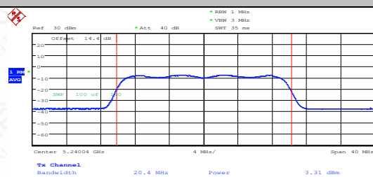
11AX20MIMO-Ant1-5240-PASS
