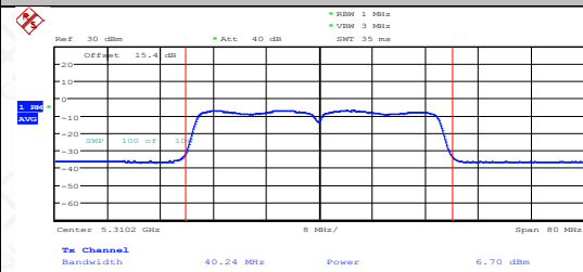
11AC40MIMO-Ant2-5310-PASS
