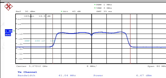
11AC40SISO-Ant2-5270-PASS
