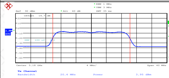
11AX20MIMO-Ant2-5180-PASS
