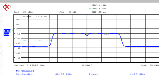
11AC40MIMO-Ant1-5270-PASS
