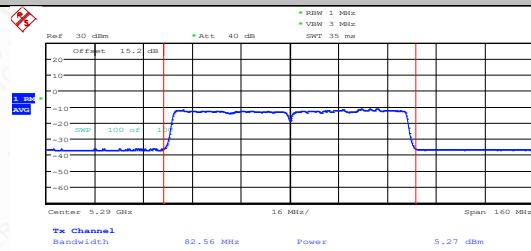
11AC80MIMO-Ant1-5290-PASS
