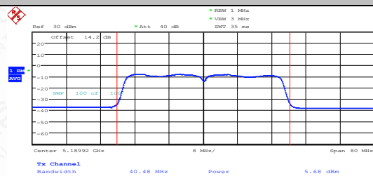
11AC40SISO-Ant1-5190-PASS
