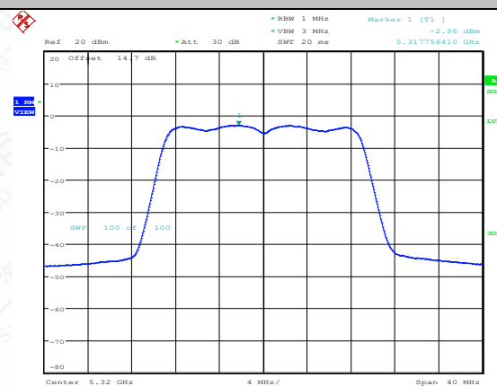
11N20MIMO-Ant1-5320-PASS
