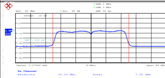
11N40MIMO-Ant2-5270-PASS
