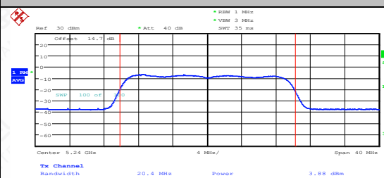
11AX20MIMO-Ant2-5240-PASS
