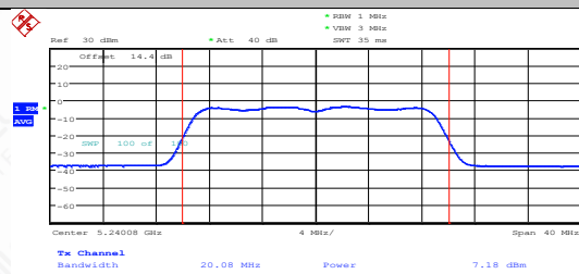
11AC20MIMO-Ant1-5240-PASS
