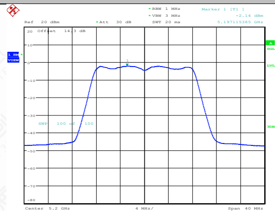
11A-CDD-Ant1-5200-PASS
