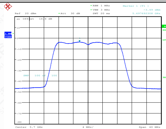
11N20SISO-Ant1-5700-PASS
