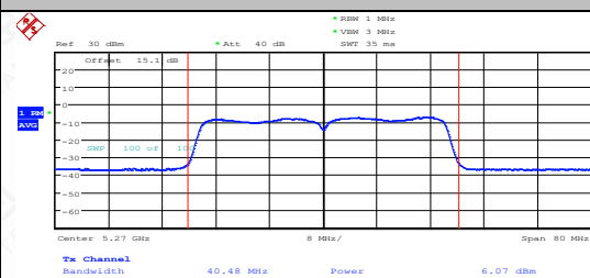
11AC40MIMO-Ant2-5270-PASS
