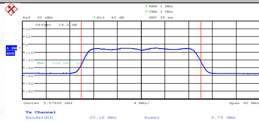
11AC20MIMO-Ant1-5580-PASS
