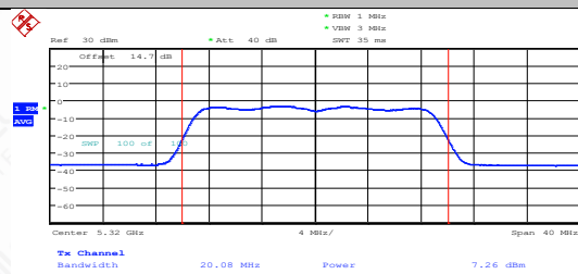
11AC20MIMO-Ant1-5320-PASS
