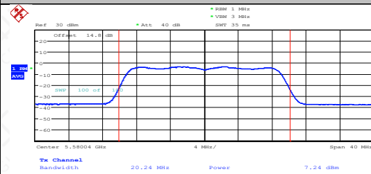
11AC20MIMO-Ant2-5580-PASS
