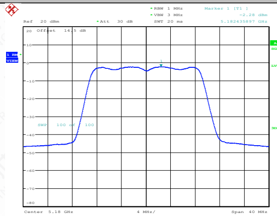
11N20SISO-Ant1-5180-PASS
