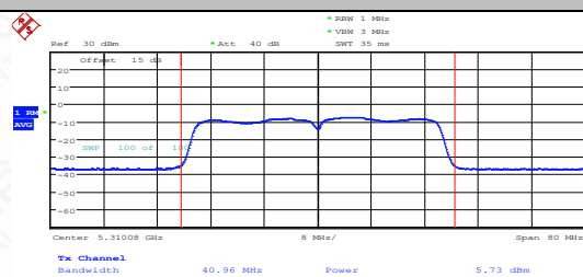
11AC40SISO-Ant1-5310-PASS
