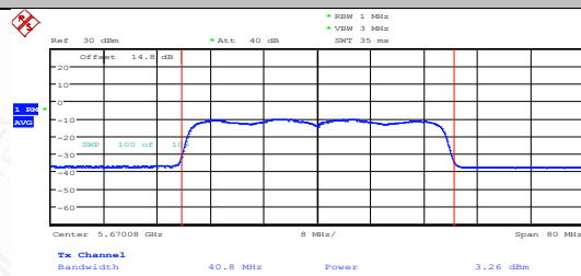
11AX40MIMO-Ant1-5670-PASS
