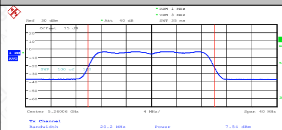
11AC20MIMO-Ant2-5260-PASS
