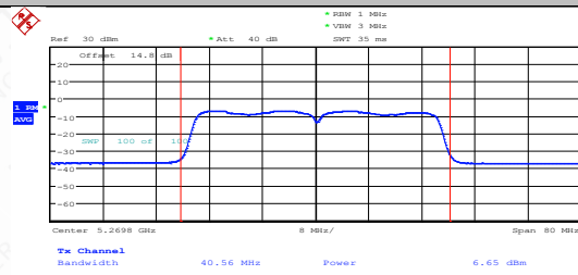
11N40MIMO-Ant1-5270-PASS
