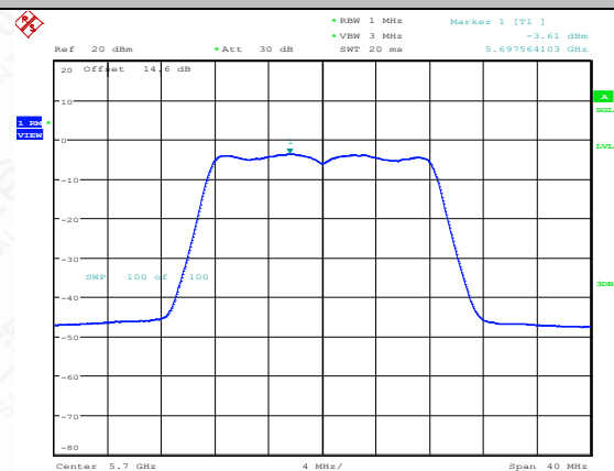
11A-CDD-Ant1-5700-PASS
