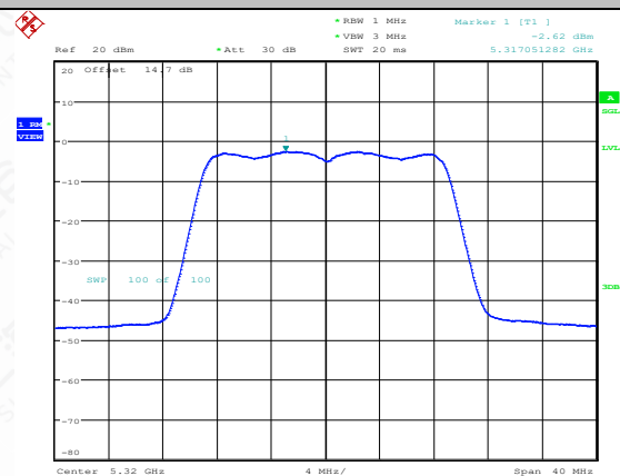
11N20SISO-Ant1-5320-PASS
