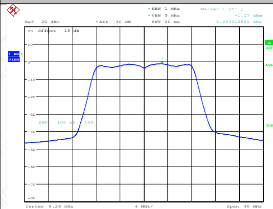
11A-Ant2-5280-PASS
