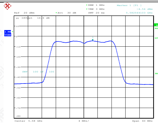
11N20SISO-Ant1-5580-PASS
