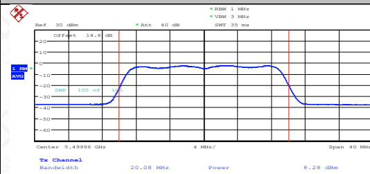
11N20MIMO-Ant2-5500-PASS
