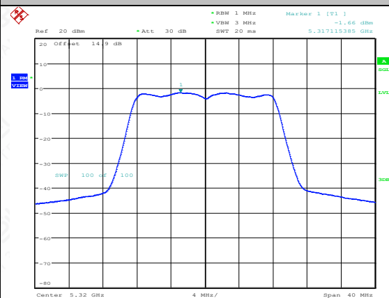
11A-Ant2-5320-PASS
