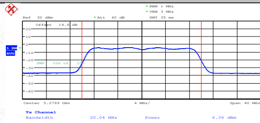
11AC20MIMO-Ant1-5280-PASS
