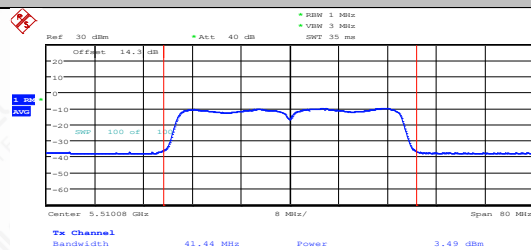
11AC40MIMO-Ant1-5510-PASS
