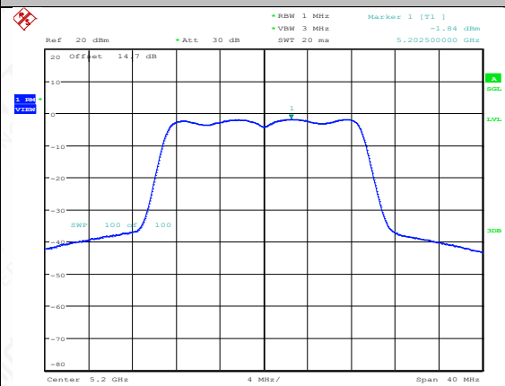
11N20SISO-Ant2-5200-PASS
