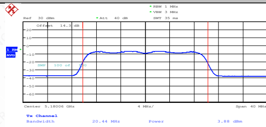
11AX20MIMO-Ant1-5180-PASS
