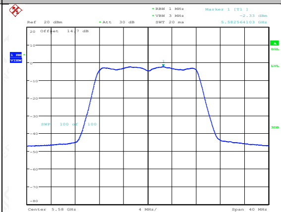
11A-Ant2-5580-PASS
