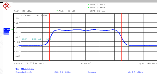
11N20MIMO-Ant1-5580-PASS
