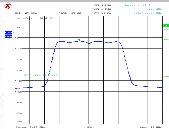
11N20SISO-Ant1-5260-PASS
