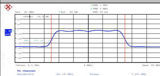
11AC20MIMO-Ant2-5500-PASS
