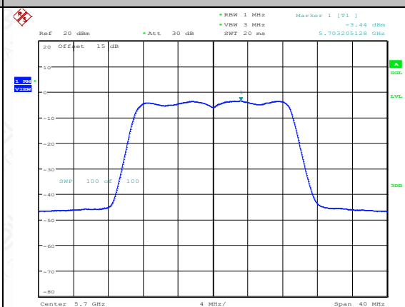
11N20MIMO-Ant2-5700-PASS
