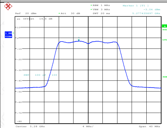
11A-CDD-Ant2-5280-PASS
