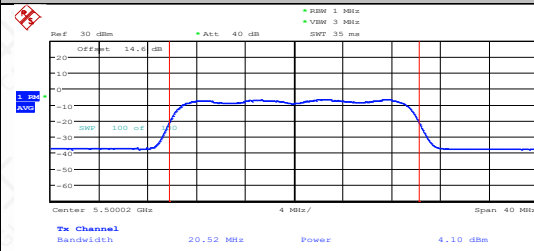
11AX20MIMO-Ant2-5500-PASS
