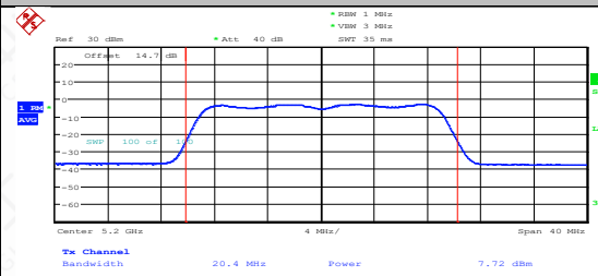
11AC20MIMO-Ant2-5200-PASS
