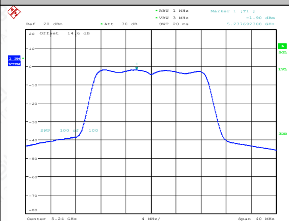
11N20SISO-Ant2-5240-PASS
