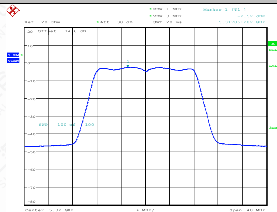
11A-CDD-Ant1-5320-PASS
