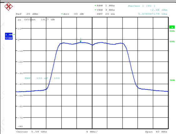
11N20SISO-Ant2-5580-PASS
