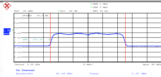
11AX40MIMO-Ant1-5550-PASS
