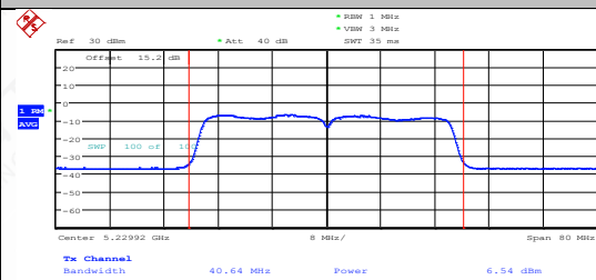
11AC40MIMO-Ant2-5230-PASS
