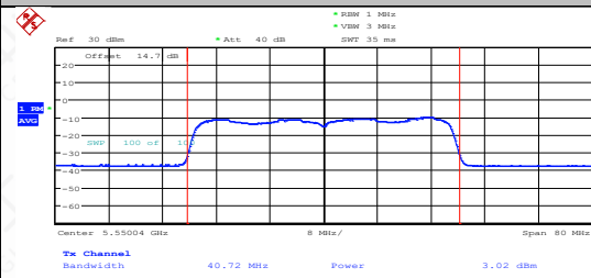
11AX40MIMO-Ant2-5550-PASS
