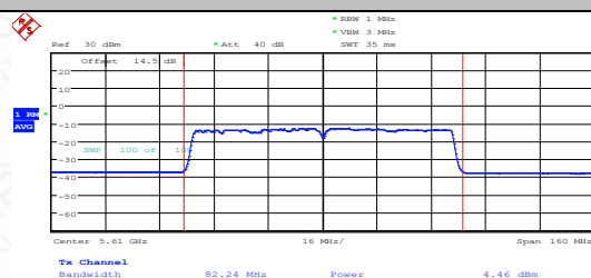
11AC80MIMO-Ant1-5610-PASS
