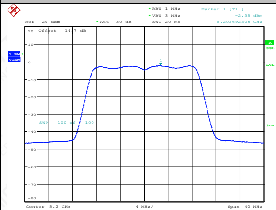
11N20MIMO-Ant2-5200-PASS
