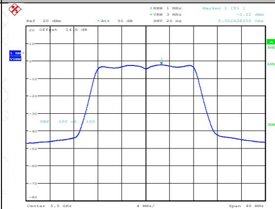
11A-CDD-Ant2-5500-PASS
