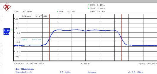
11AC20MIMO-Ant1-5260-PASS
