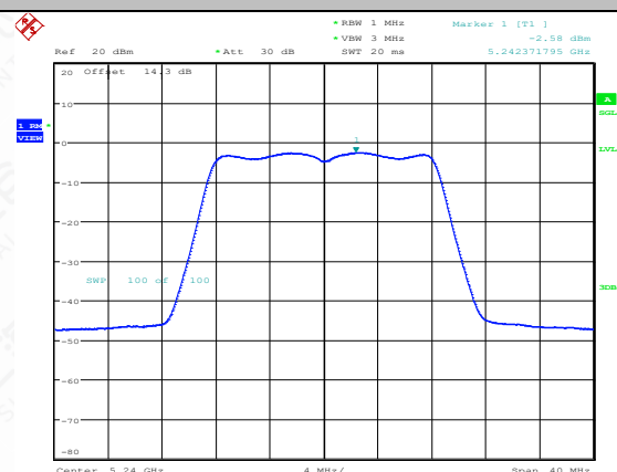
11A-CDD-Ant1-5240-PASS
