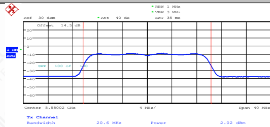
11AX20MIMO-Ant1-5580-PASS
