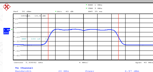
11N20MIMO-Ant1-5700-PASS
