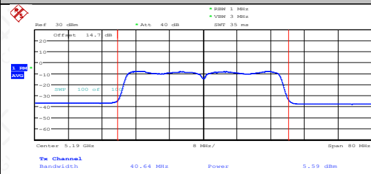
11AC40MIMO-Ant2-5190-PASS
