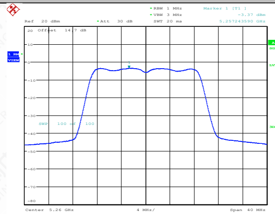
11N20MIMO-Ant1-5260-PASS
