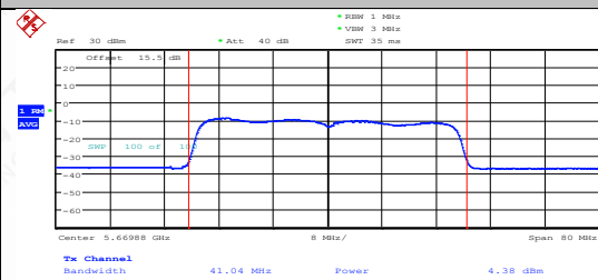
11AX40MIMO-Ant2-5670-PASS
