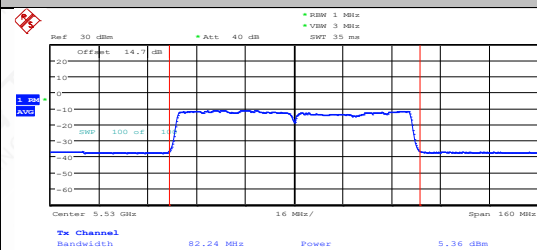
11AC80MIMO-Ant2-5530-PASS
