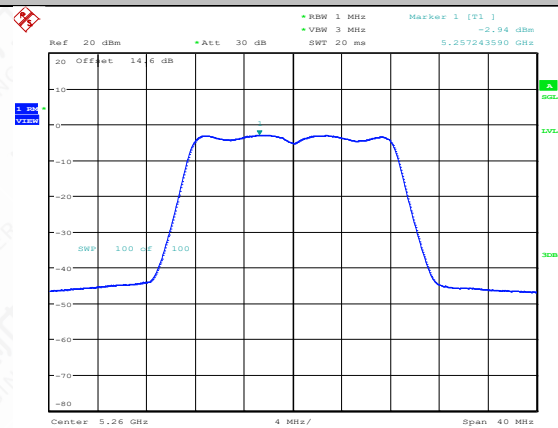
11A-Ant1-5260-PASS
