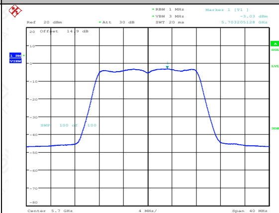
11A-CDD-Ant2-5700-PASS
