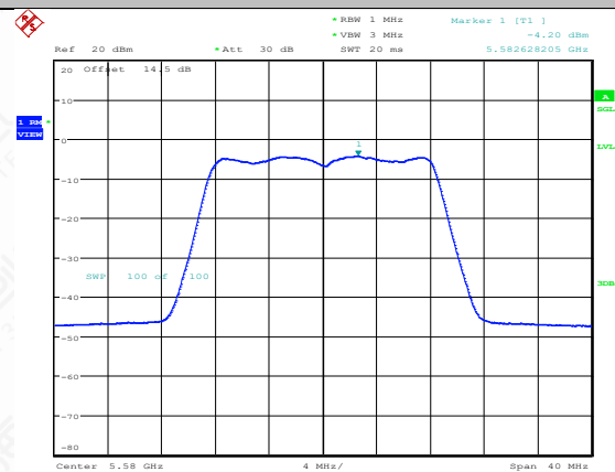
11A-CDD-Ant1-5580-PASS
