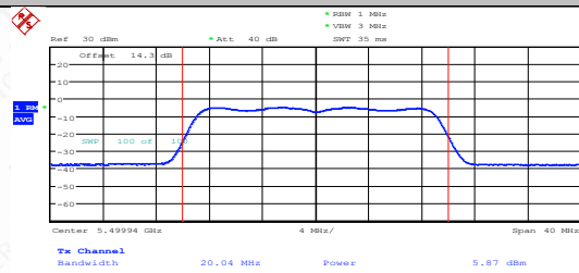
11N20MIMO-Ant1-5500-PASS
