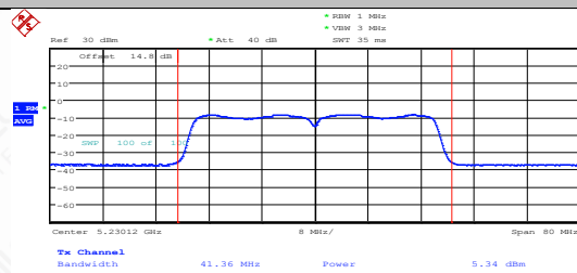
11AC40MIMO-Ant1-5230-PASS
