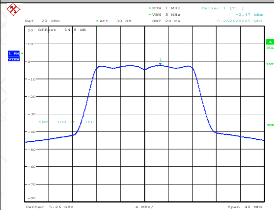
11A-Ant2-5260-PASS
