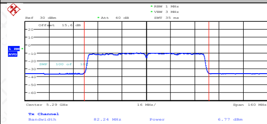
11AC80MIMO-Ant2-5290-PASS
