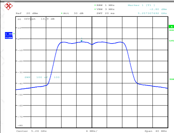
11N20SISO-Ant2-5260-PASS
