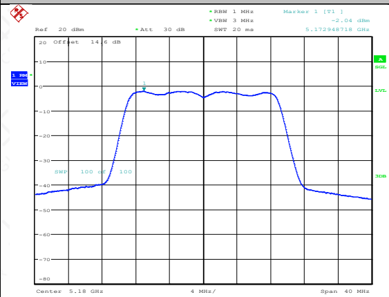
11N20SISO-Ant2-5180-PASS
