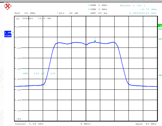
11N20MIMO-Ant1-5580-PASS
