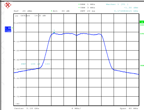
11A-CDD-Ant2-5180-PASS
