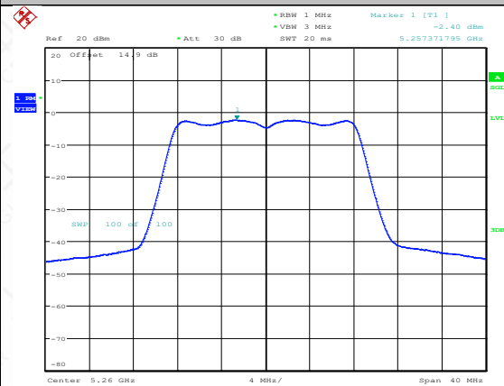
11A-CDD-Ant2-5260-PASS
