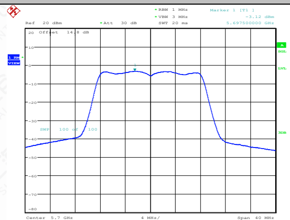
11A-Ant1-5700-PASS
