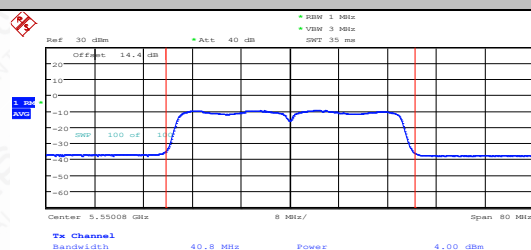
11AC40MIMO-Ant1-5550-PASS
