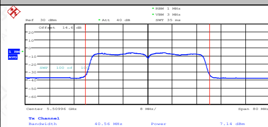
11N40MIMO-Ant2-5510-PASS
