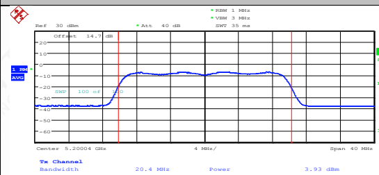
11AX20MIMO-Ant2-5200-PASS
