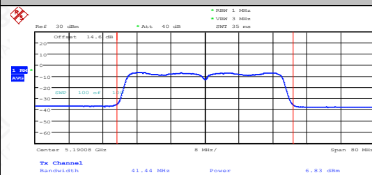
11AC40SISO-Ant2-5190-PASS
