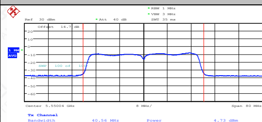
11AC40MIMO-Ant2-5550-PASS
