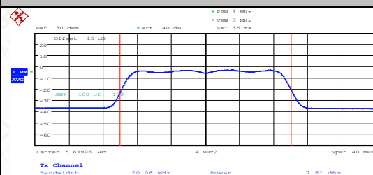
11N20MIMO-Ant2-5700-PASS
