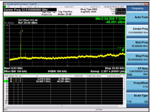
11N20SISO-Ant1-2412-30~25000-PASS
