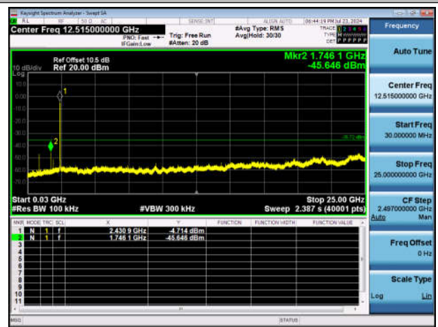
11N20SISO-Ant1-2437-30~25000-PASS
