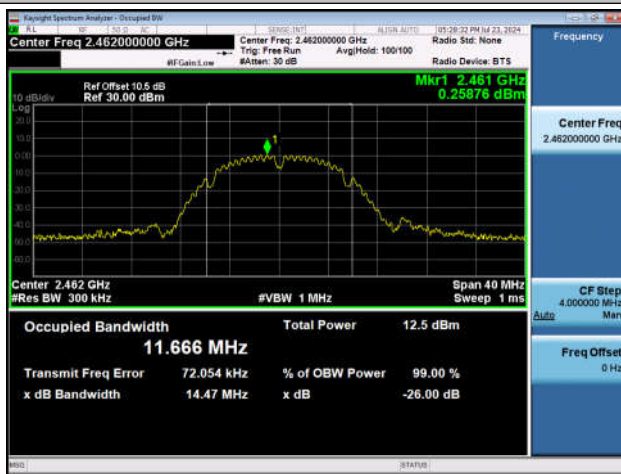
11B-Ant1-2462
