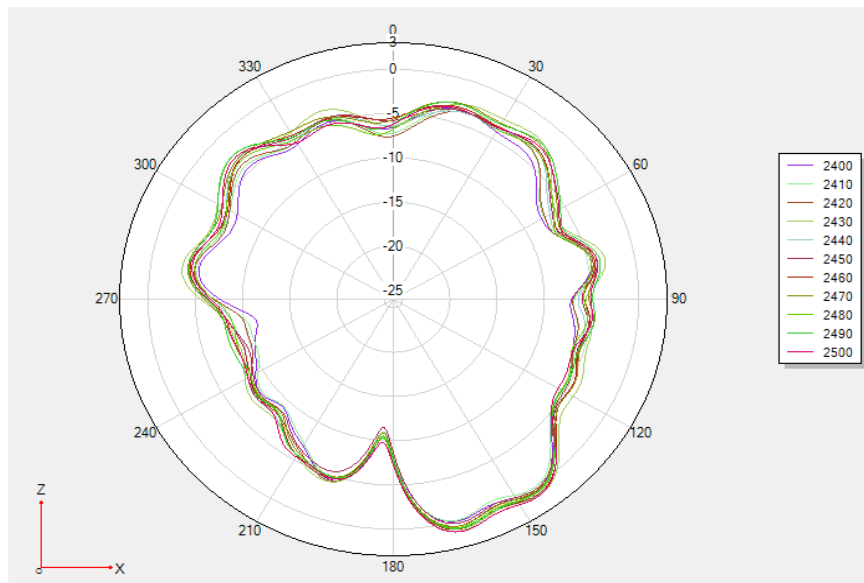
Phi 90 2D
