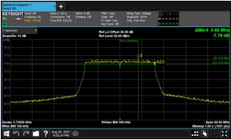
Figure 724 - Core 0 (A) 5720 MHz (CH144) 6 dB Bandwidth
