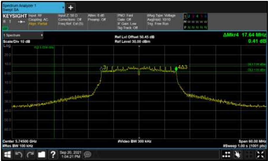
Figure 904 - Core 0 (A) 5745 MHz (CH149) 6 dB Bandwidth
