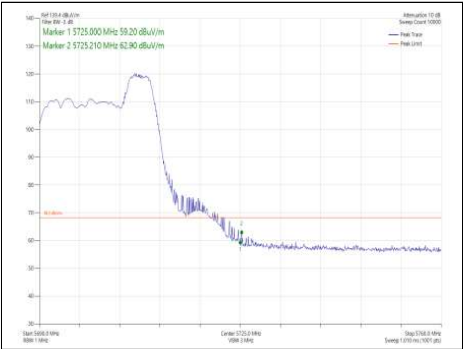
Figure 942- 802.11ax HE20, Core 0, 52-40 - 5700 MHz Band Edge Frequency 5725 MHz
