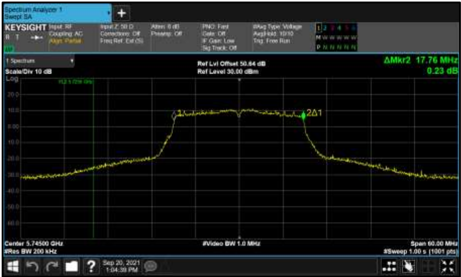
Figure 905 - Core 1 (B) 5745 MHz (CH149) 99% Bandwidth
