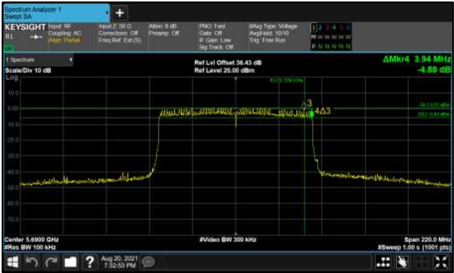
Figure 884 - Core 0 (A) 5690 MHz (CH138) 6 dB Bandwidth
