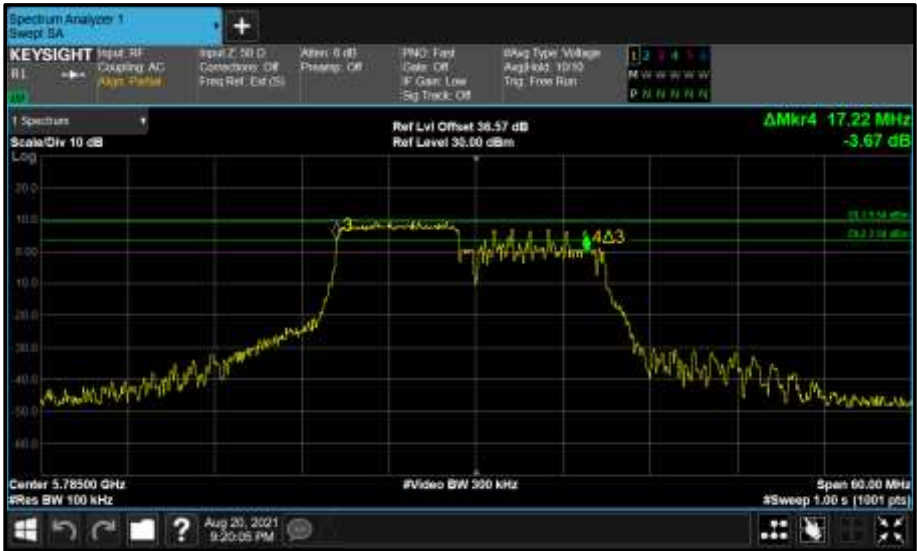
Figure 826 - Core 0 (A) 5785 MHz (CH157) 6 dB Bandwidth
