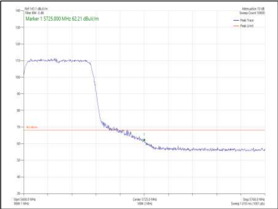
Figure 941- 802.11ax HE20, Core 0, SU - 5700 MHz Band Edge Frequency 5725 MHz
