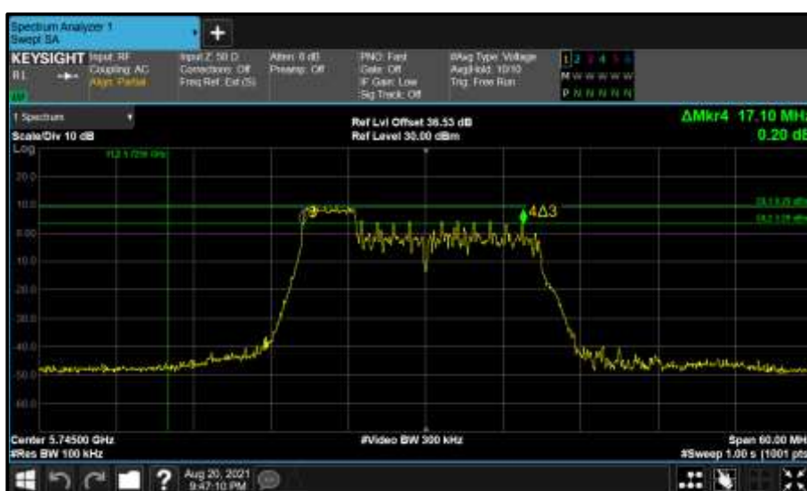
Figure 798 - Core 0 (A) 5745 MHz (CH149) 6 dB Bandwidth
