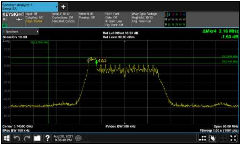
Figure 746 - Core 0 (A) 5745 MHz (CH149) 6 dB Bandwidth
