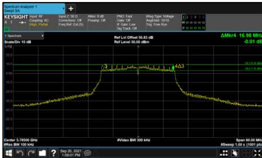
Figure 910 - Core 1 (B) 5785 MHz (CH157) 6 dB Bandwidth
