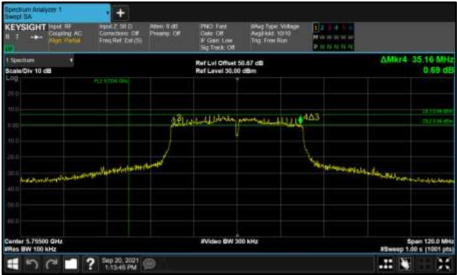
Figure 922 - Core 1 (B) 5755 MHz (CH151) 6 dB Bandwidth
