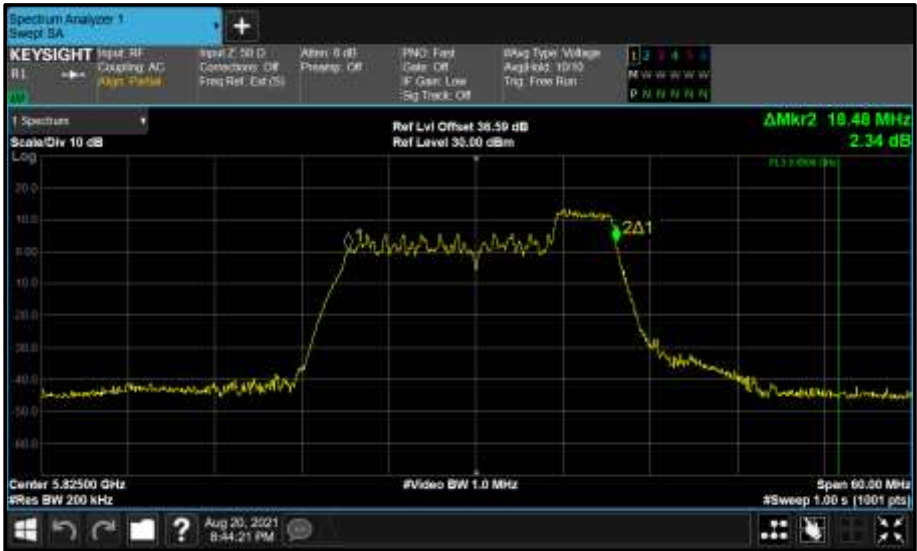
Figure 775 - Core 1 (B) 5825 MHz (CH165) 99% Bandwidth
