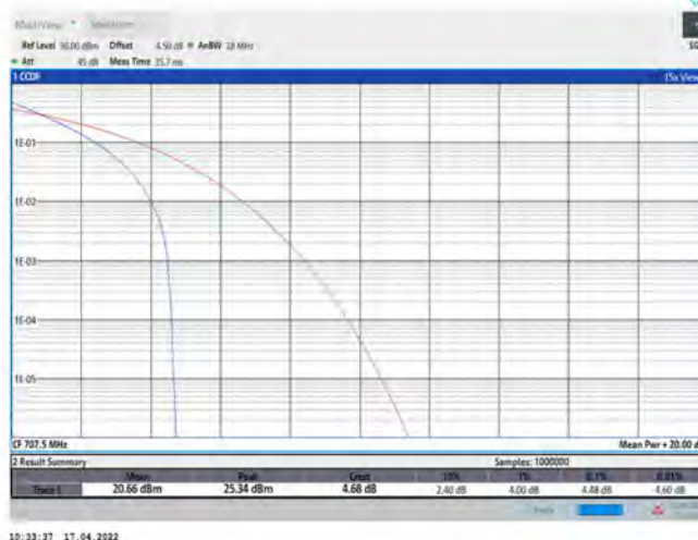
Band12-10MHz-QPSK-23095-50RB#0
