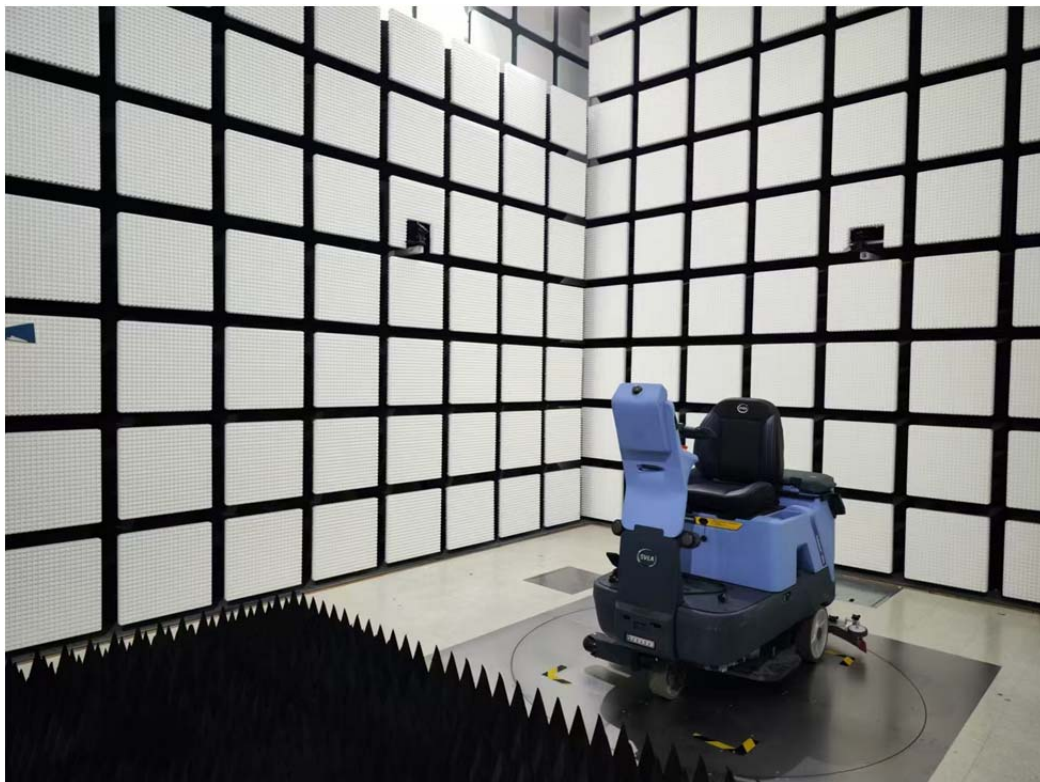
Radiated Emission Above 18-25GHz View
