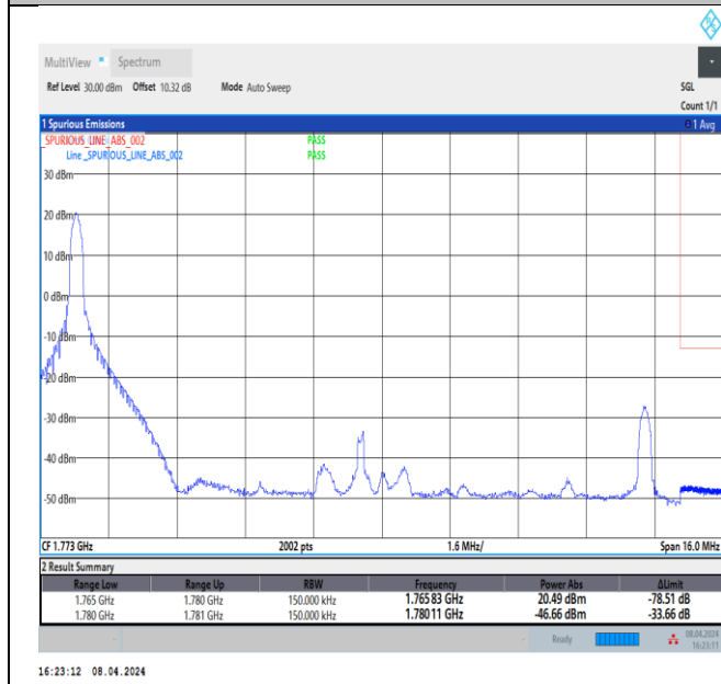
Band66_15MHz_64QAM_132597_1RB#0
