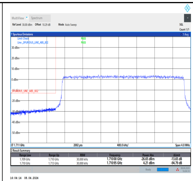
Band66_3MHz_16QAM_131987_15RB#0
