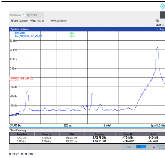
Band66_15MHz_QPSK_132047_1RB#74
