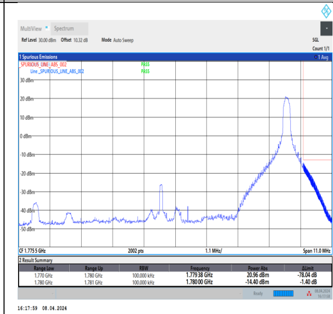
Band66_10MHz_16QAM_132622_1RB#49
