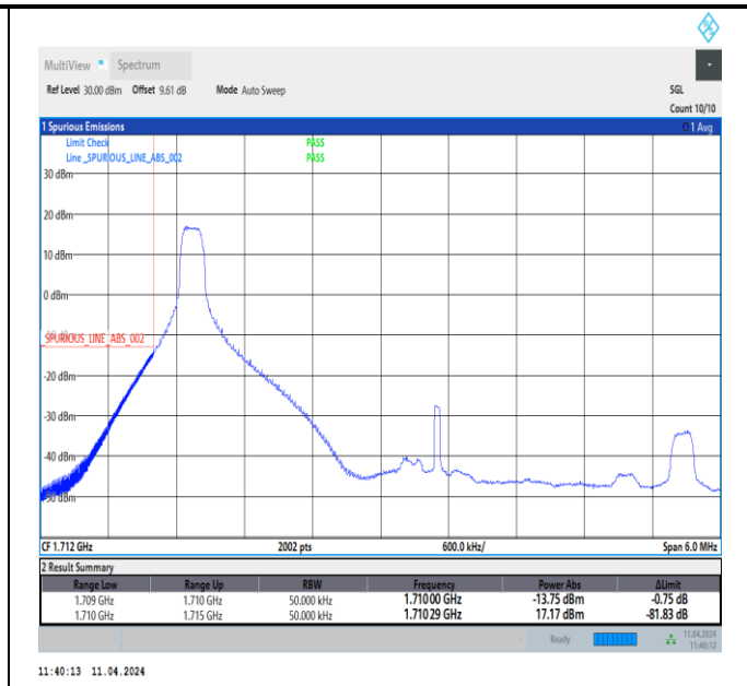
Band66_5MHz_16QAM_131997_1RB#0
