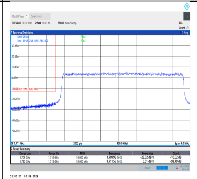
Band66_3MHz_QPSK_131987_15RB#0
