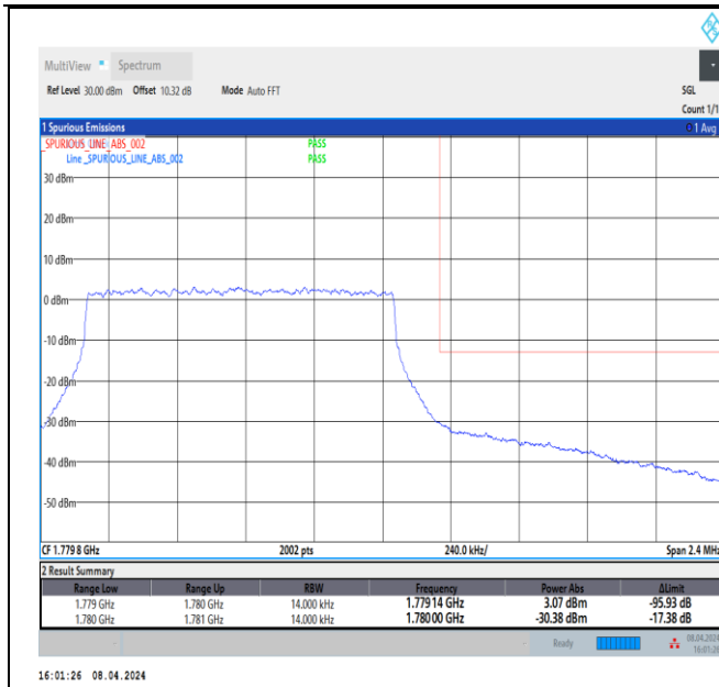
Band66_1.4MHz_64QAM_132665_6RB#0
