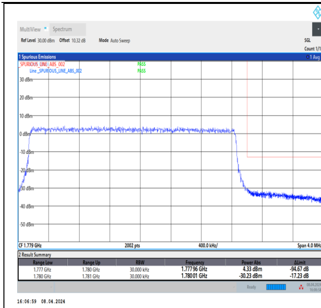
Band66_3MHz_16QAM_132657_15RB#0
