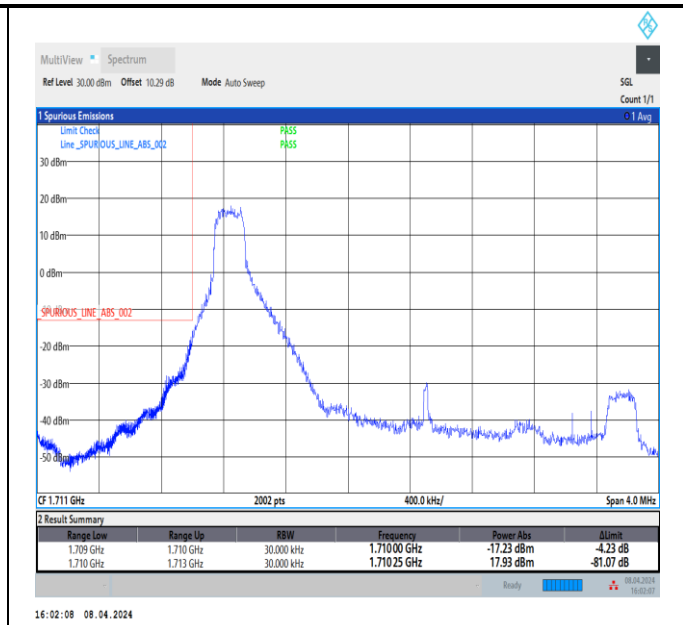
Band66_3MHz_QPSK_131987_1RB#0
