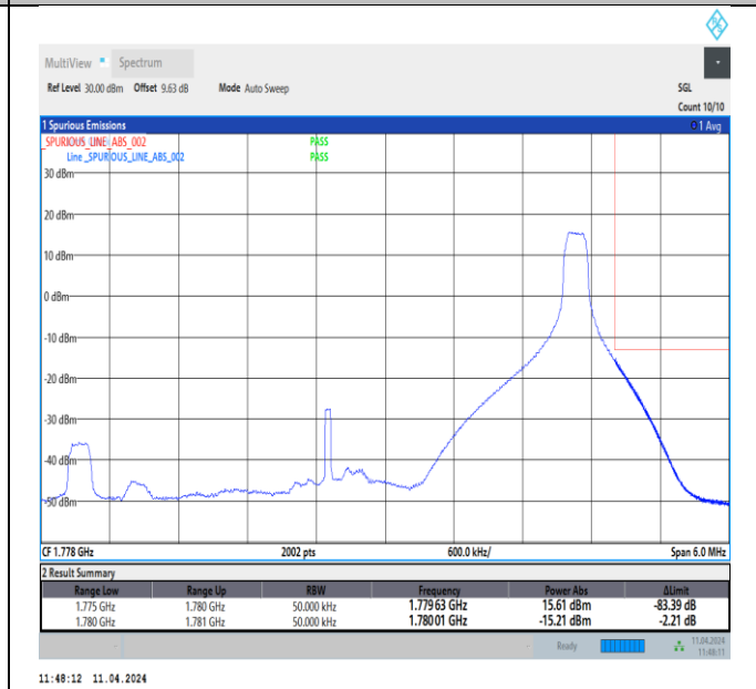
Band66_5MHz_64QAM_132647_1RB#24
