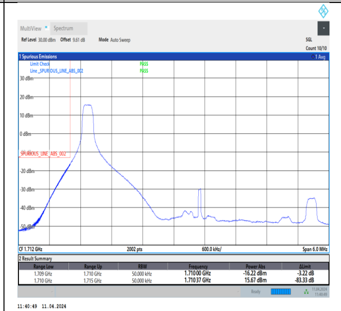
Band66_5MHz_64QAM_131997_1RB#0
