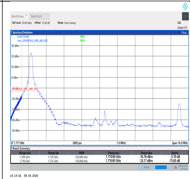
Band66_15MHz_QPSK_132047_1RB#0
