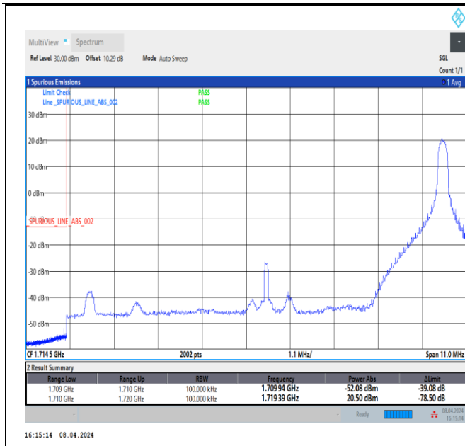
Band66_10MHz_16QAM_132022_1RB#49
