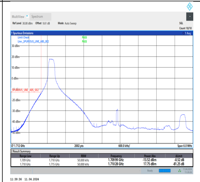
Band66_5MHz_QPSK_131997_1RB#0
