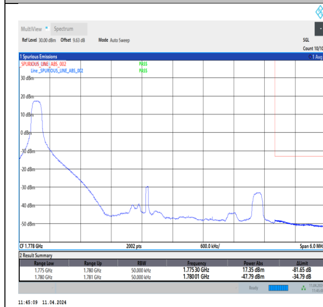
Band66_5MHz_QPSK_132647_1RB#0
