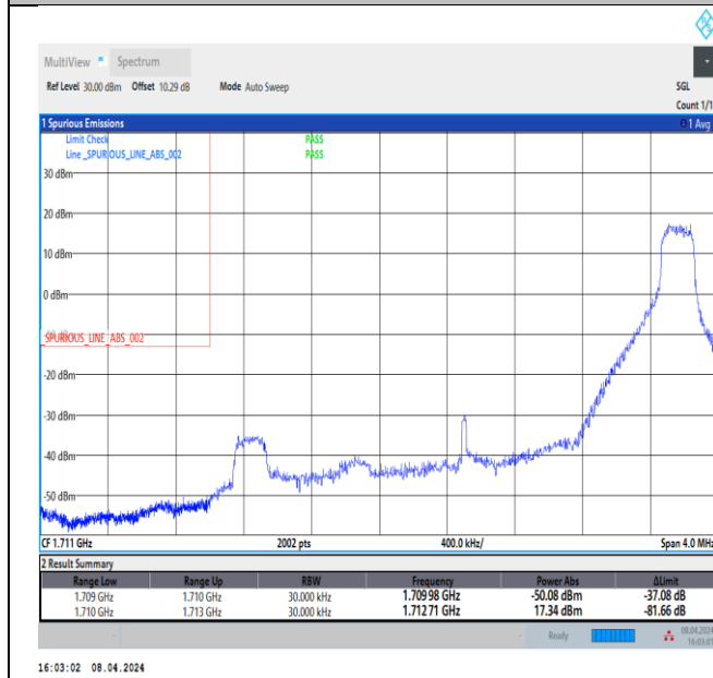
Band66_3MHz_QPSK_131987_1RB#14
