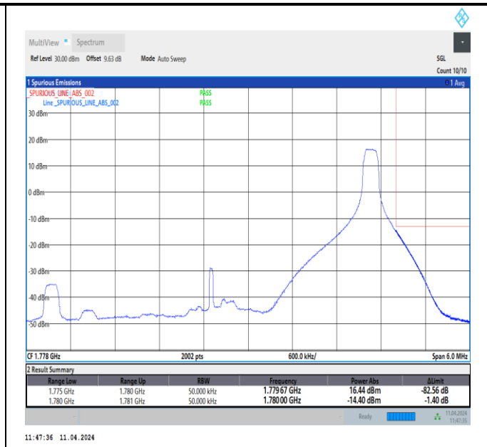
Band66_5MHz_16QAM_132647_1RB#24
