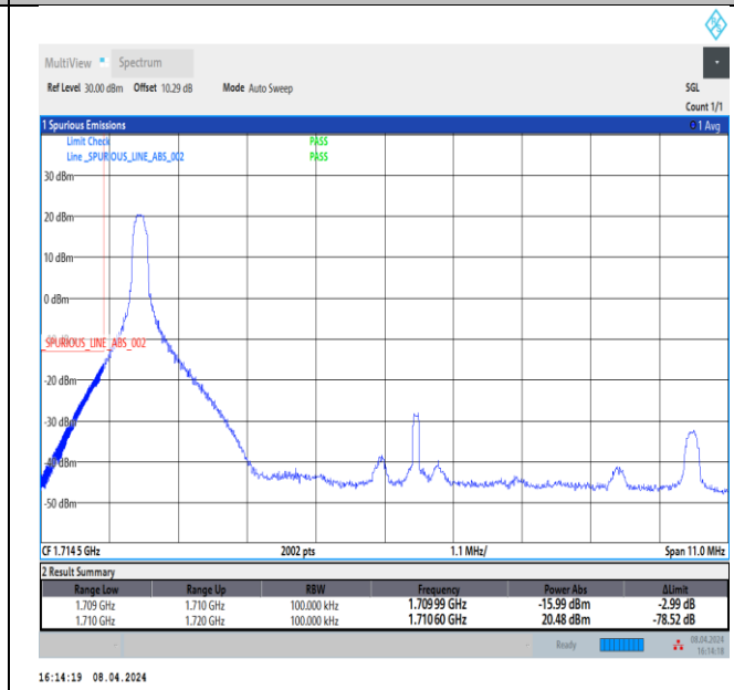
Band66_10MHz_16QAM_132022_1RB#0
