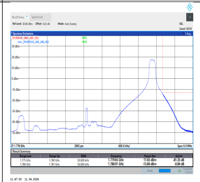
Band66_5MHz_QPSK_132647_1RB#24
