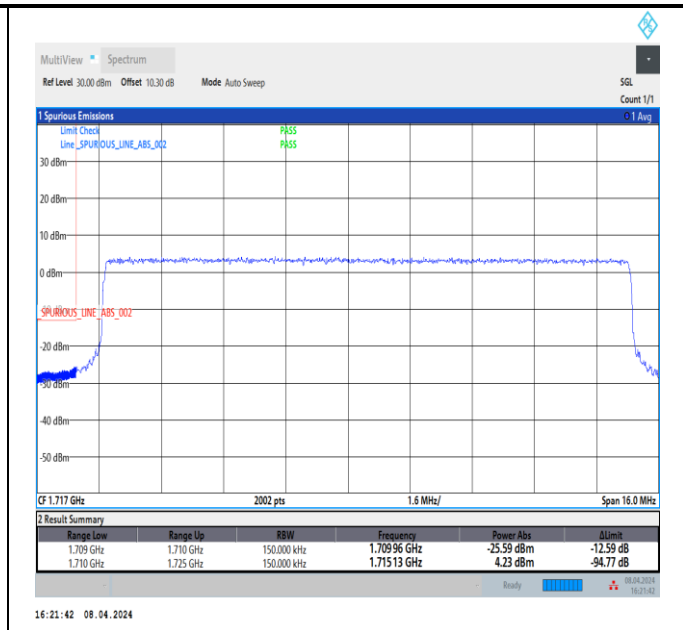
Band66_15MHz_QPSK_132047_75RB#0
