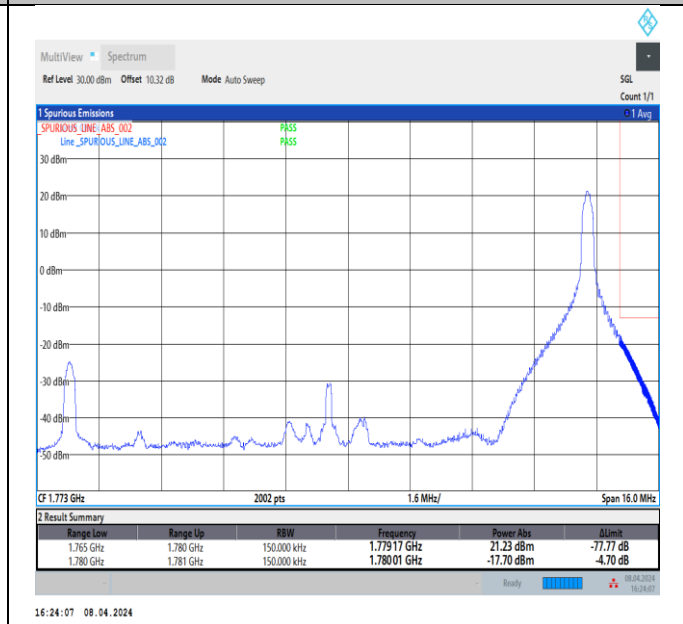
Band66_15MHz_64QAM_132597_1RB#74
