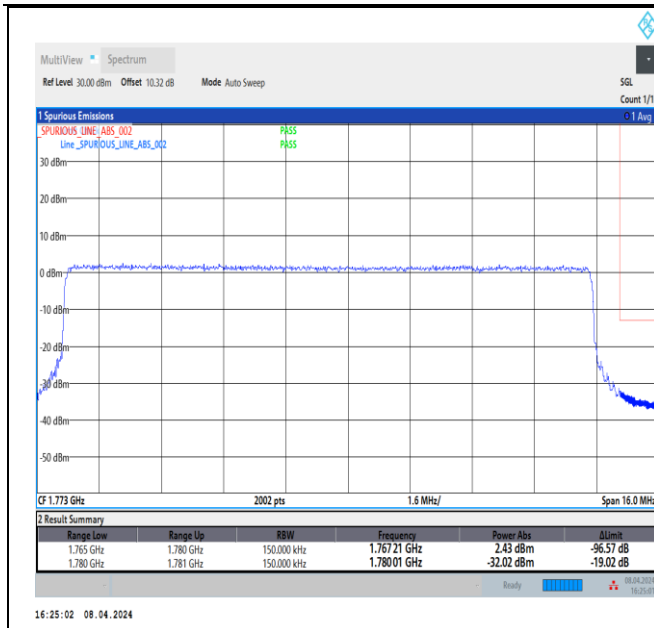
Band66_15MHz_64QAM_132597_75RB#0
