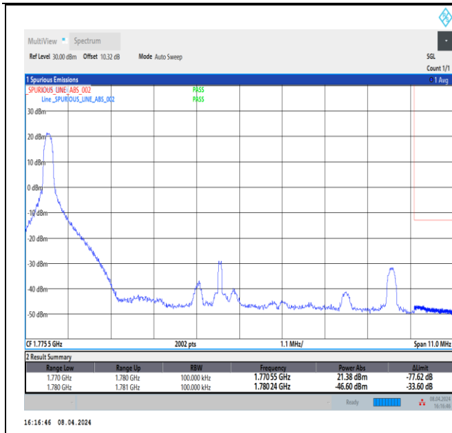
Band66_10MHz_QPSK_132622_1RB#0
