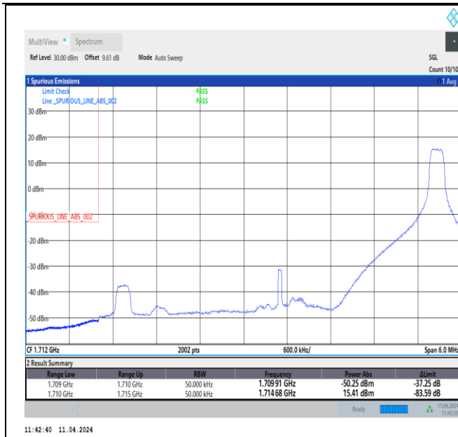
Band66_5MHz_64QAM_131997_1RB#24
