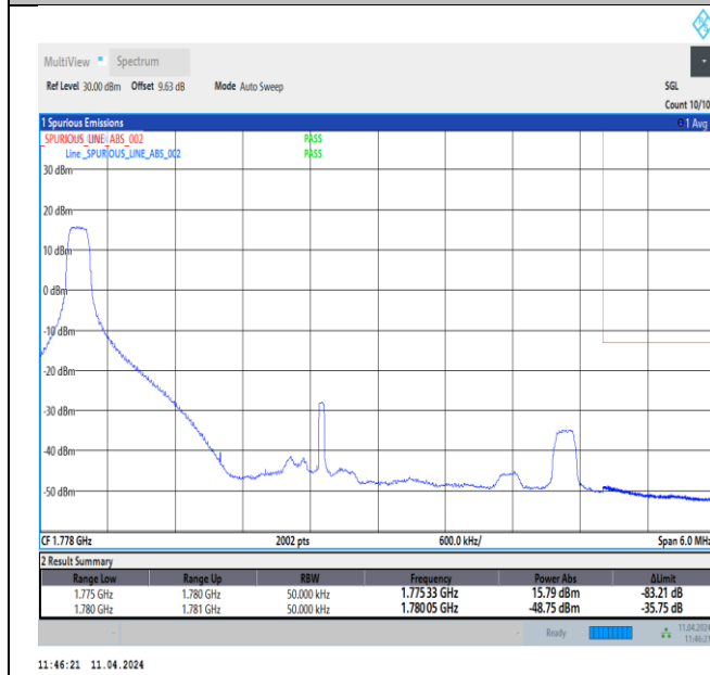
Band66_5MHz_64QAM_132647_1RB#0
