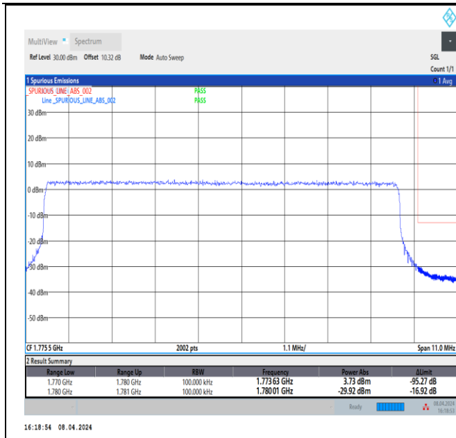
Band66_10MHz_16QAM_132622_50RB#0
