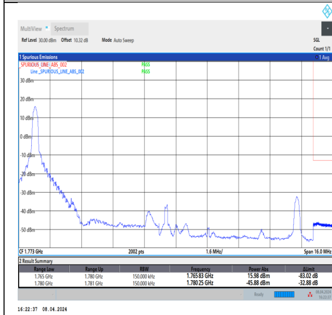
Band66_15MHz_QPSK_132597_1RB#0
