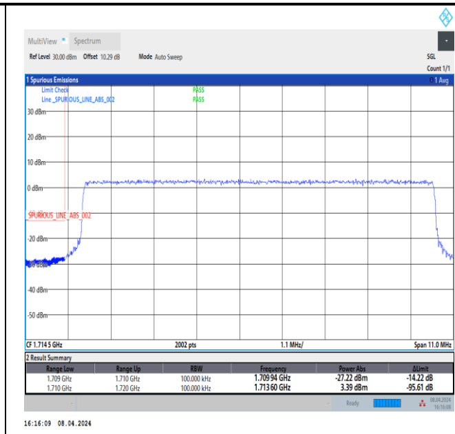
Band66_10MHz_16QAM_132022_50RB#0
