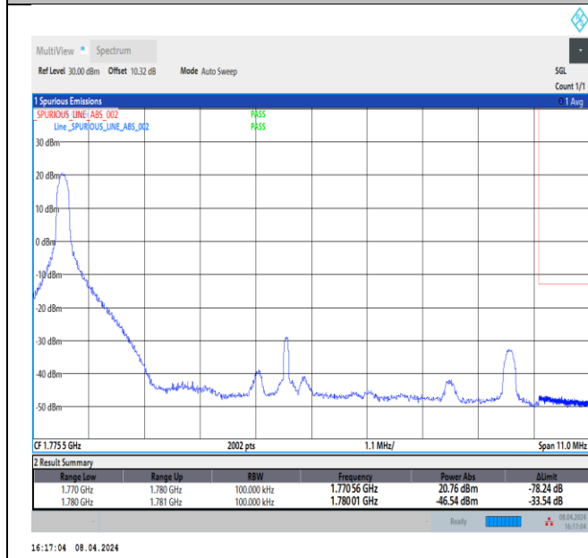
Band66_10MHz_16QAM_132622_1RB#0
