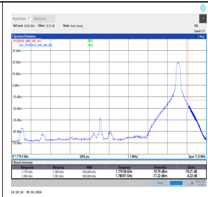
Band66_10MHz_64QAM_132622_1RB#49
