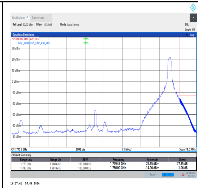
Band66_10MHz_QPSK_132622_1RB#49
