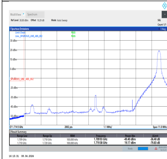
Band66_10MHz_64QAM_132022_1RB#49
