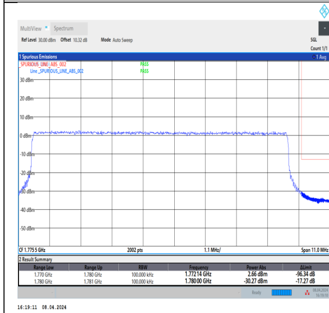
Band66_10MHz_64QAM_132622_50RB#0
