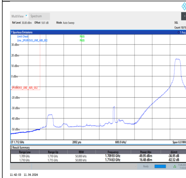
Band66_5MHz_16QAM_131997_1RB#24
