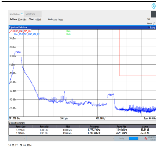
Band66_3MHz_64QAM_132657_1RB#0
