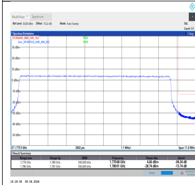
Band66_10MHz_QPSK_132622_50RB#0
