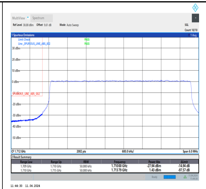
Band66_5MHz_64QAM_131997_25RB#0
