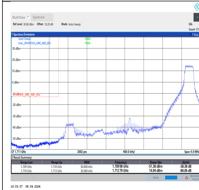
Band66_3MHz_64QAM_131987_1RB#14
