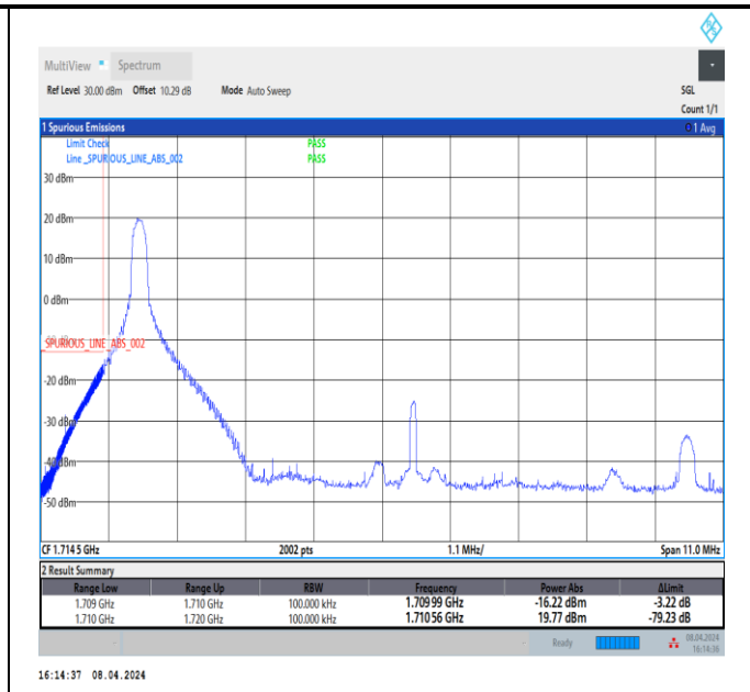
Band66_10MHz_64QAM_132022_1RB#0
