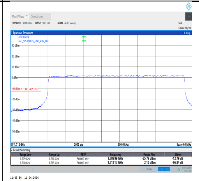
Band66_5MHz_16QAM_131997_25RB#0
