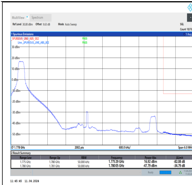
Band66_5MHz_16QAM_132647_1RB#0
