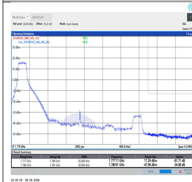
Band66_3MHz_16QAM_132657_1RB#0
