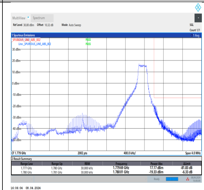
Band66_3MHz_16QAM_132657_1RB#14
