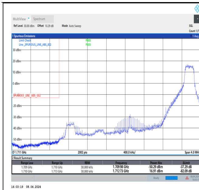
Band66_3MHz_16QAM_131987_1RB#14
