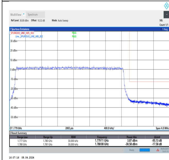
Band66_3MHz_64QAM_132657_15RB#0
