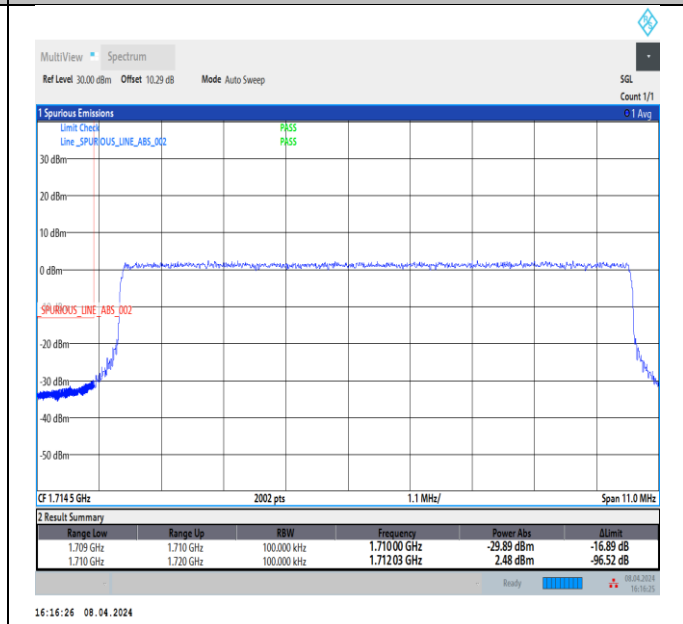
Band66_10MHz_64QAM_132022_50RB#0
