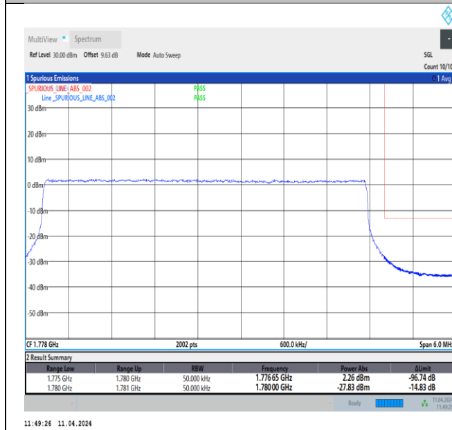
Band66_5MHz_16QAM_132647_25RB#0
