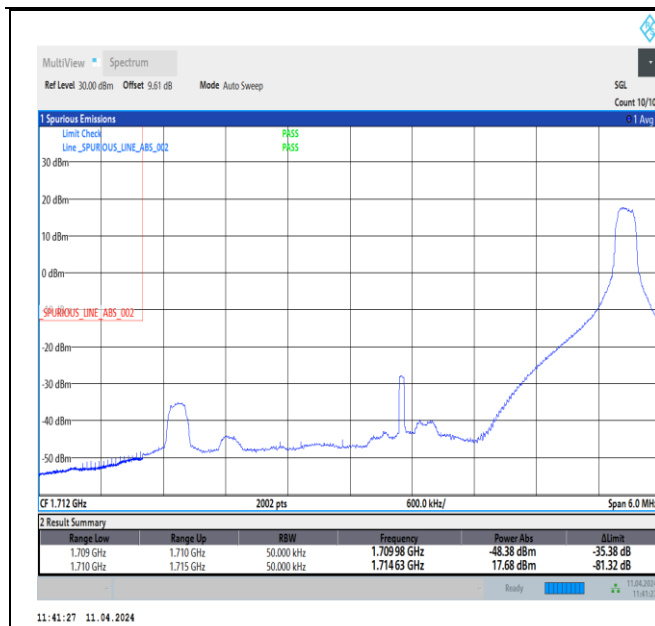
Band66_5MHz_QPSK_131997_1RB#24
