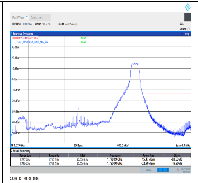
Band66_3MHz_64QAM_132657_1RB#14
