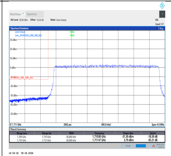
Band66_3MHz_64QAM_131987_15RB#0
