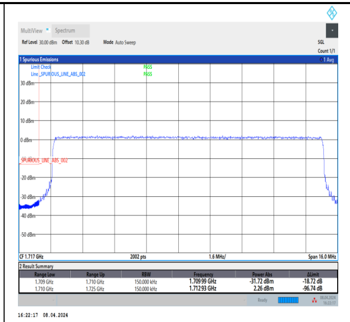
Band66_15MHz_64QAM_132047_75RB#0
