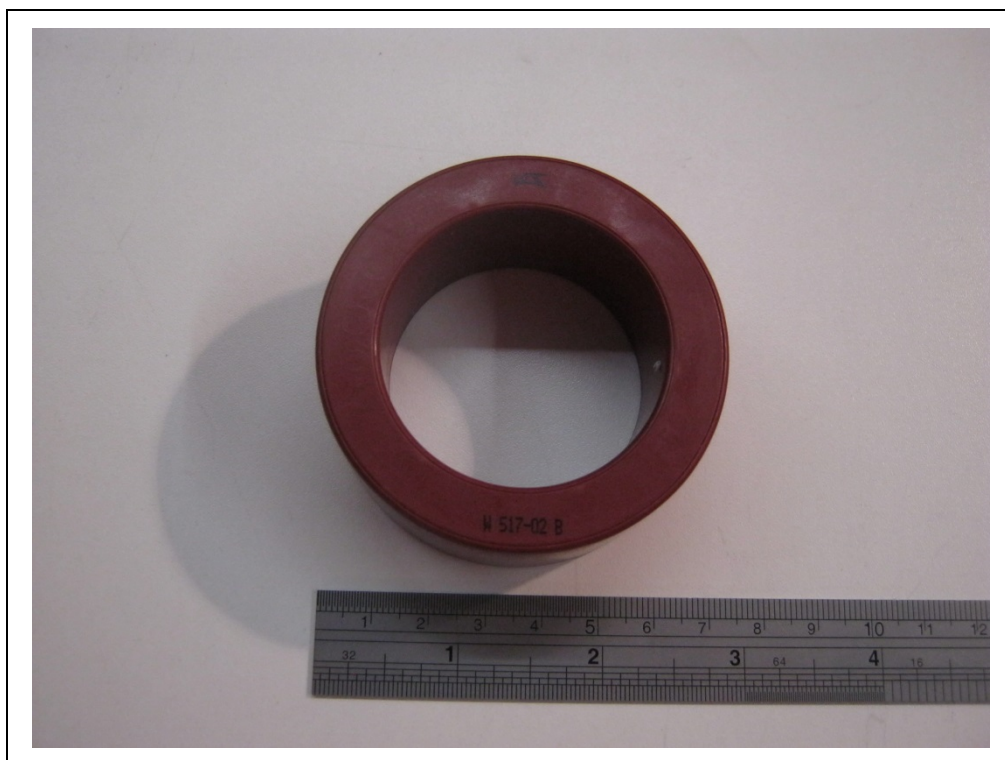
Photograph A3-6: Detail on ferrite VITROPERM 500F, Type T60006-L2063-W157
