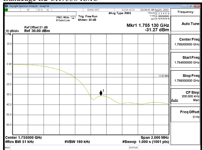
Bandedge B4 CH1513 RMC
