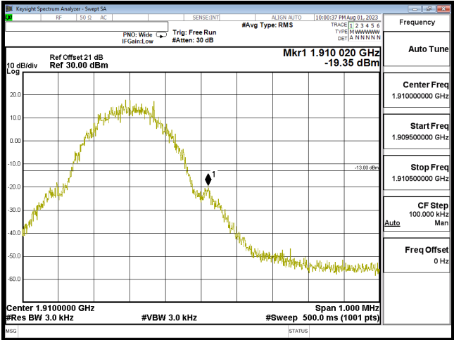
Bandedge 2G1900 CH810 VOICE
