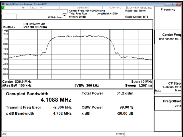
OCC B5 CH4183 RMC
