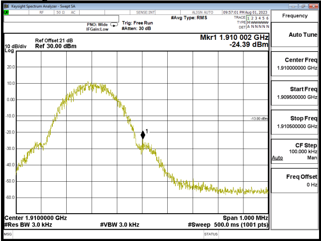
Bandedge 2G1900 CH810 EGPRS
