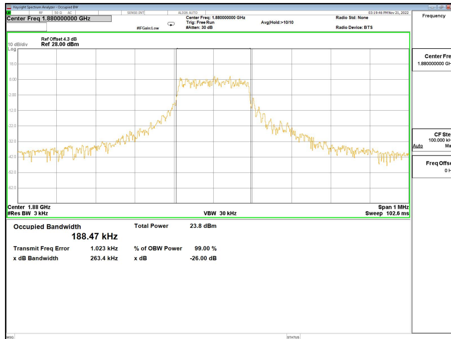
Band2-26dB/99% OBW-18900 Channel-QPSK-12@0-15K
