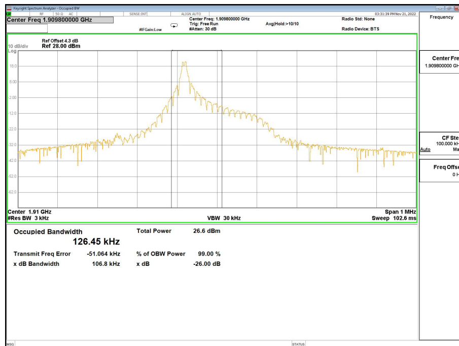
Band2-26dB/99% OBW-19198 Channel-BPSK-1@0-15K
