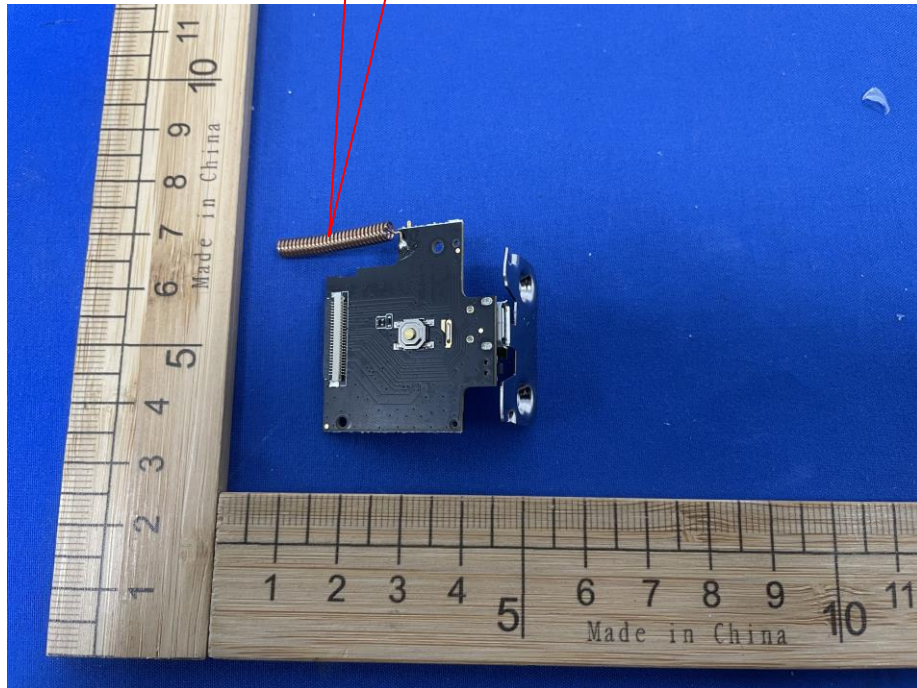
433 Antenna
