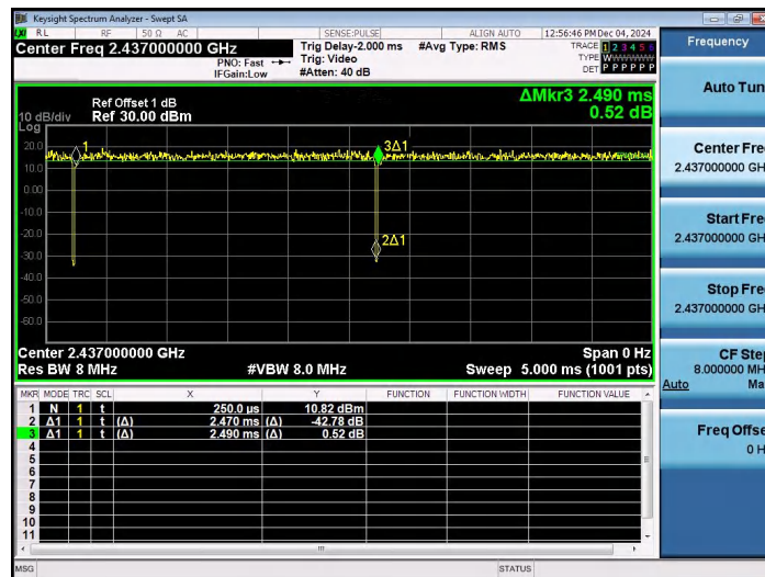
NTVN-11N40SISO-Ant1-2437
