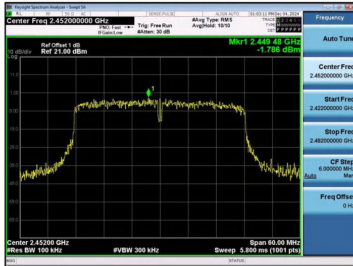
11N40SISO-Ant1-2452-0~Reference-PASS
