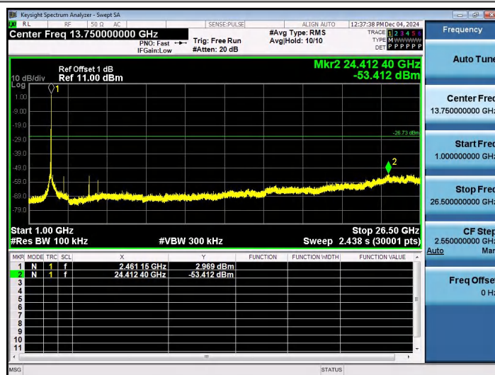
11B-Ant1-2462-1000~26500-PASS
