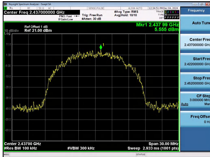
11B-Ant1-2437-0~Reference-PASS
