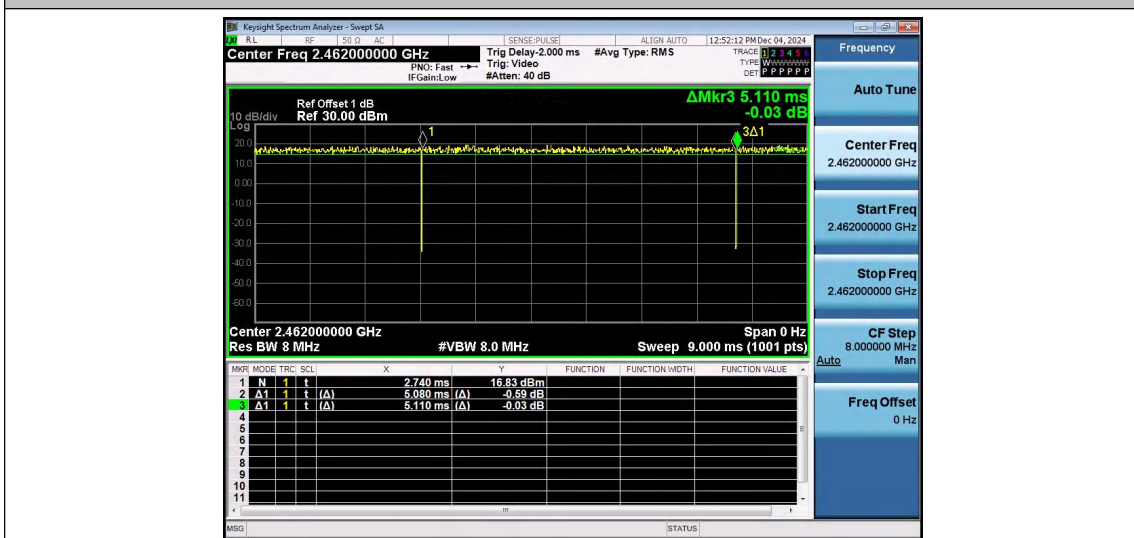
NTVN-11N20SISO-Ant1-2462
