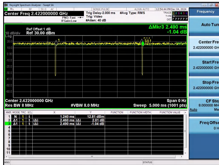
NTVN-11N40SISO-Ant1-2422
