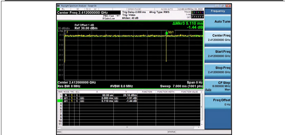
NTVN-11N20SISO-Ant1-2412
