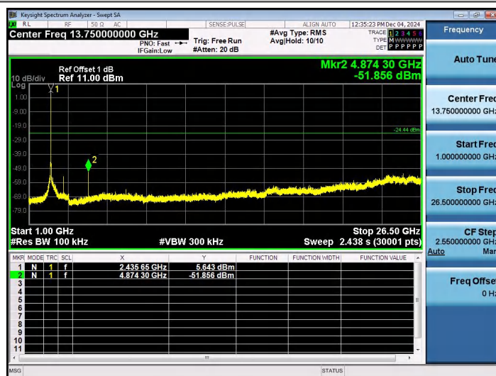
11B-Ant1-2437-1000~26500-PASS
