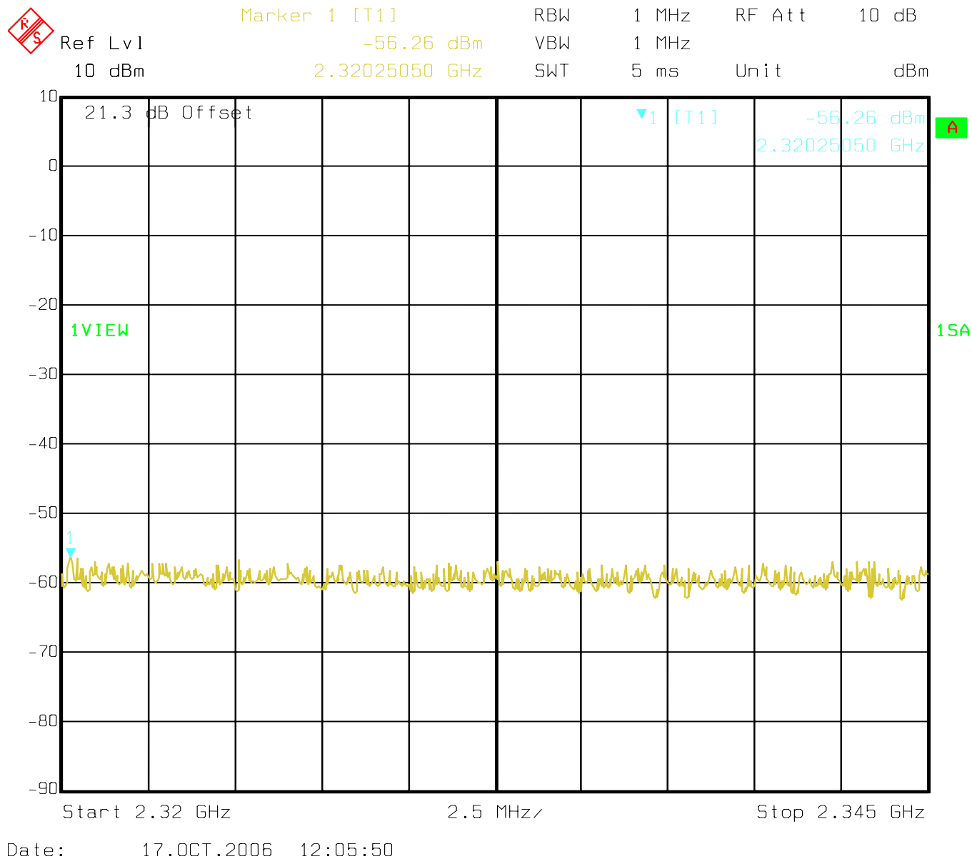
Plot 5 - Spurious emissions at the antenna terminals (2320 MHz to 2345 MHz, channel B, 2312.5 MHz)
