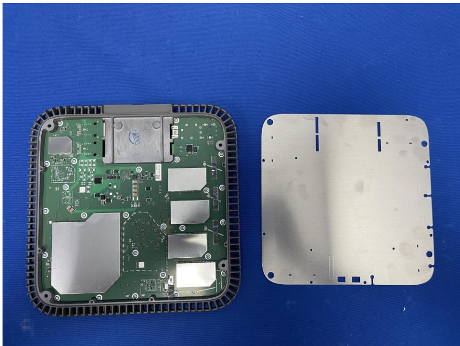
(2) EUT Photo (External Variant)
