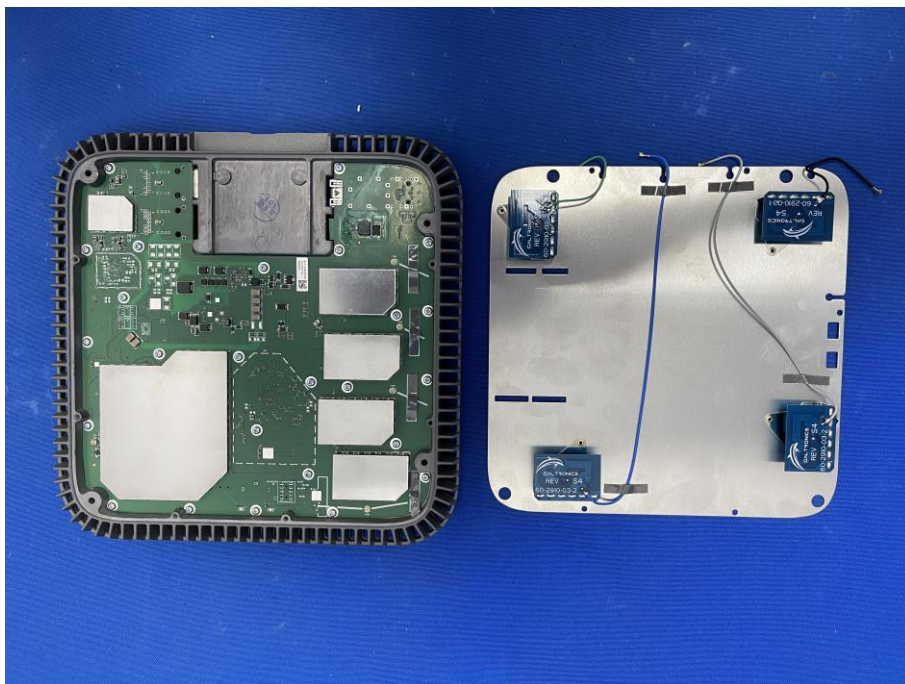
(6) EUT Photo (Internal Variant)
