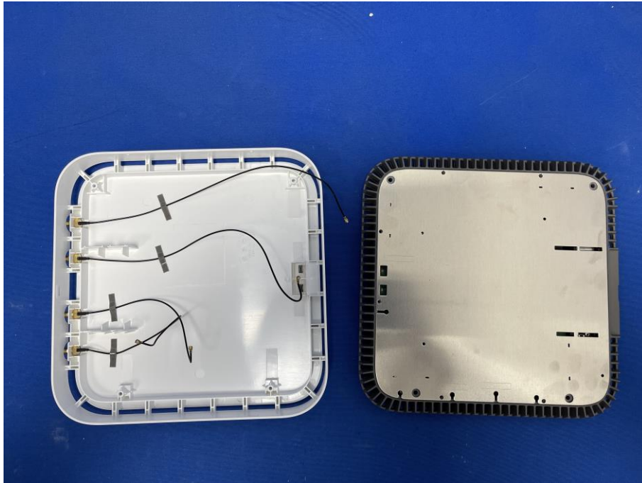
(1) EUT Photo (External Variant)
