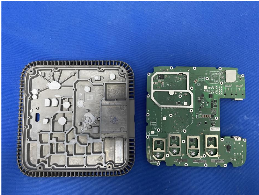
(7) EUT Photo (Internal Variant)
