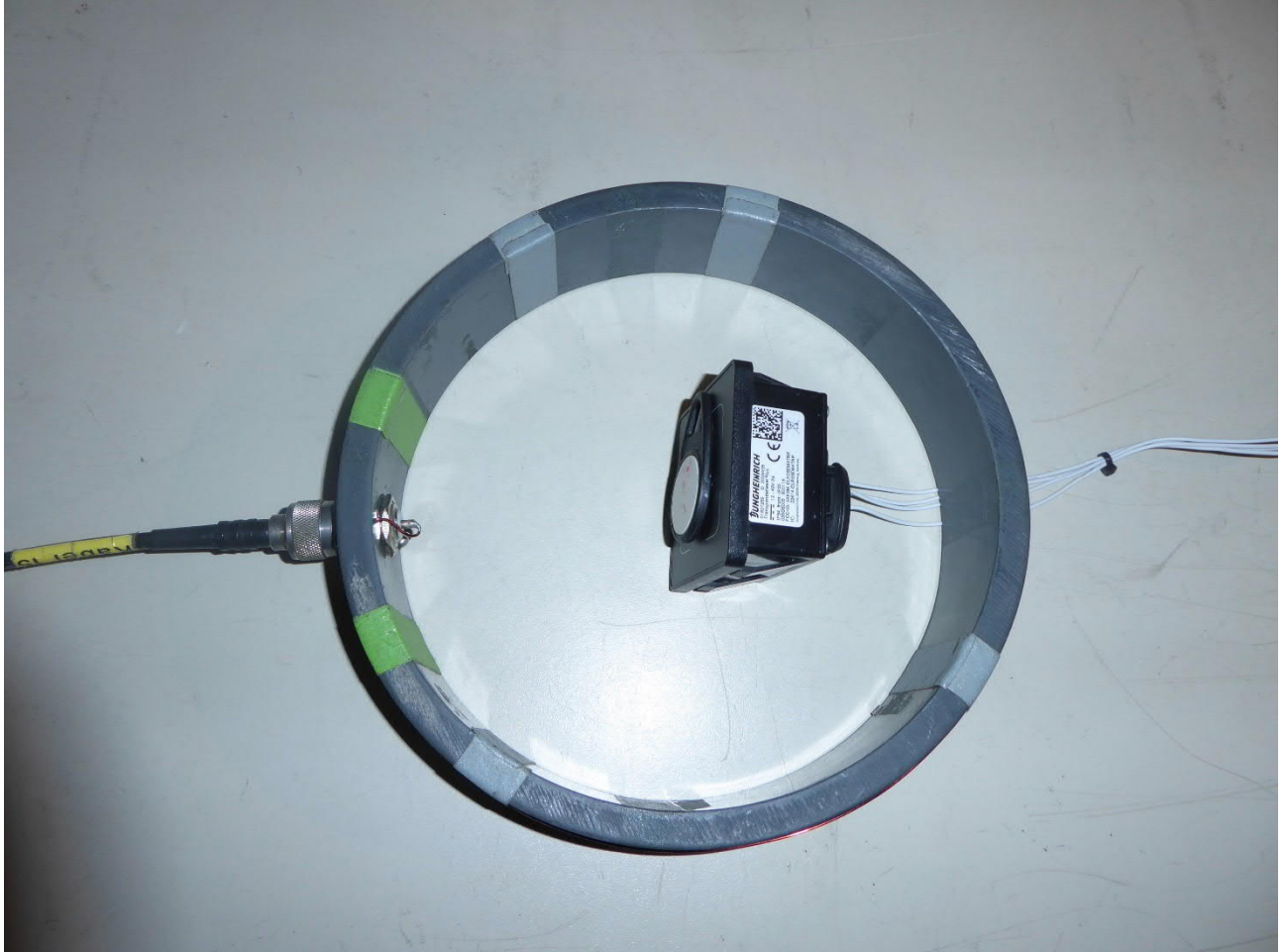
Test setup 99 % bandwidth
