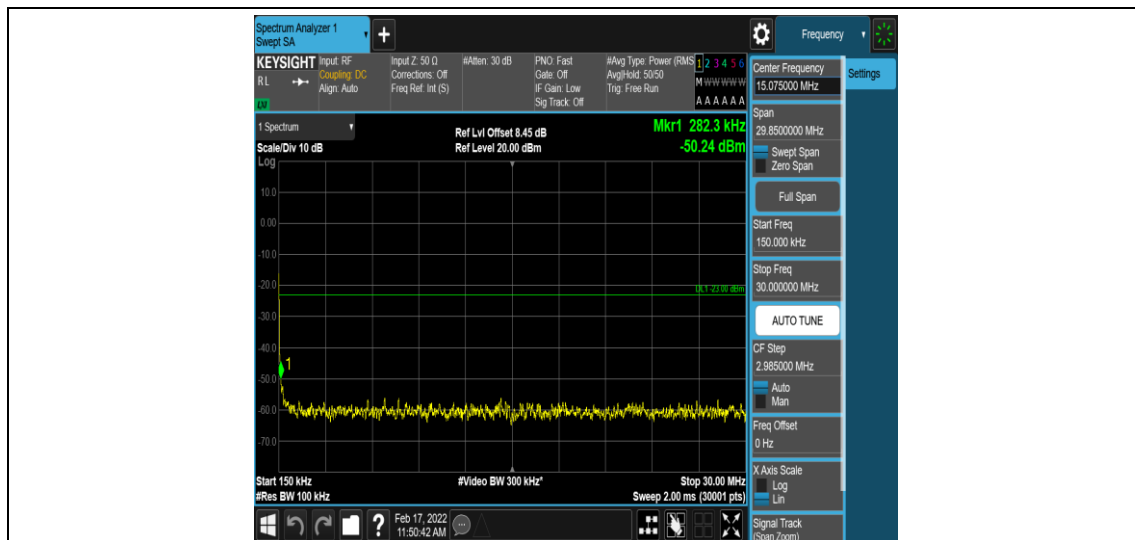
Band26-1.4MHz-QPSK-26915-1-0-Low-0.15-30--50.24-PASS
