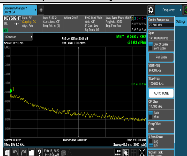
Band26-1.4MHz-16QAM-26797-1-0-Low-0.009-0.15--51.63-PASS
