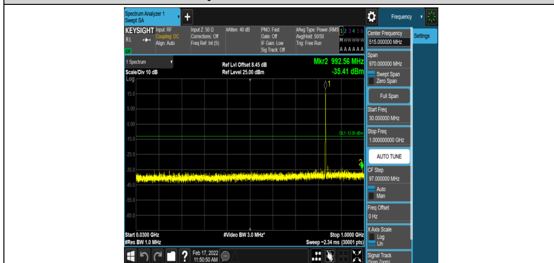
Band26-1.4MHz-QPSK-26915-1-0-Low-30-1000--35.41-PASS
