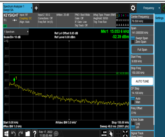
Band26-1.4MHz-16QAM-27033-1-0-High-0.009-0.15--52.39-PASS
