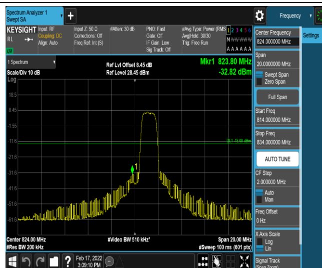
Band26-10MHz-16QAM-26840-6-0-Low--32.82-PASS
