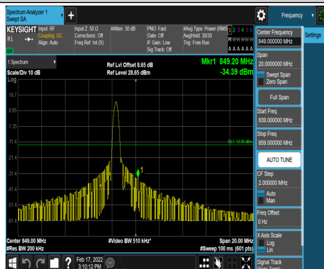
Band26-10MHz-16QAM-26990-1-0-High--34.39-PASS
