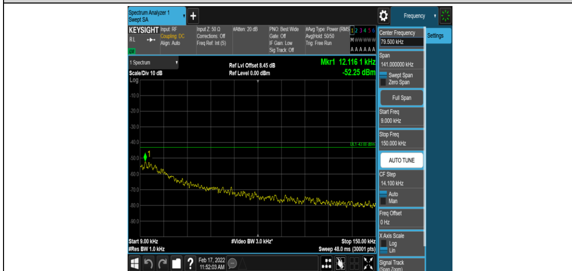
Band26-1.4MHz-16QAM-26915-1-0-Low-0.009-0.15--52.25-PASS
