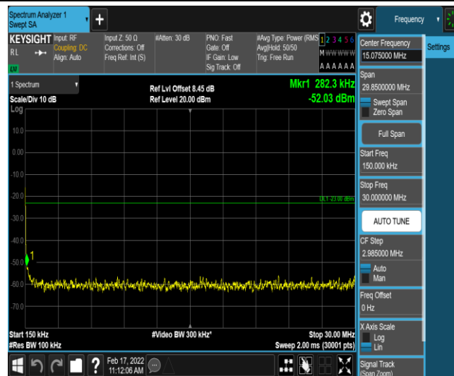
Band26-1.4MHz-QPSK-26797-1-0-Low-0.15-30--52.03-PASS
