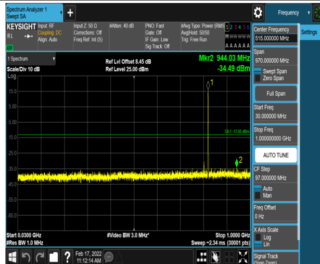
Band26-1.4MHz-QPSK-26797-1-0-Low-30-1000--34.49-PASS
