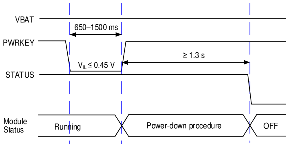
Figure 8: Power-down Timing
