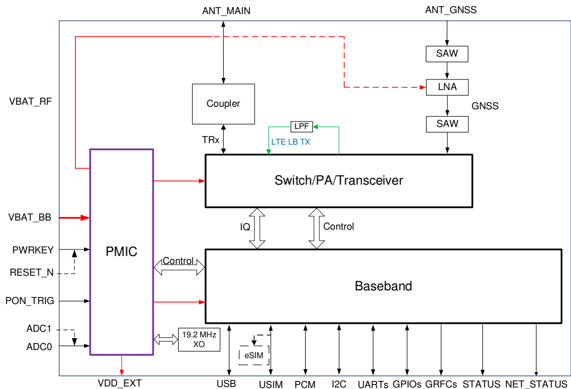
Figure 1: Functional Diagram of UBM1-GL
