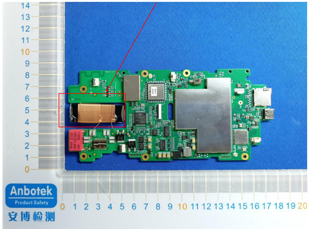
125KHz Antenna
