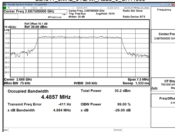
Band41_5MHz_64QAM_RB25_0_CH41565
