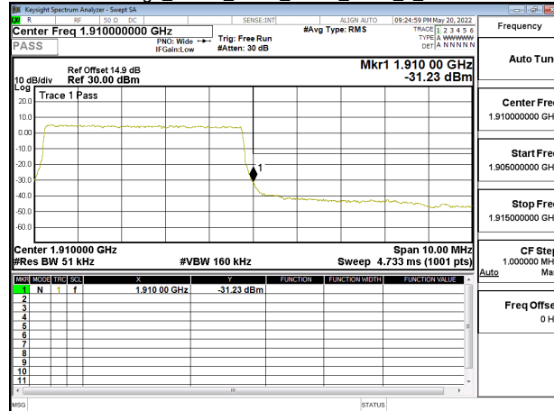
Band Edge_Band2_5MHz_QPSK_RB25_0_CH19175
