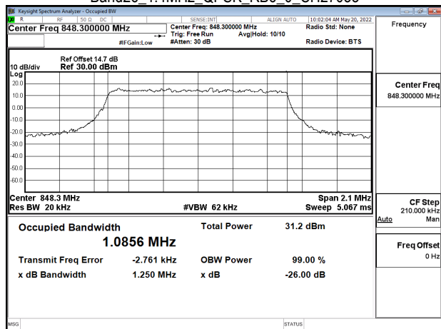
Band26_1.4MHz_QPSK_RB6_0_CH27033
