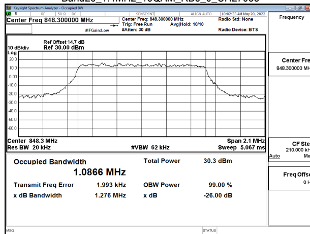
Band26_1.4MHz_16QAM_RB6_0_CH27033
