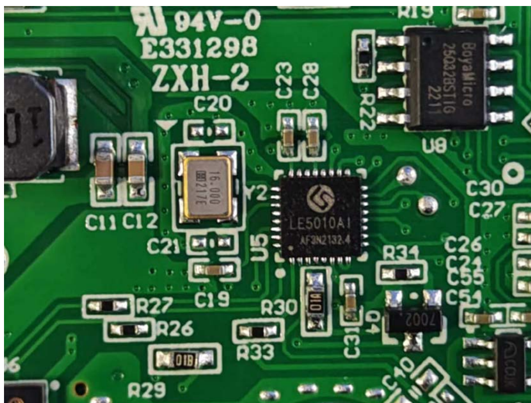
FIGURE 6 LED STRIP (M/N: CSTN16CDID) CHIP&CRYSTAL ON BOARD#1
