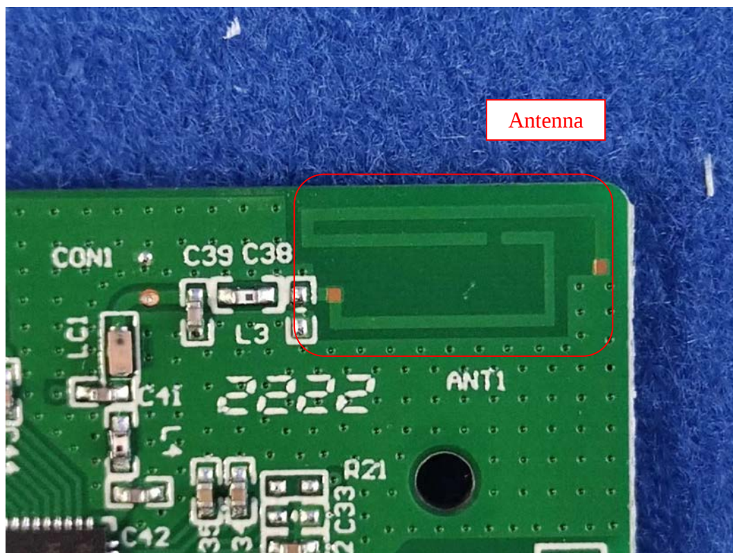
FIGURE 8 LED STRIP (M/N: CSTN16CDID) ANTENNA
