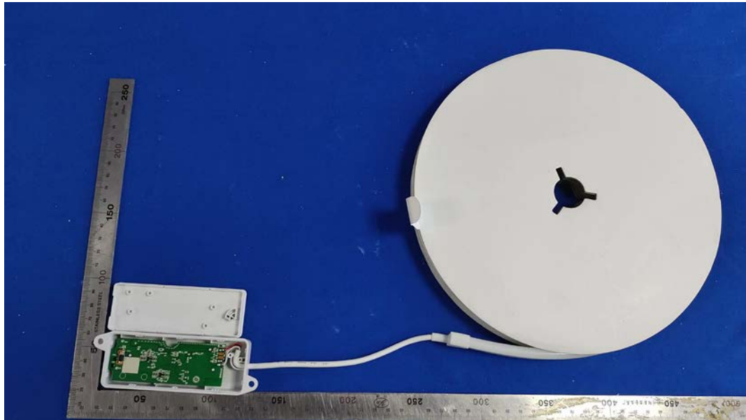
FIGURE 3 LED STRIP (M/N: CSTN16CDID) COVER REMOVED
