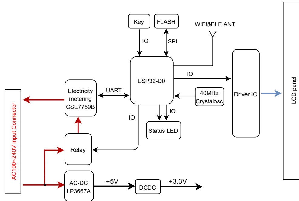
POWR320D Block Diagram
