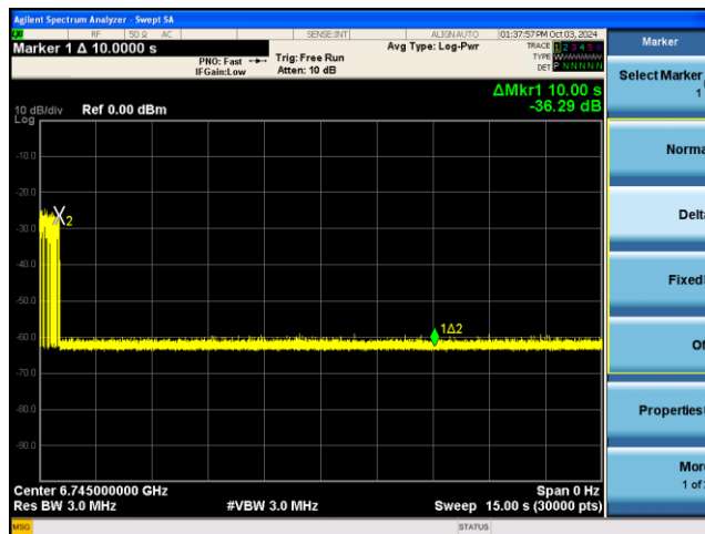
BE320-6745MHz -Inc2
