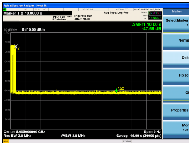
BE80-5985MHz-Inc2
