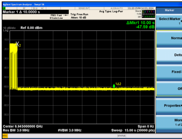
BE80-6945MHz-Inc1
