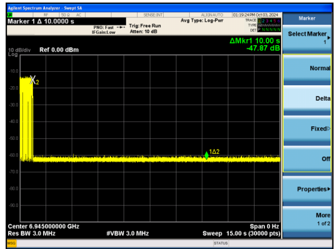
BE80-6945MHz -Inc2
