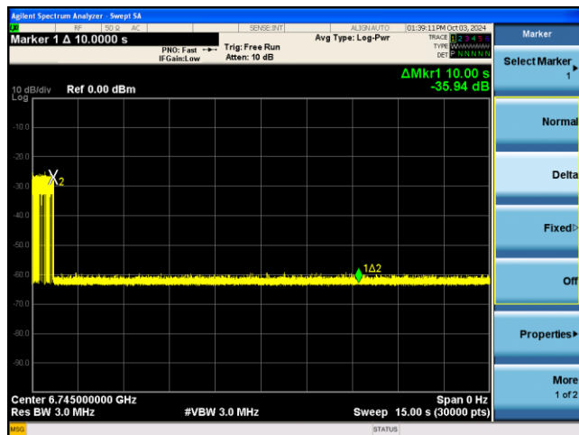
BE320-6745MHz-Inc1
