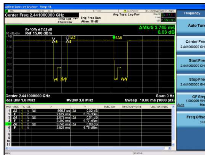
Bluetooth-GFSK
